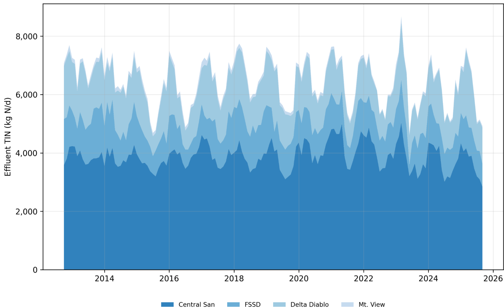
Figure C-4. TIN Load Contribution by Discharger to Suisun Bay
