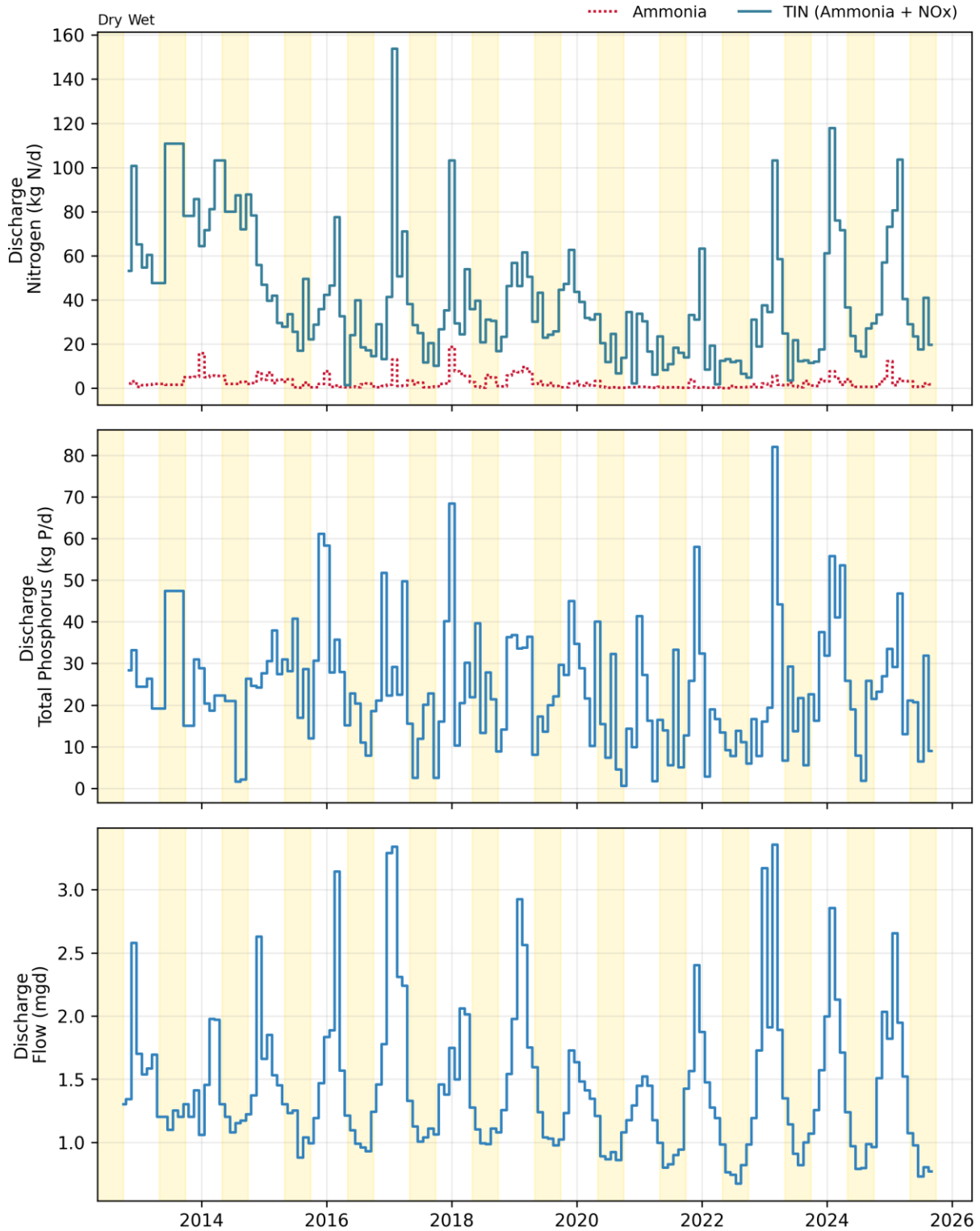
Figure 1-1. Discharge: American Canyon Monthly Flows and Loads
