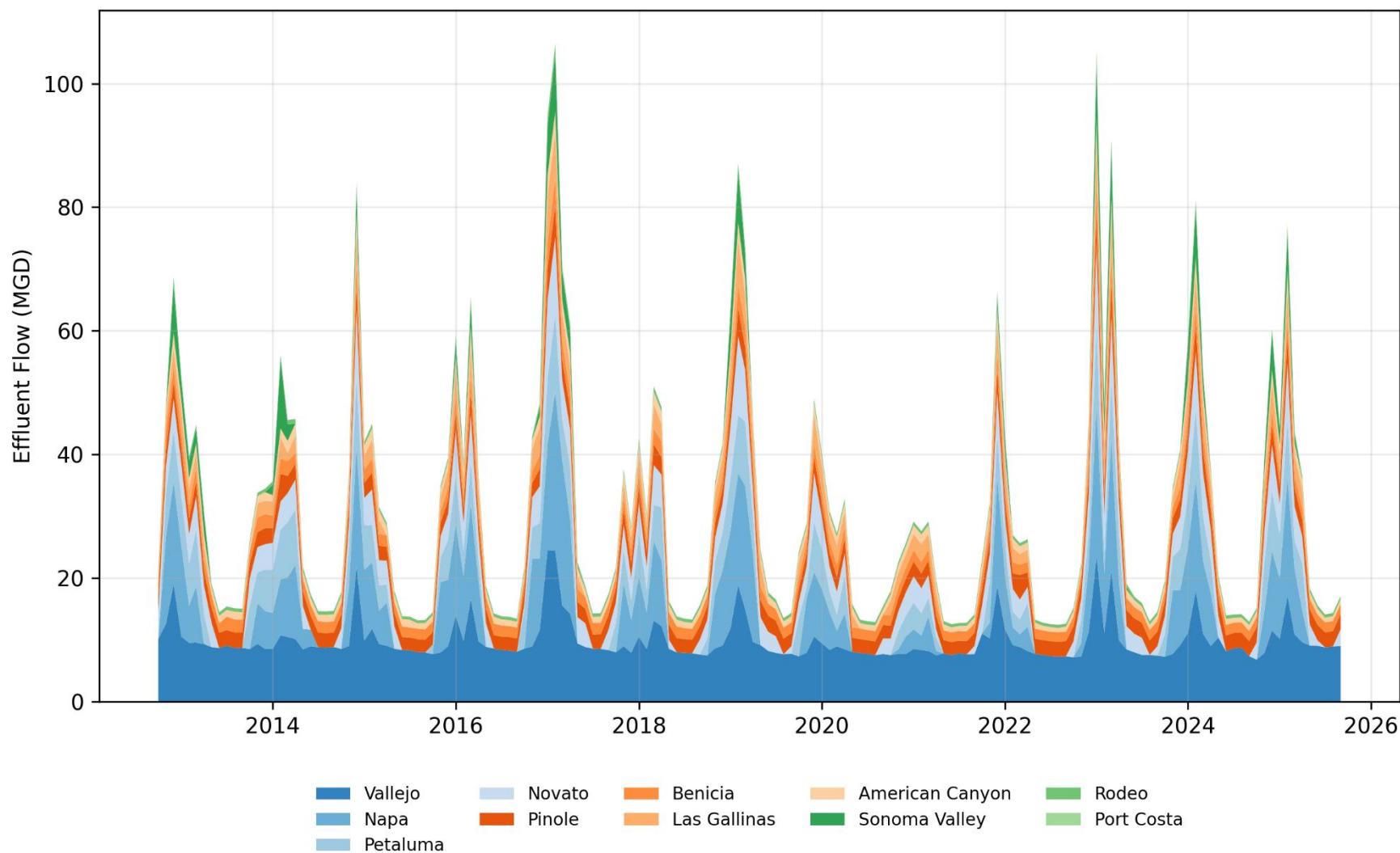
Figure C-6. Flow Contribution by Discharger to San Pablo Bay
