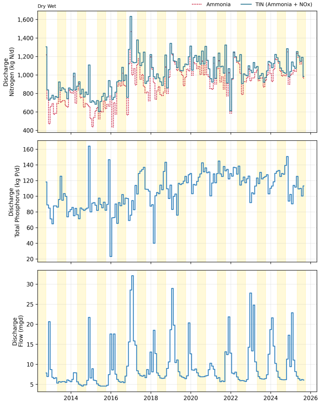
Figure 5-1. Discharge: CWSA Monthly Flows and Loads
