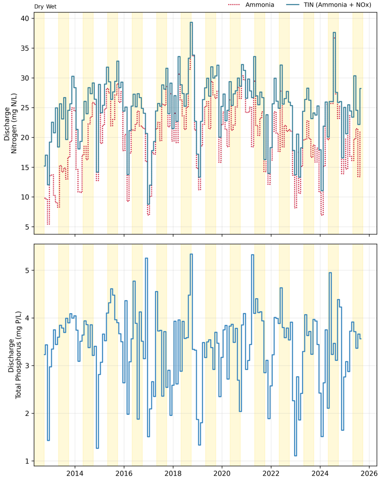
Figure 30-4. Discharge: Vallejo Monthly Concentrations
