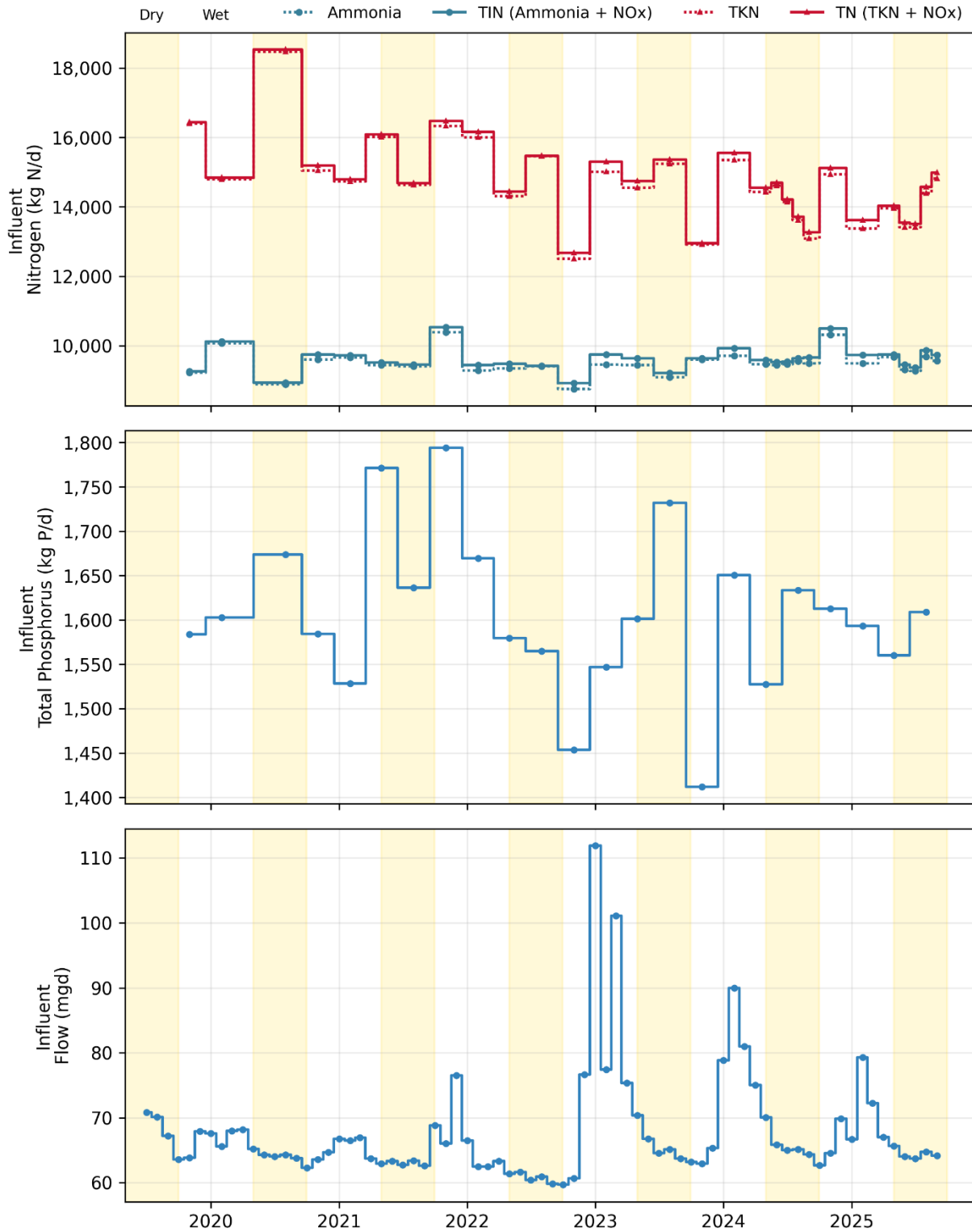
Figure 8-1. Influent: EBDA Monthly Flows and Loads (Values are only provided for months when all six agencies sampled; Loads are summed for all agencies.)
