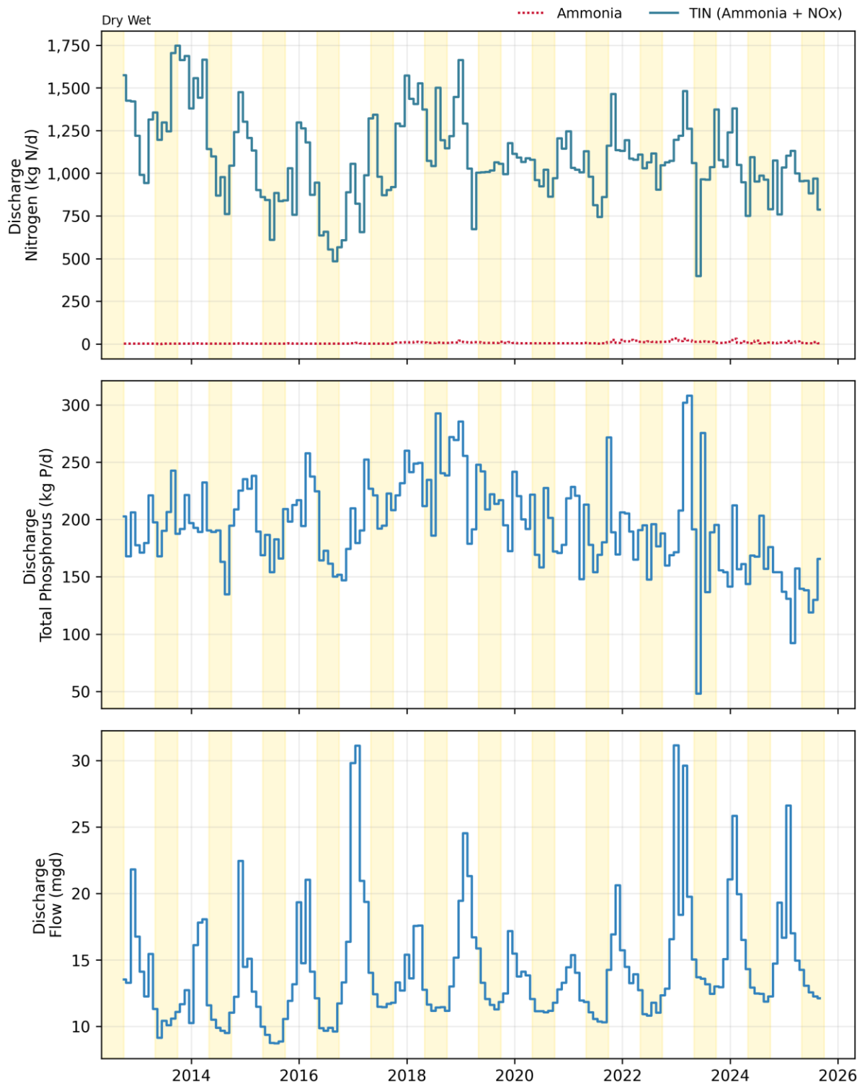
Figure 10-3. Discharge: FSSD Monthly Flows and Loads
