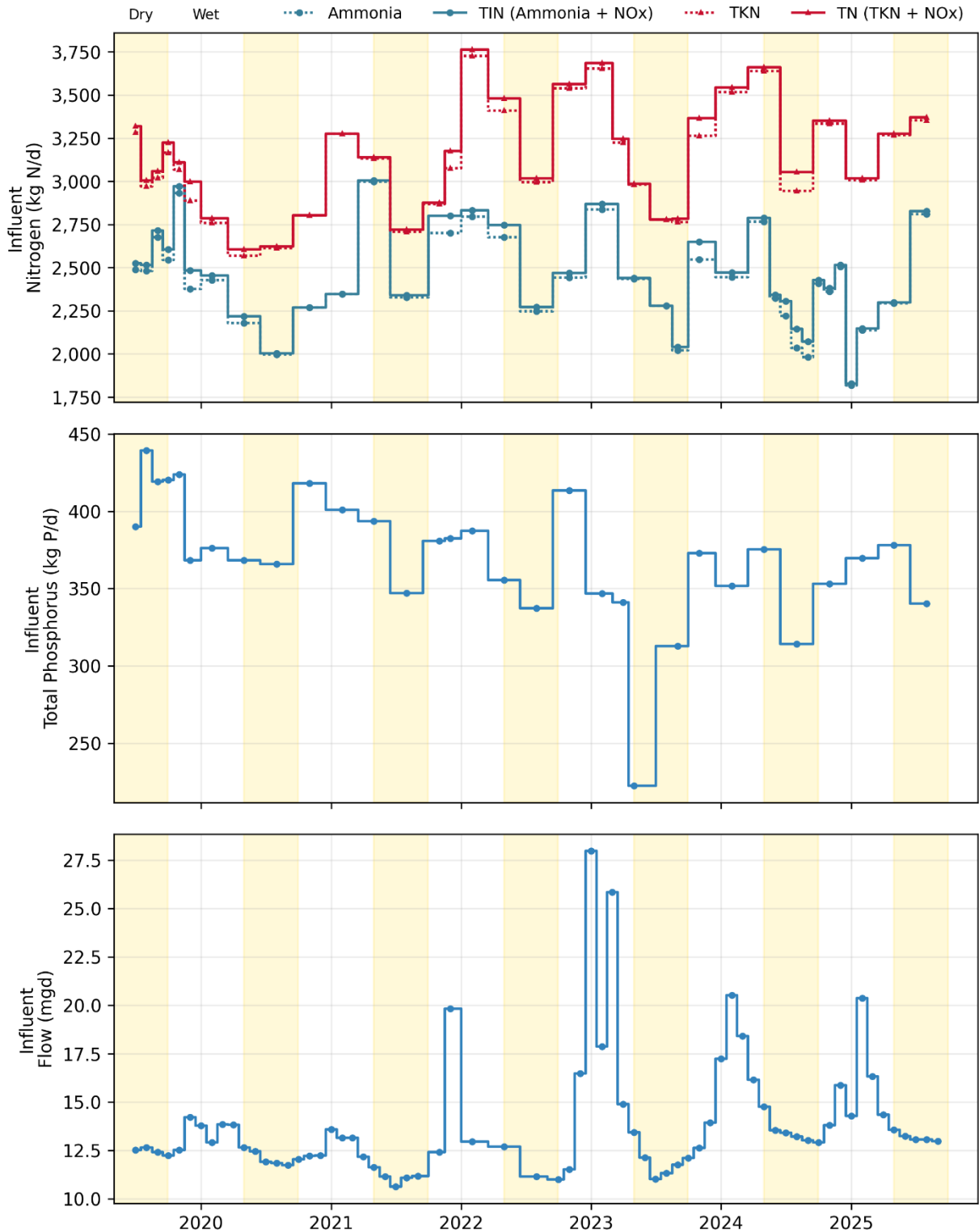
Figure 27-1. Influent: SVCW Monthly Flows and Loads
