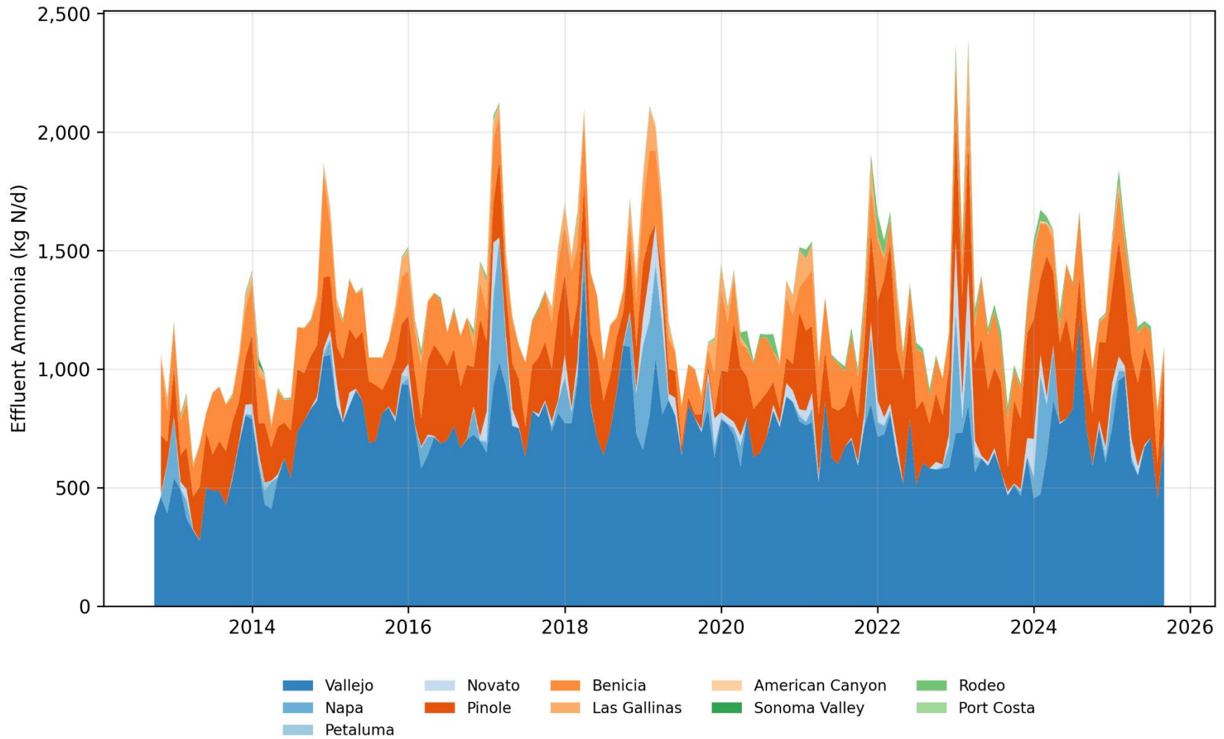
Figure C-7. Ammonia Load Contribution by Discharger to San Pablo Bay
