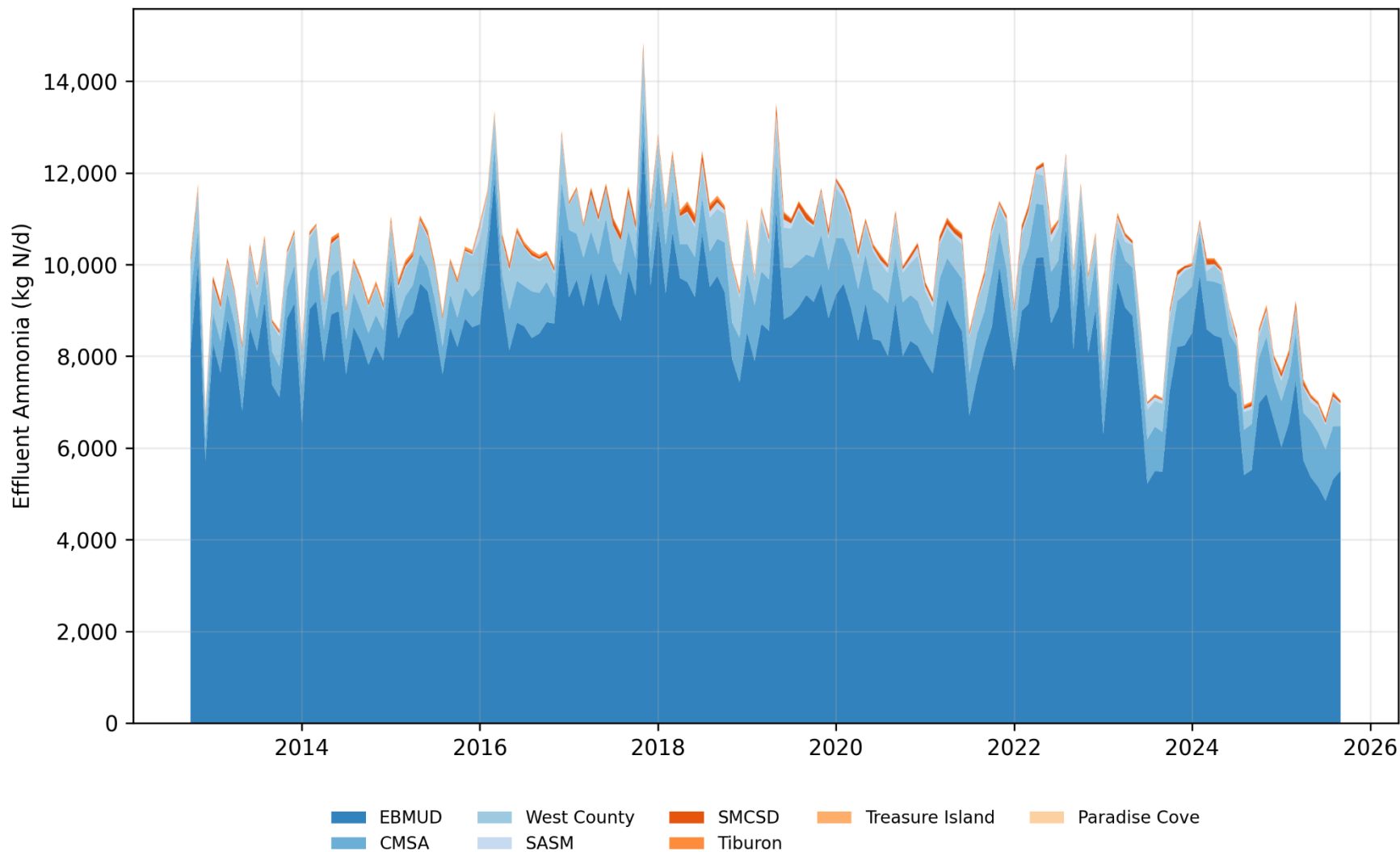
Figure C-12. Ammonia Load Contribution by Discharger to Central Bay
