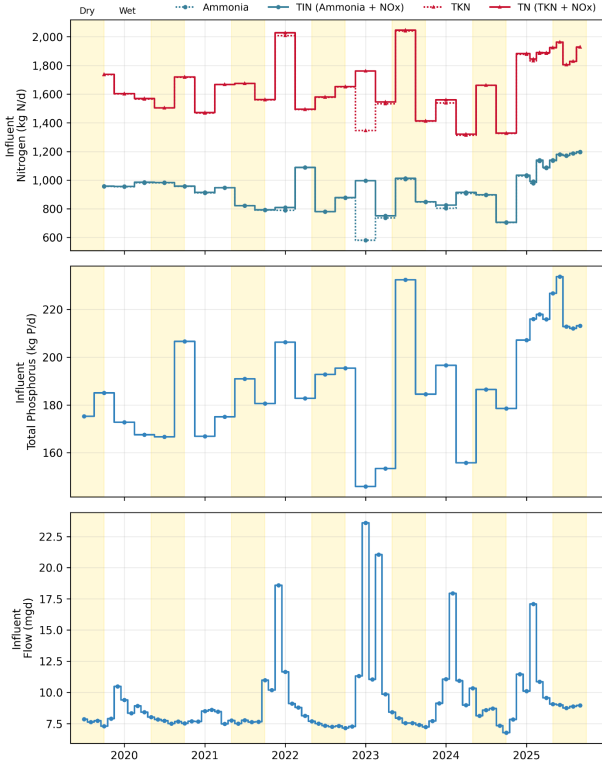
Figure 30-1. Influent: Vallejo Monthly Flows and Loads
