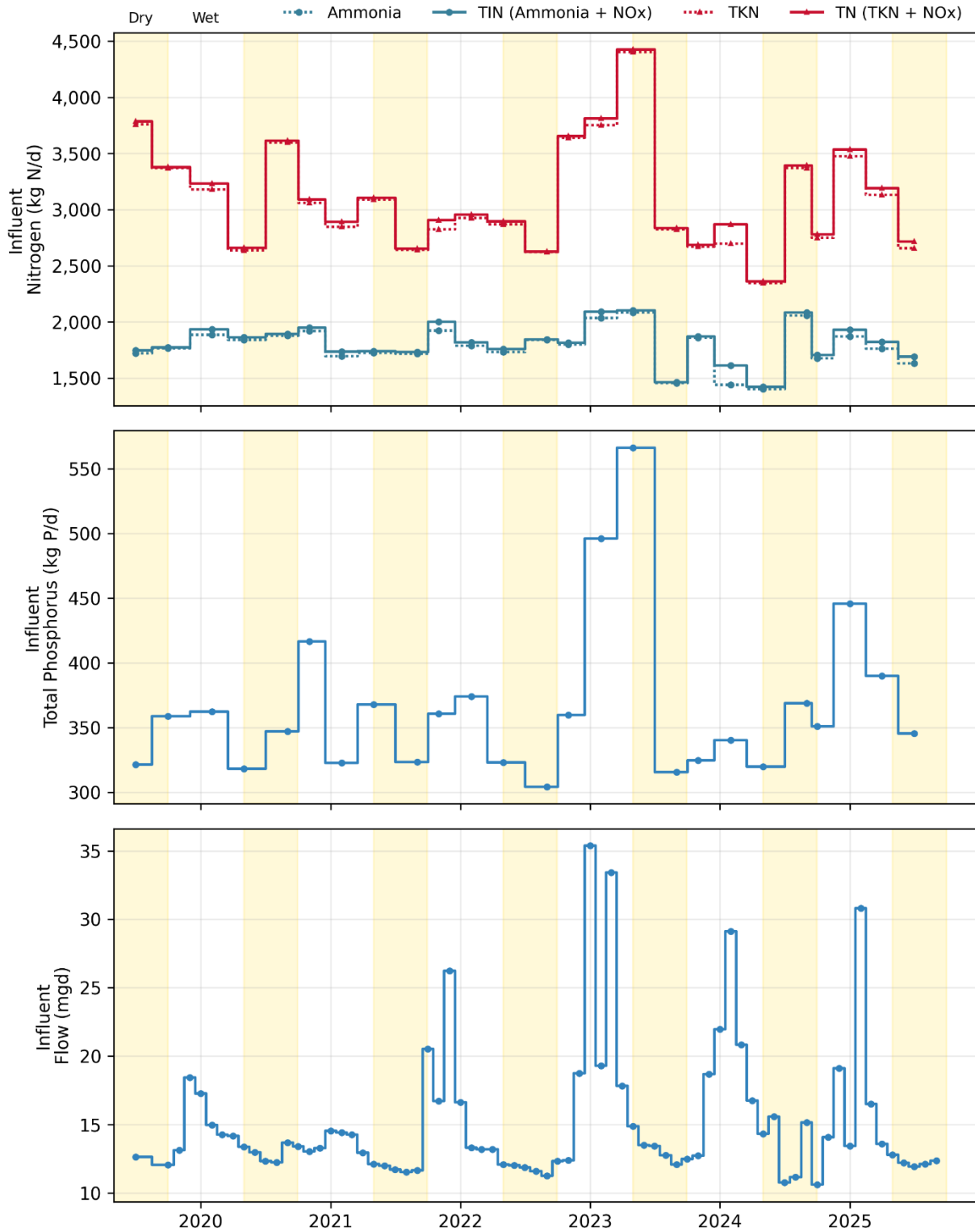
Figure 31-1. Influent: Monthly Flows and Loads for Both Treatment Plants
