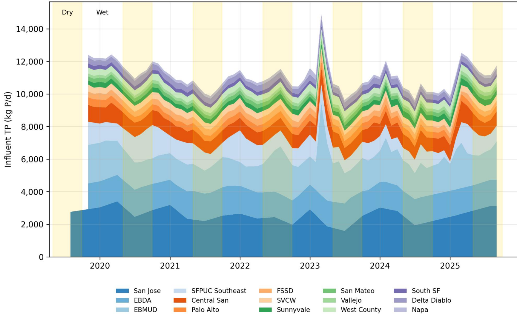
Figure A-7. Influent: Historical Average Quarterly TP Loads for Evaluation Period
