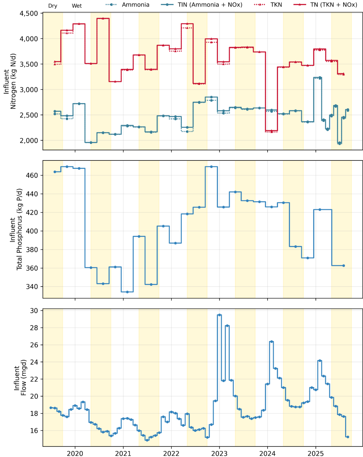
Figure 15-1. Influent: Palo Alto Monthly Flows and Loads
