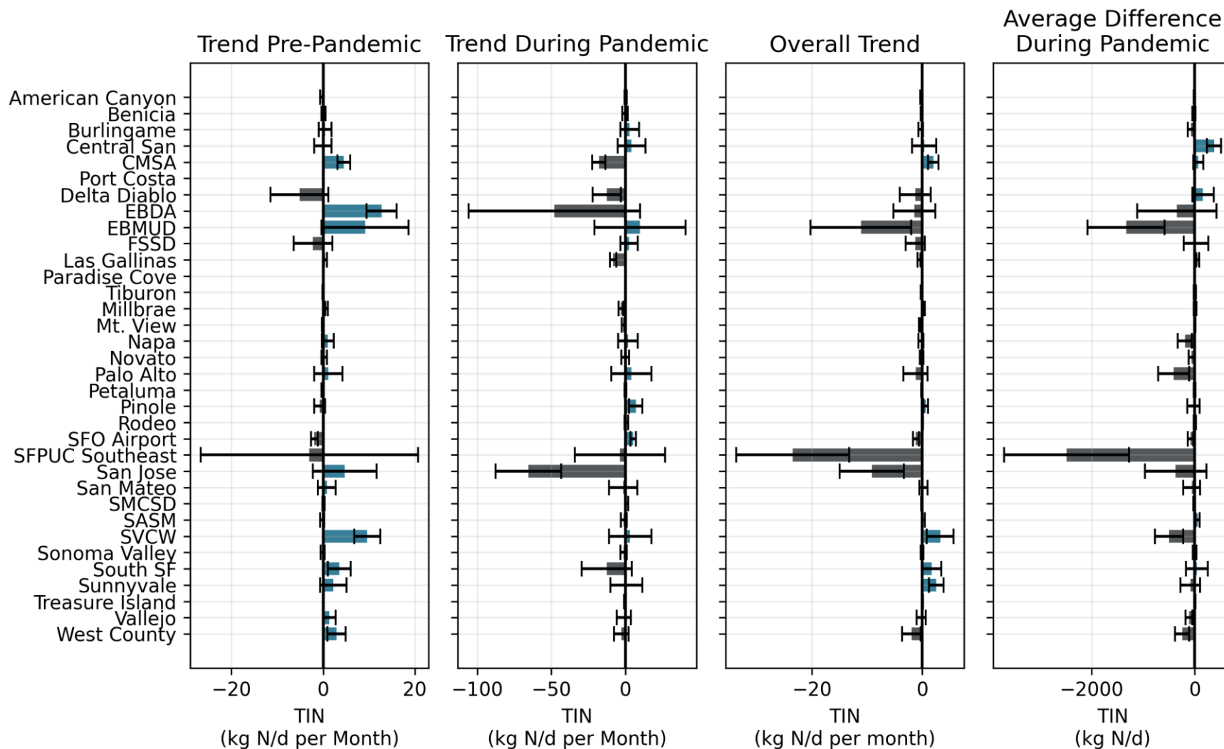
Figure B-8. Trend Coefficients for TIN (95% Confidence Interval Shown in Black)
