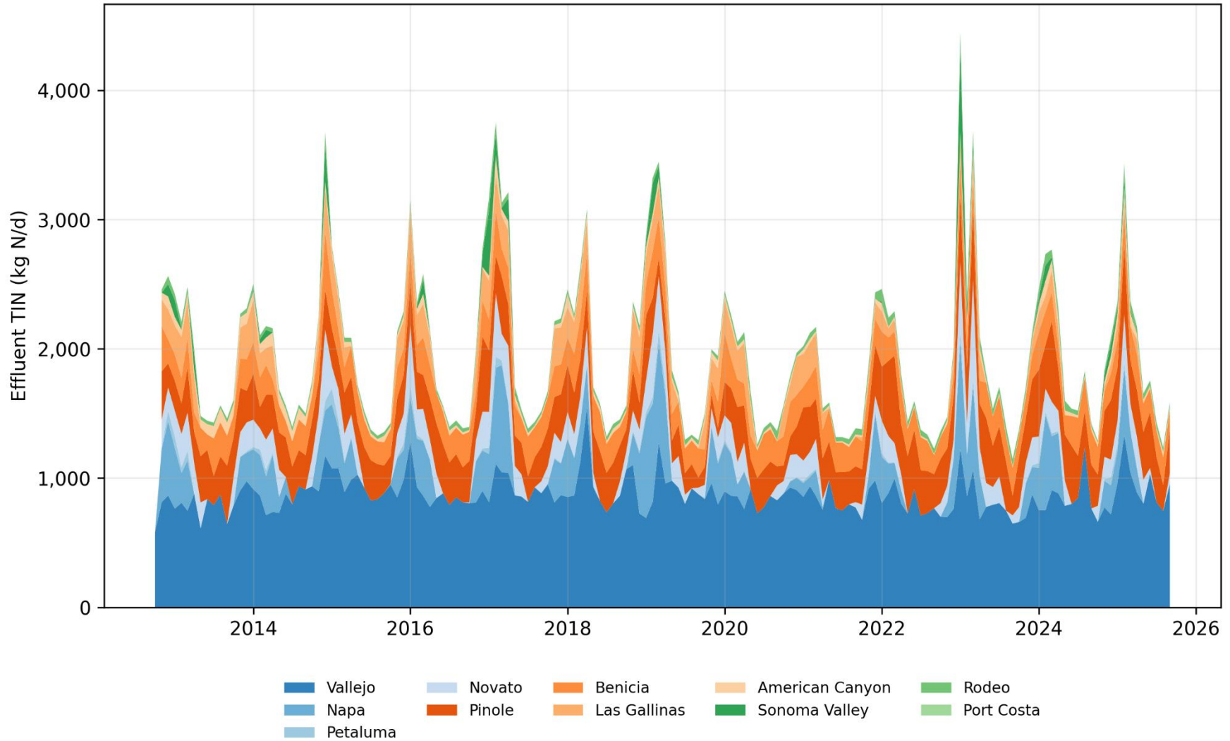
Figure C-9. TIN Load Contribution by Discharger to San Pablo Bay
