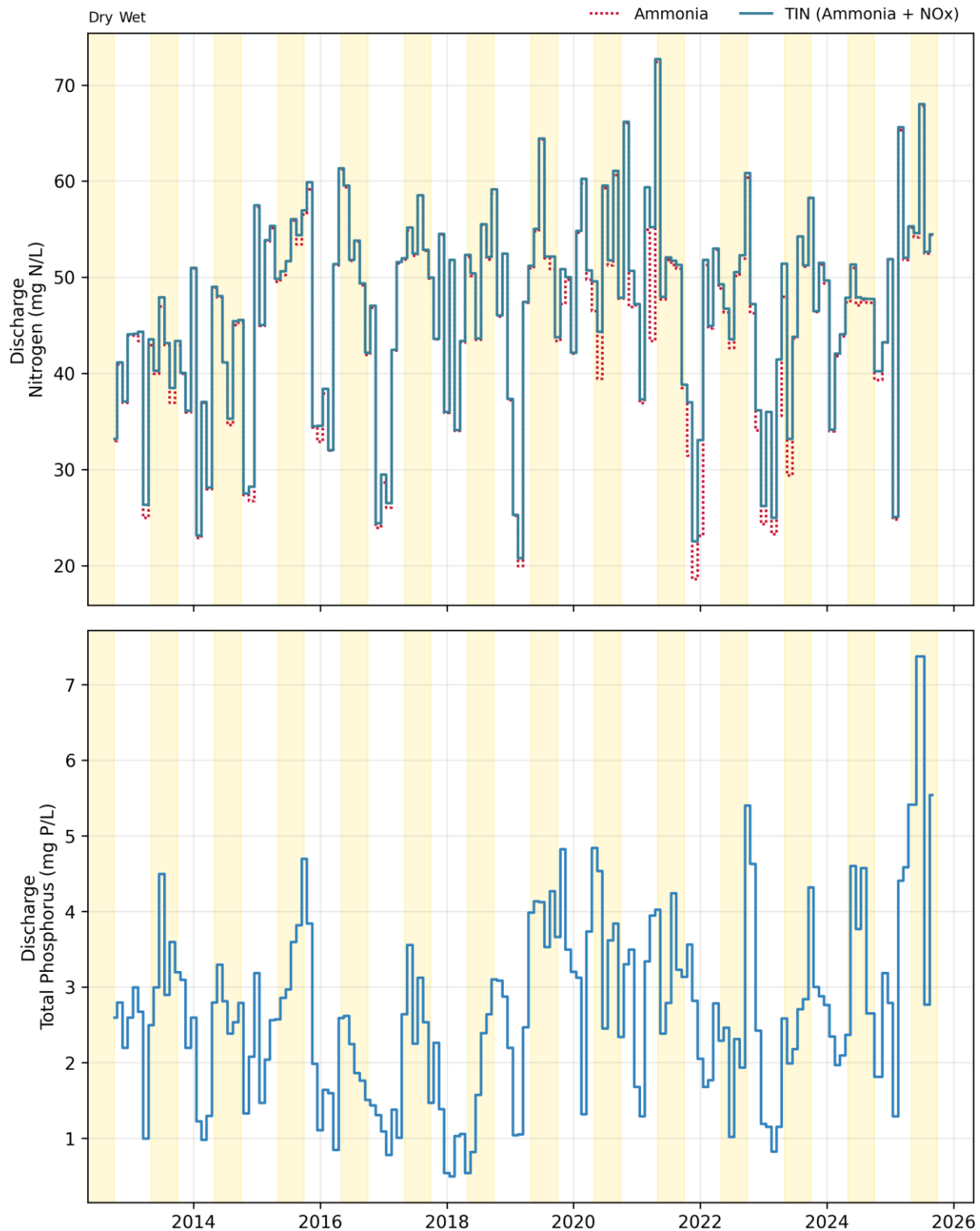
Figure 11-2. Discharge: Millbrae Monthly Concentrations
