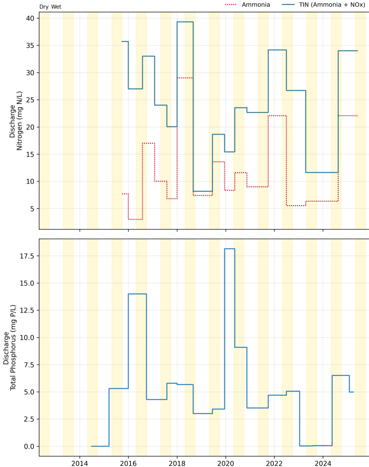
Figure 6-2. Discharge: Port Costa Monthly Concentrations
