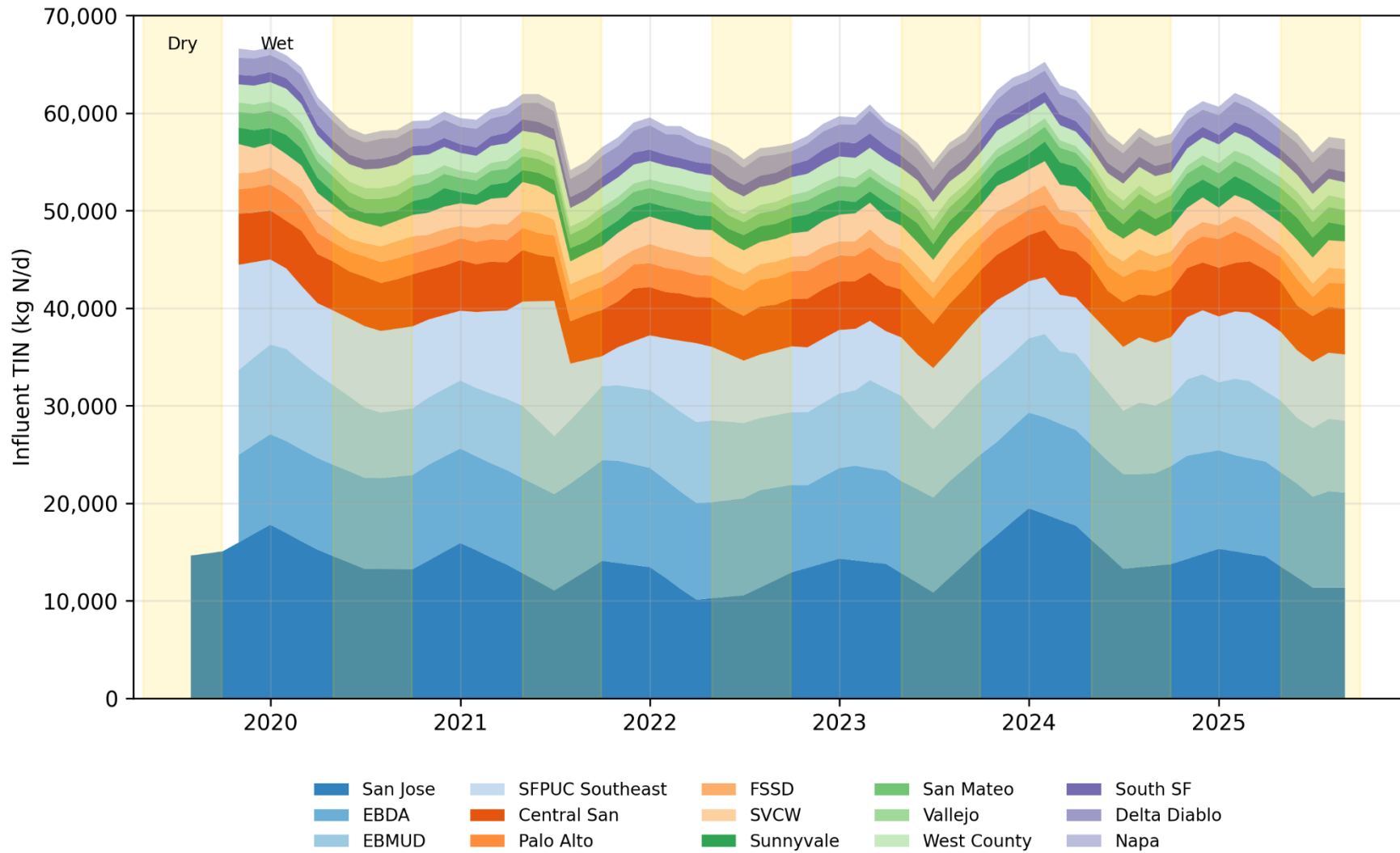
Figure A-4. Influent: Historical Average Quarterly TIN Loads
