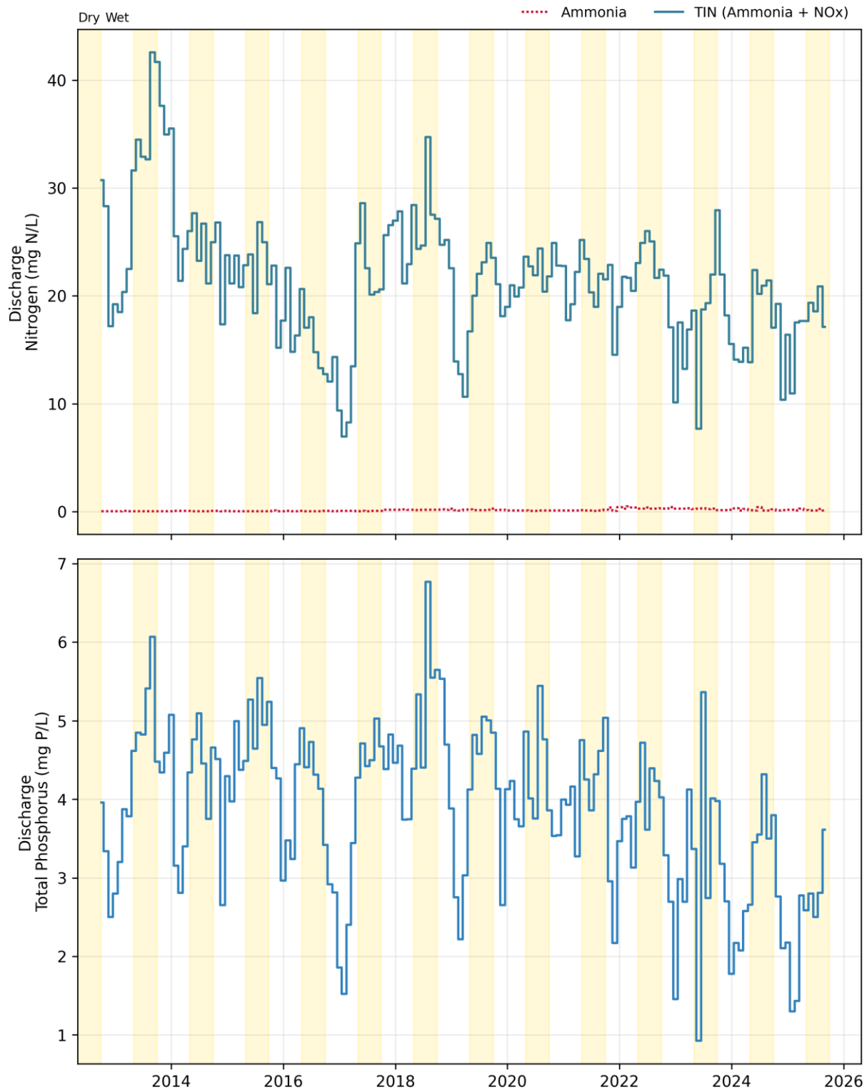
Figure 10-4. Discharge: FSSD Monthly Concentrations
