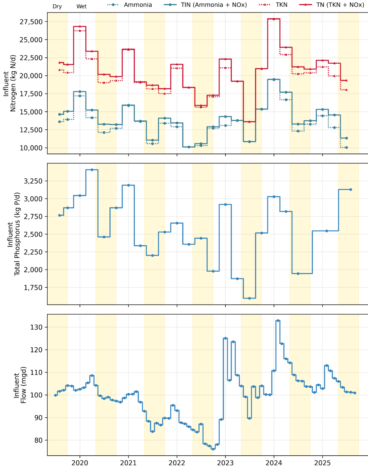
Figure 19-1. Influent: San Jose Monthly Flows and Loads
