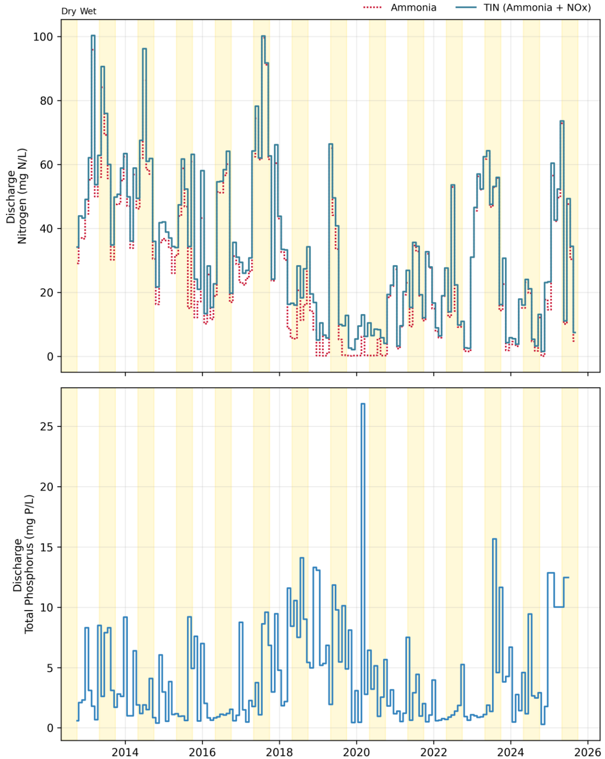
Figure 22-2. Discharge: SFO Airport Monthly Concentrations
