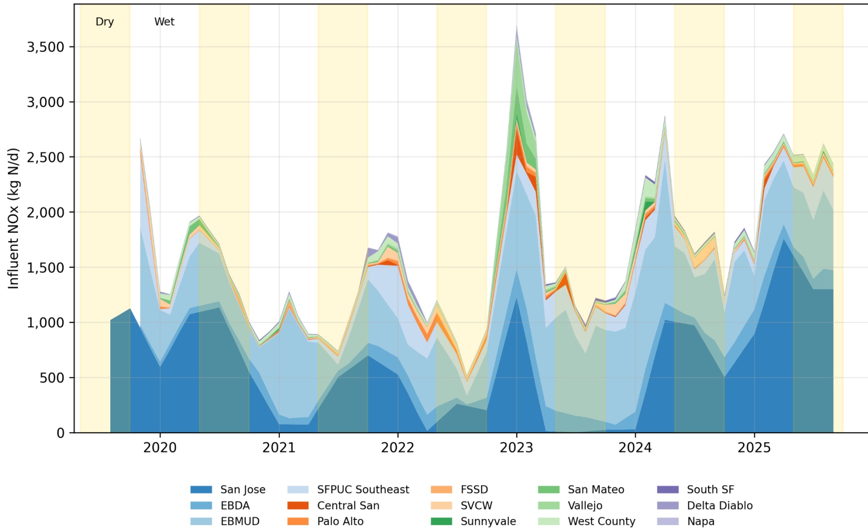
Figure A-3. Influent: Historical Average Quarterly NOx Loads
