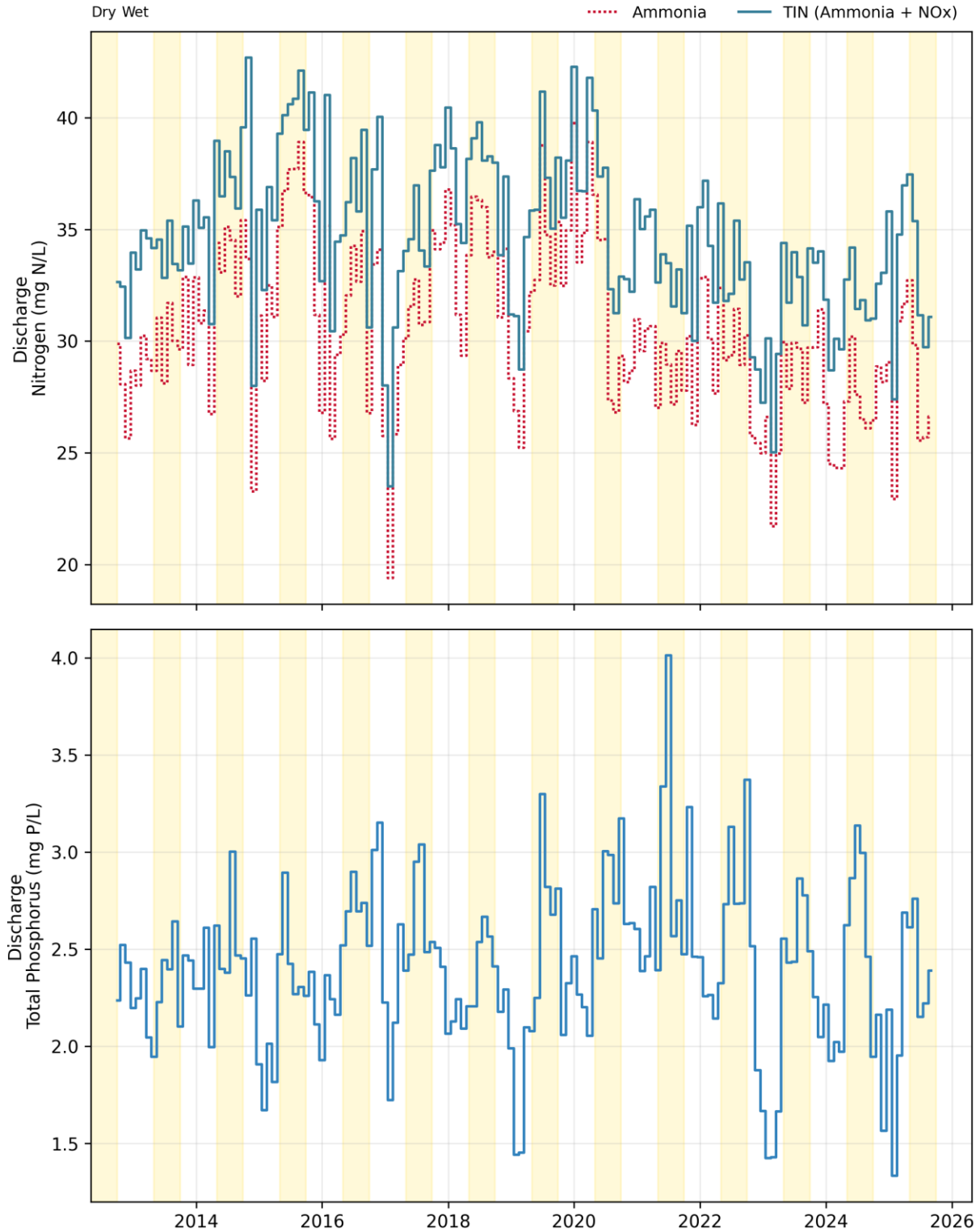
Figure 8-4. Discharge: EBDA Monthly Concentrations
