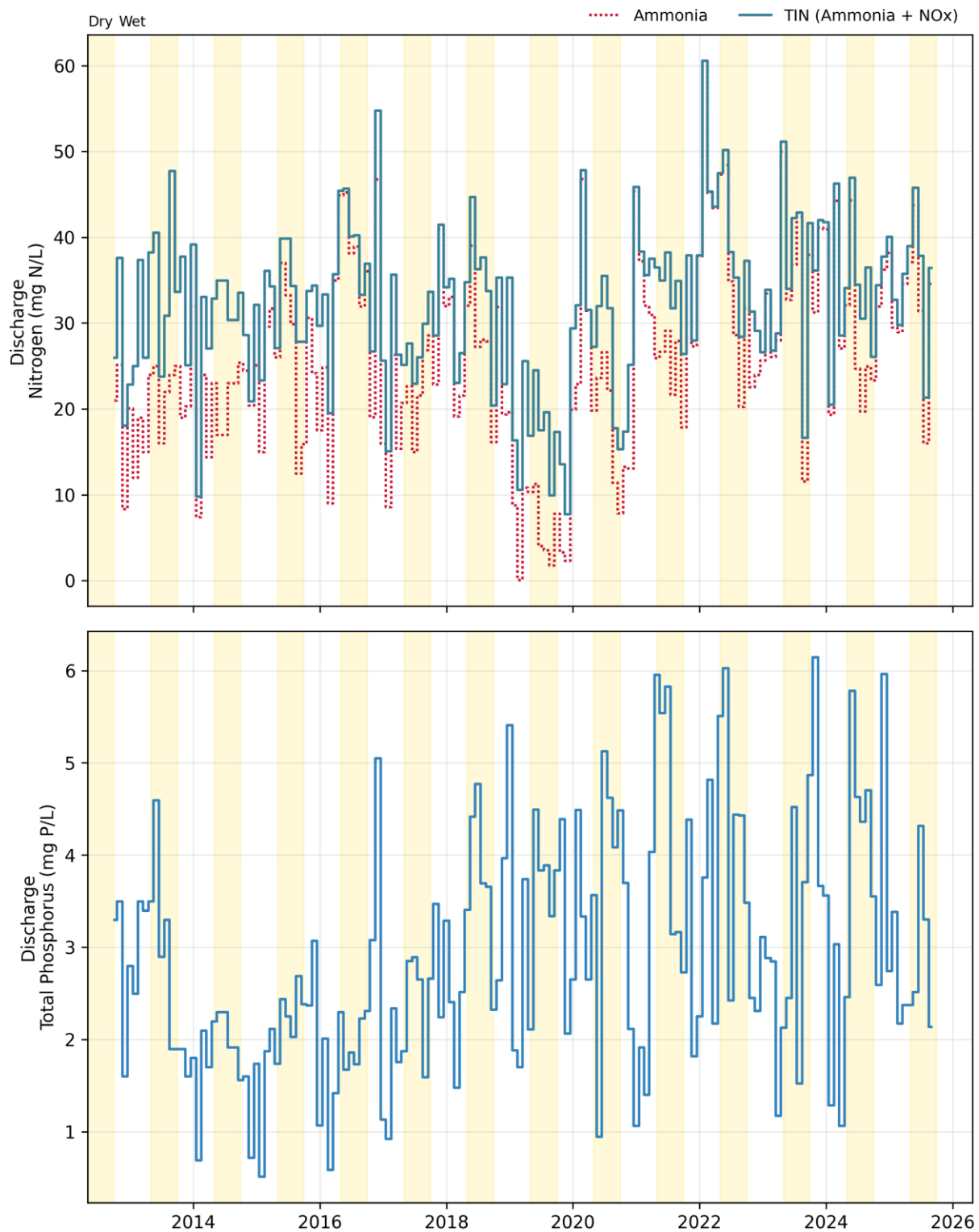
Figure 17-2. Discharge: Pinole Monthly Concentrations
