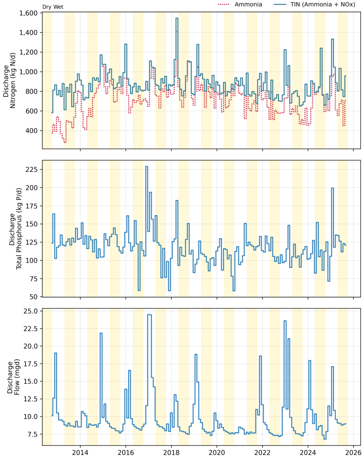
Figure 30-3. Discharge: Vallejo Monthly Flows and Loads
