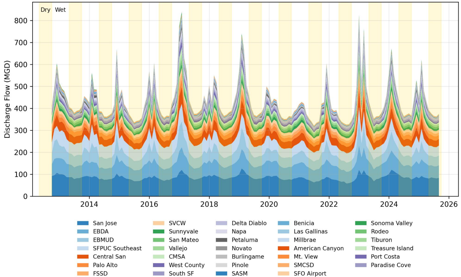
Figure B-1. Discharge: Average Monthly Discharge Flows
