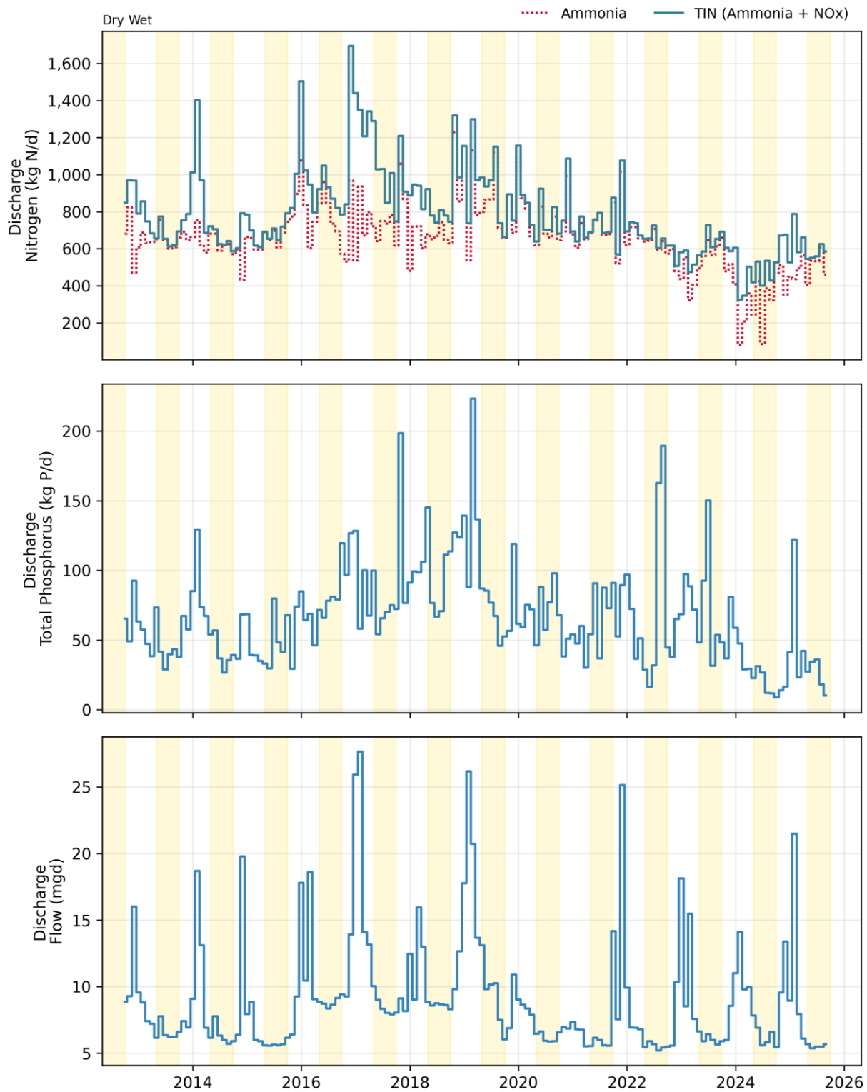
Figure 31-3. Discharge: Monthly Flows and Loads for Both Treatment Plants at the Common Outfall
