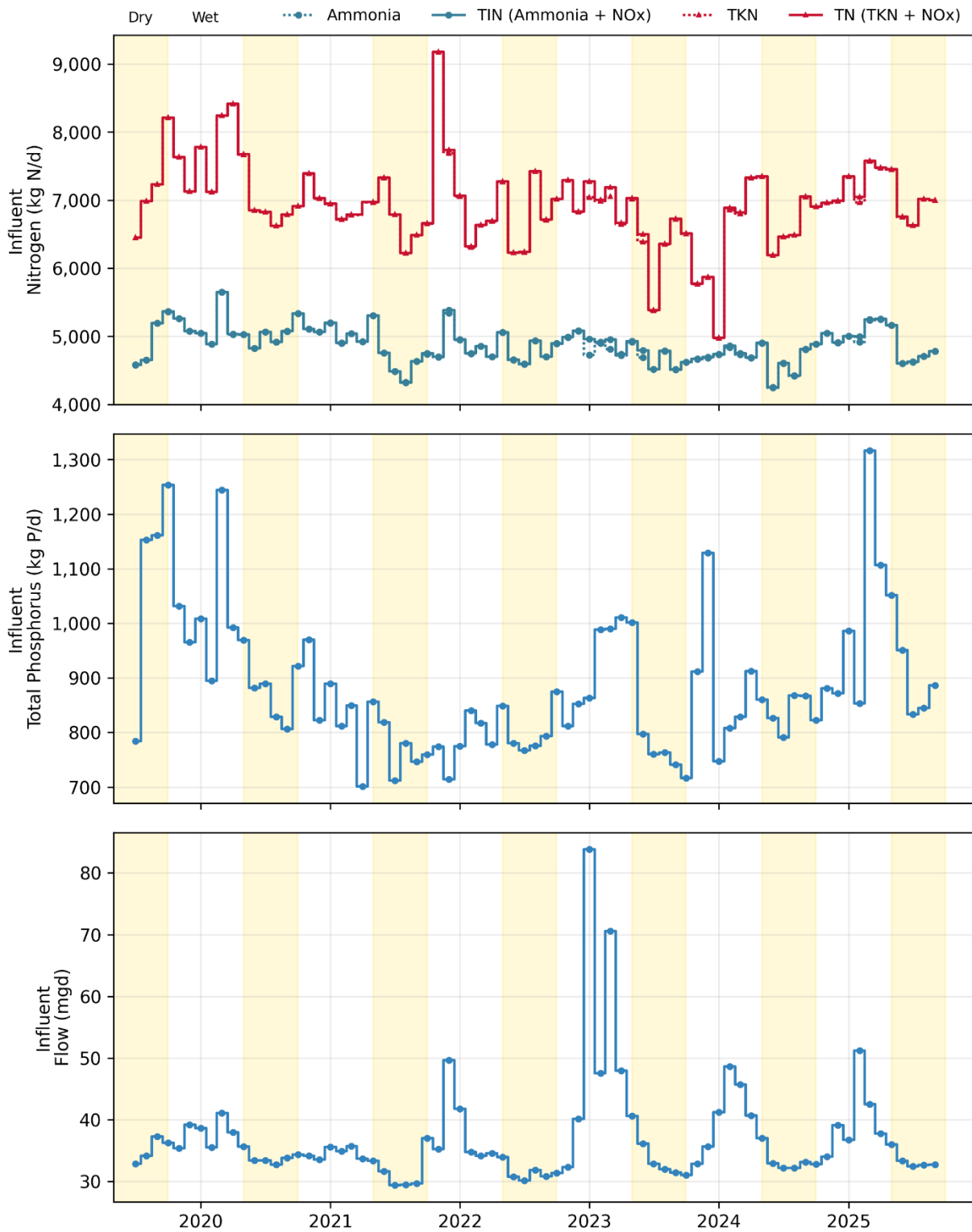
Figure 4-1. Influent: Central San Monthly Flows and Loads
