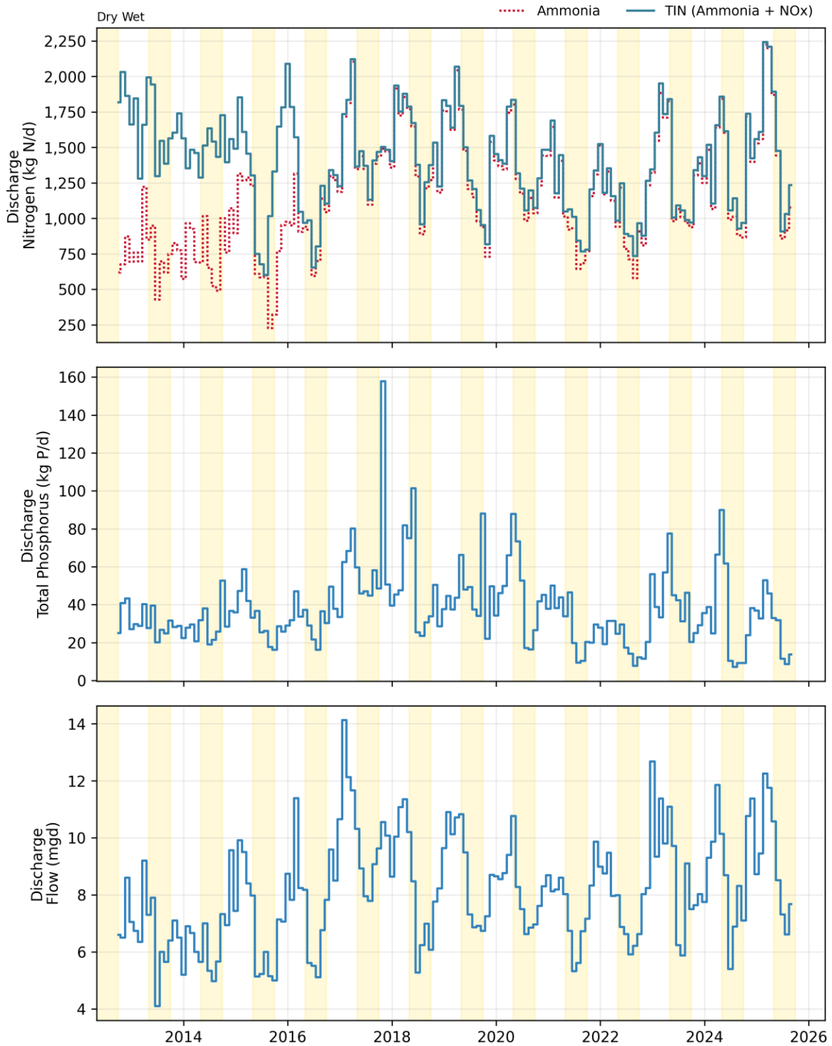
Figure 7-3. Discharge: Delta Diablo Monthly Flows and Loads
