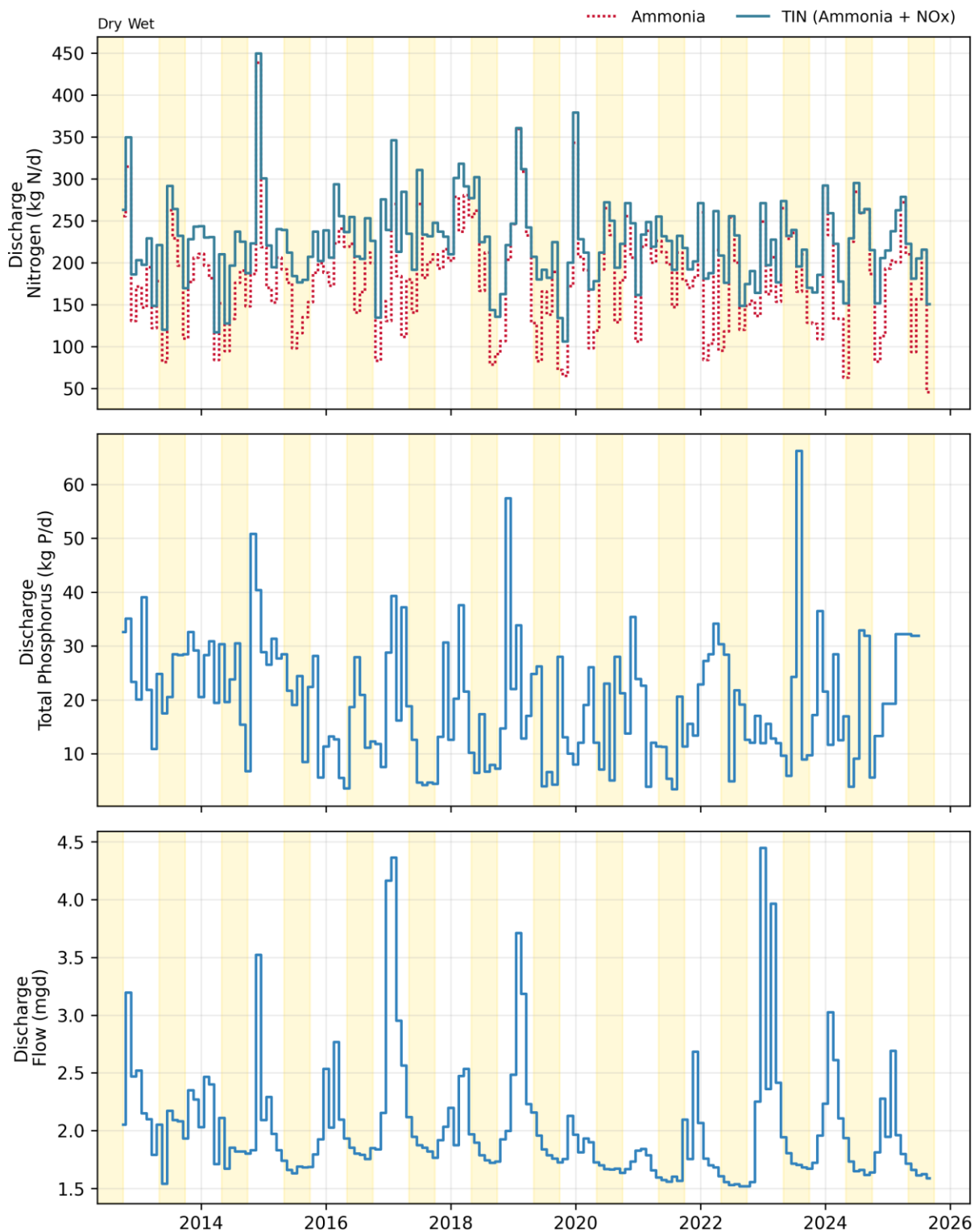
Figure 2-1. Discharge: Benicia Monthly Flows and Loads
