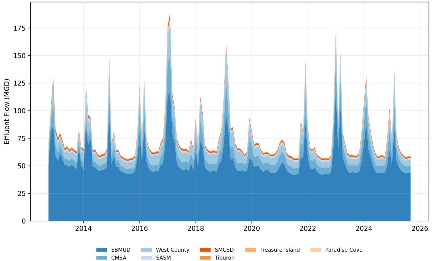
Figure C-11. Flow Contribution by Discharger to Central Bay
