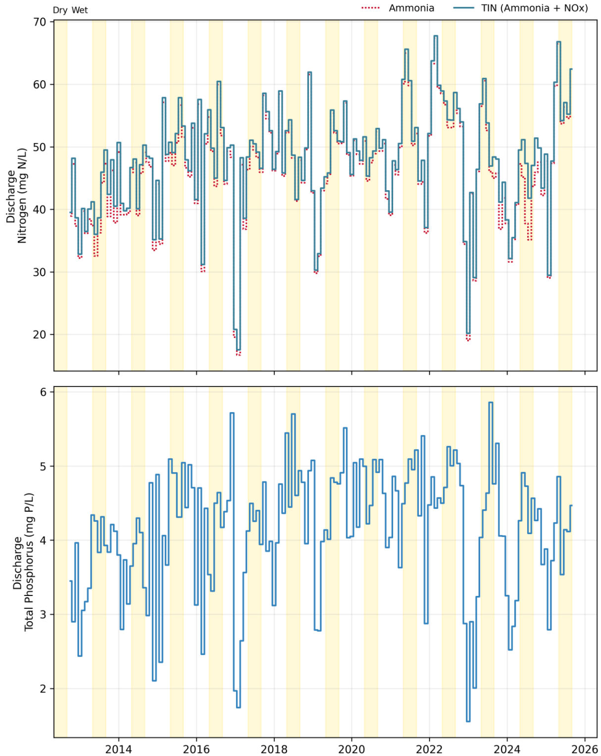
Figure 27-4. Discharge: SVCW Monthly Concentrations
