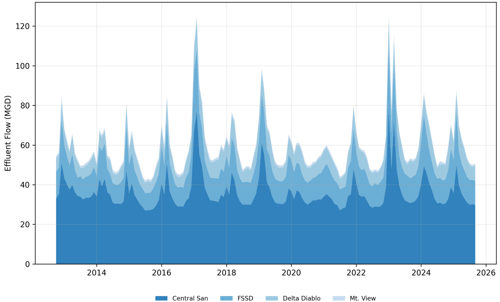
Figure C-1. Flow Contribution by Discharger to Suisun Bay
