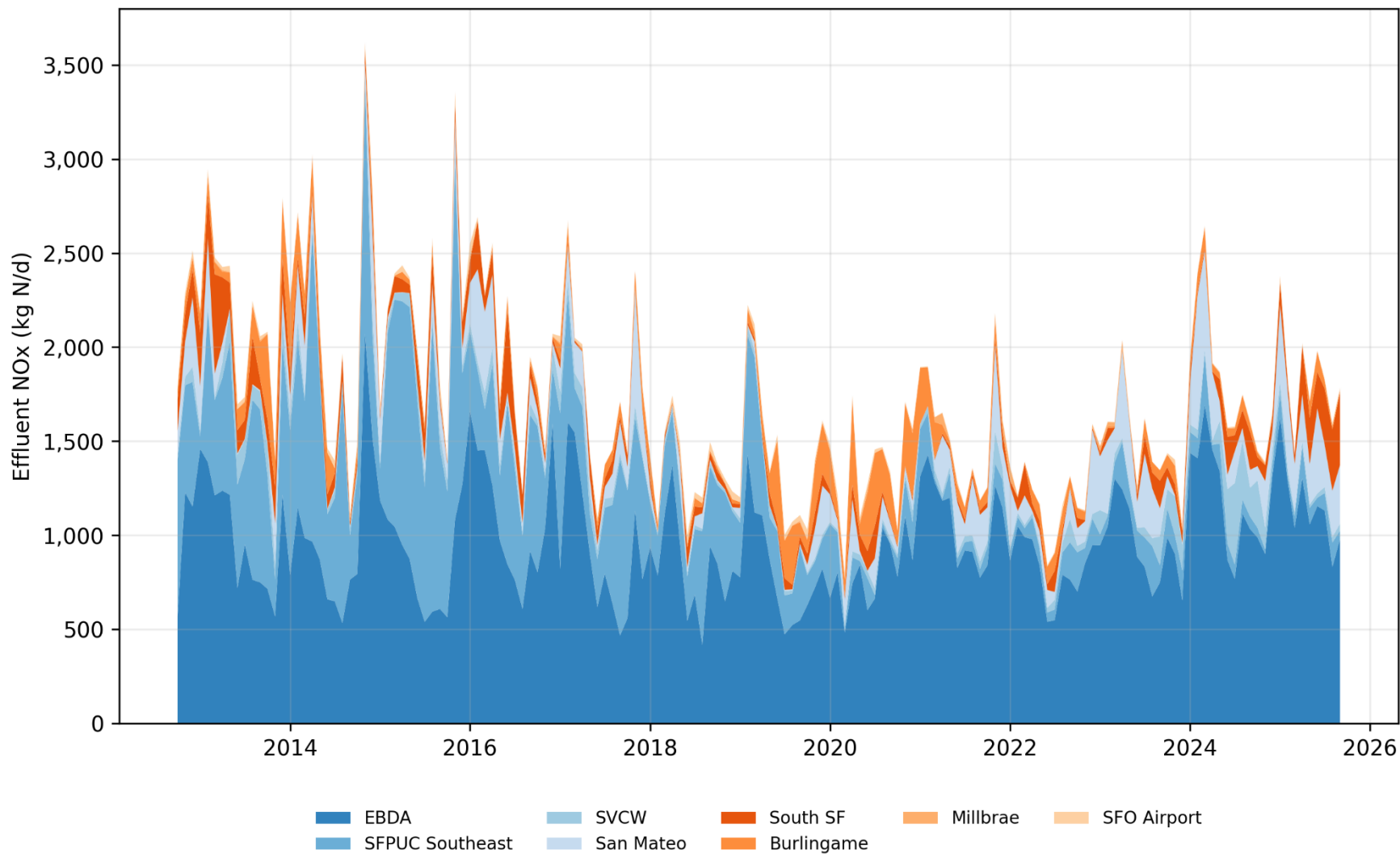
Figure C-18.NOx Load Contribution by Discharger to South Bay
