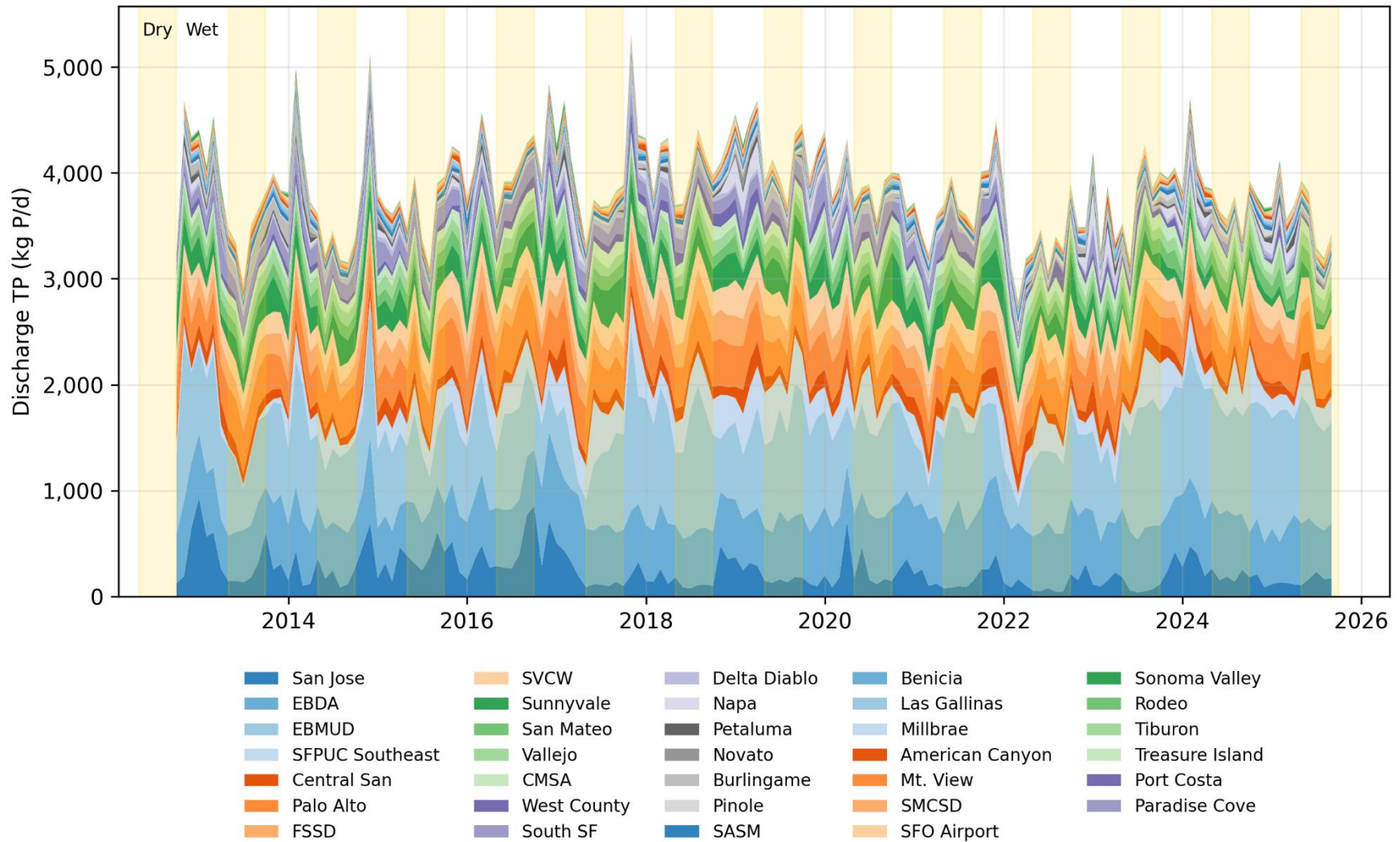
Figure B-9. Discharge: Average Monthly Discharge TP Loads
