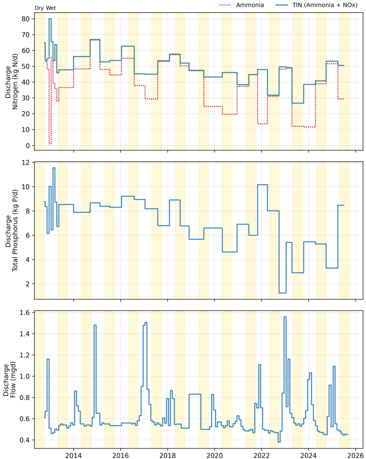
Fig-re 28-1. Discharge: Tiburon Monthly Flows and Loads
