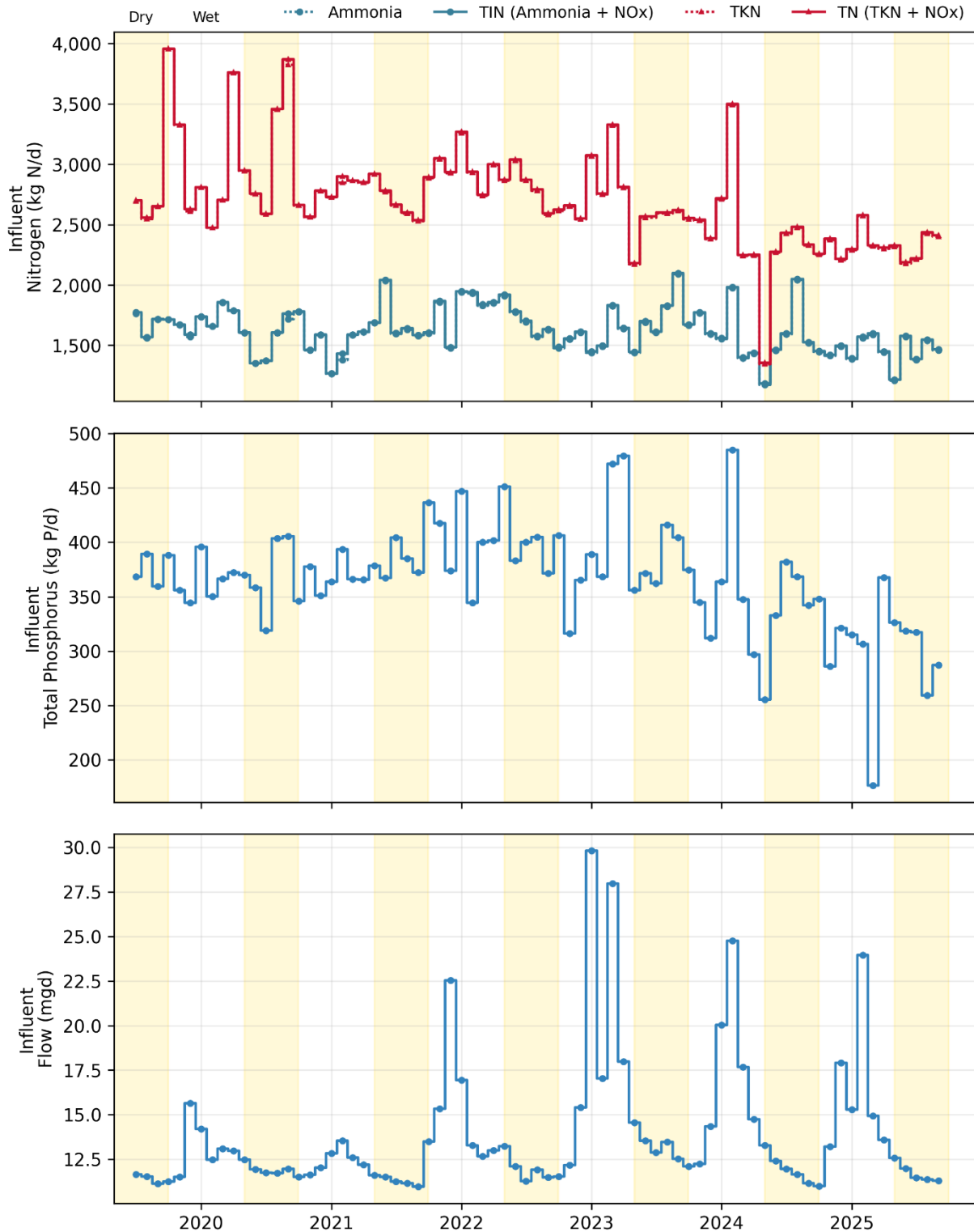
Figure 10-1. Influent: FSSD Monthly Flows and Loads
