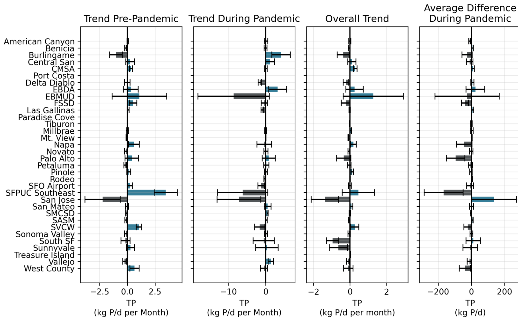
Figure B-10. Trend Coefficients for TP (95% Confidence Interval Shown in Black)
