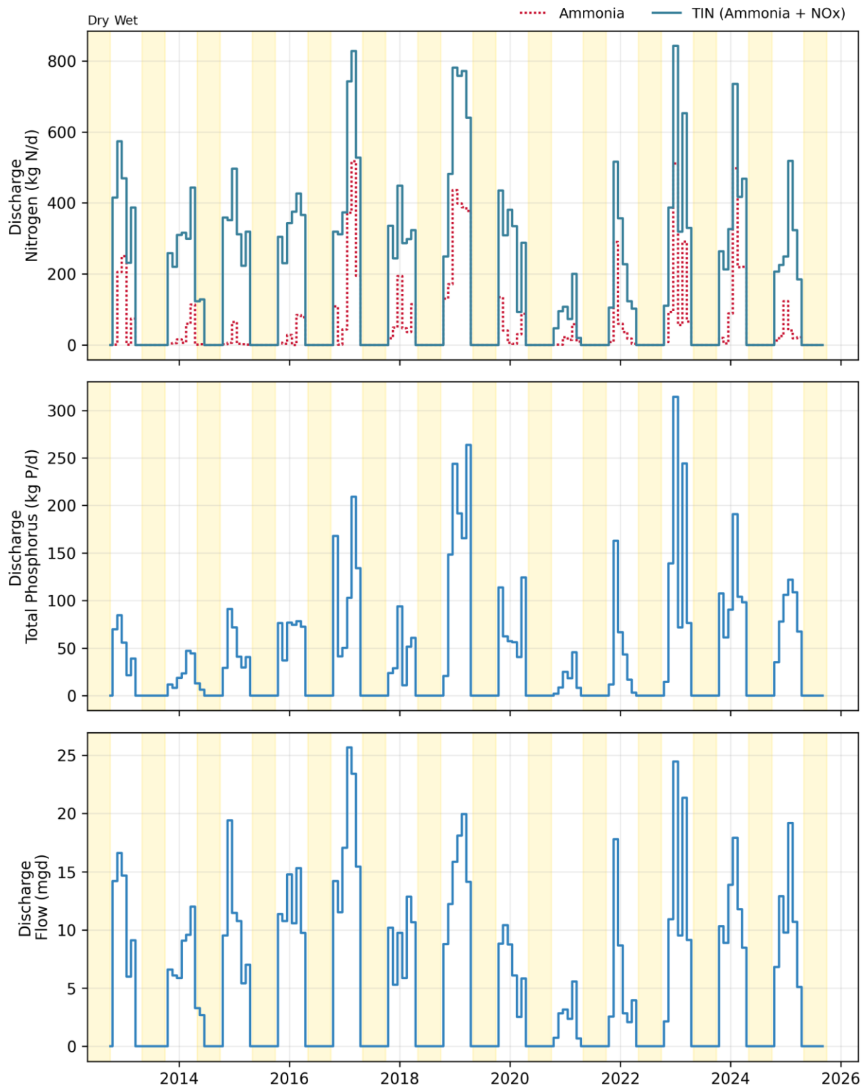
Figure 13-3. Discharge: Napa Sanitation District Monthly Flows and Loads
