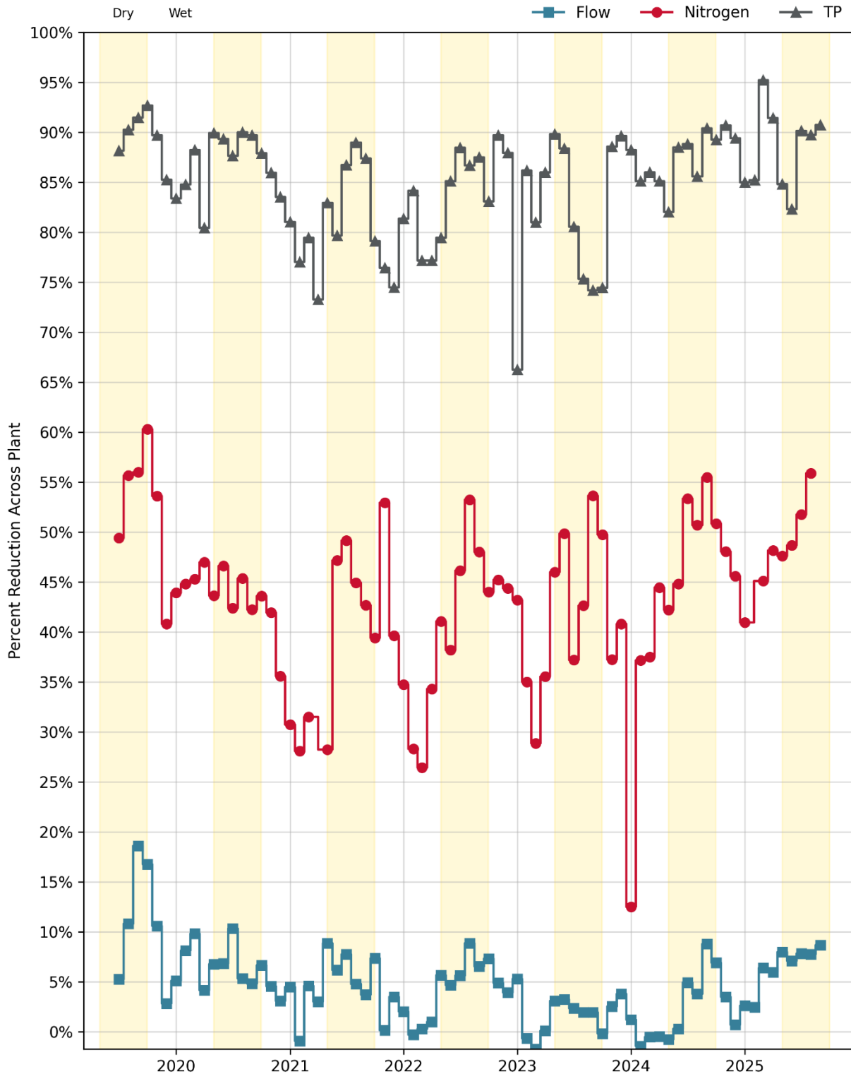
Figure 4-2. Influent: Central San Monthly Reductions Across the Plant
