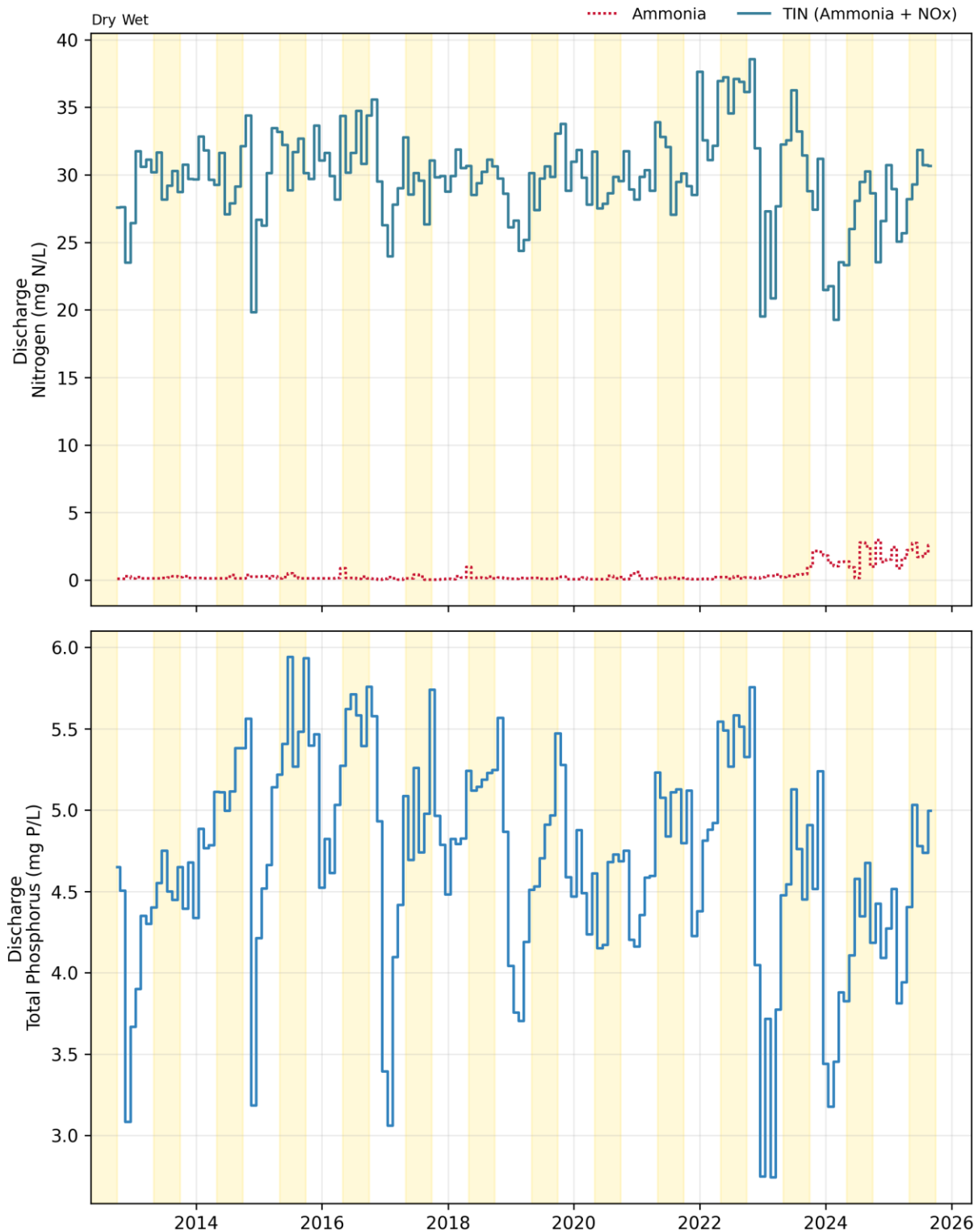
Figure 15-4. Discharge: Palo Alto Monthly Concentrations
