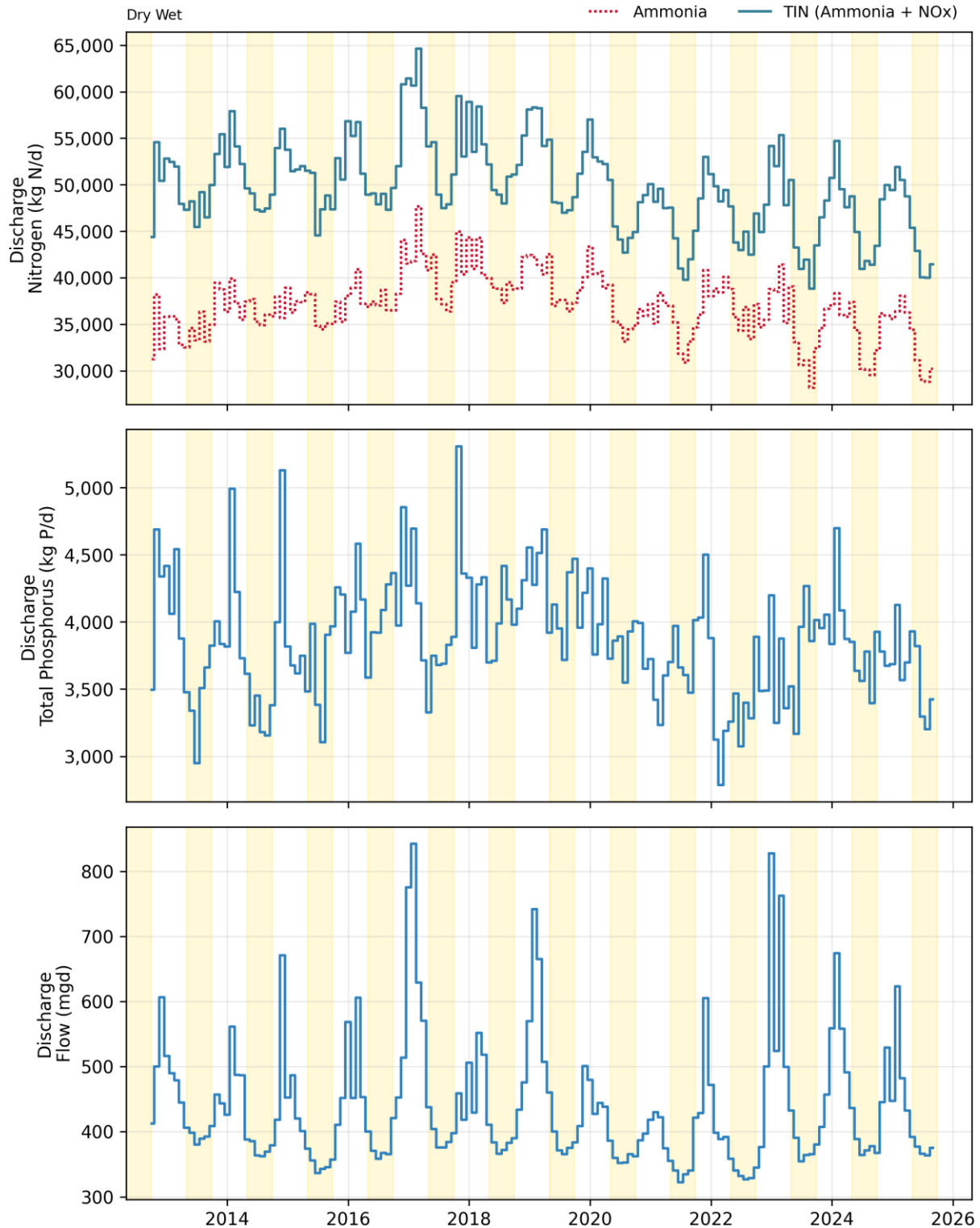
Figure 3-2. Historical Average Monthly Daily Discharge Flows and Loads
