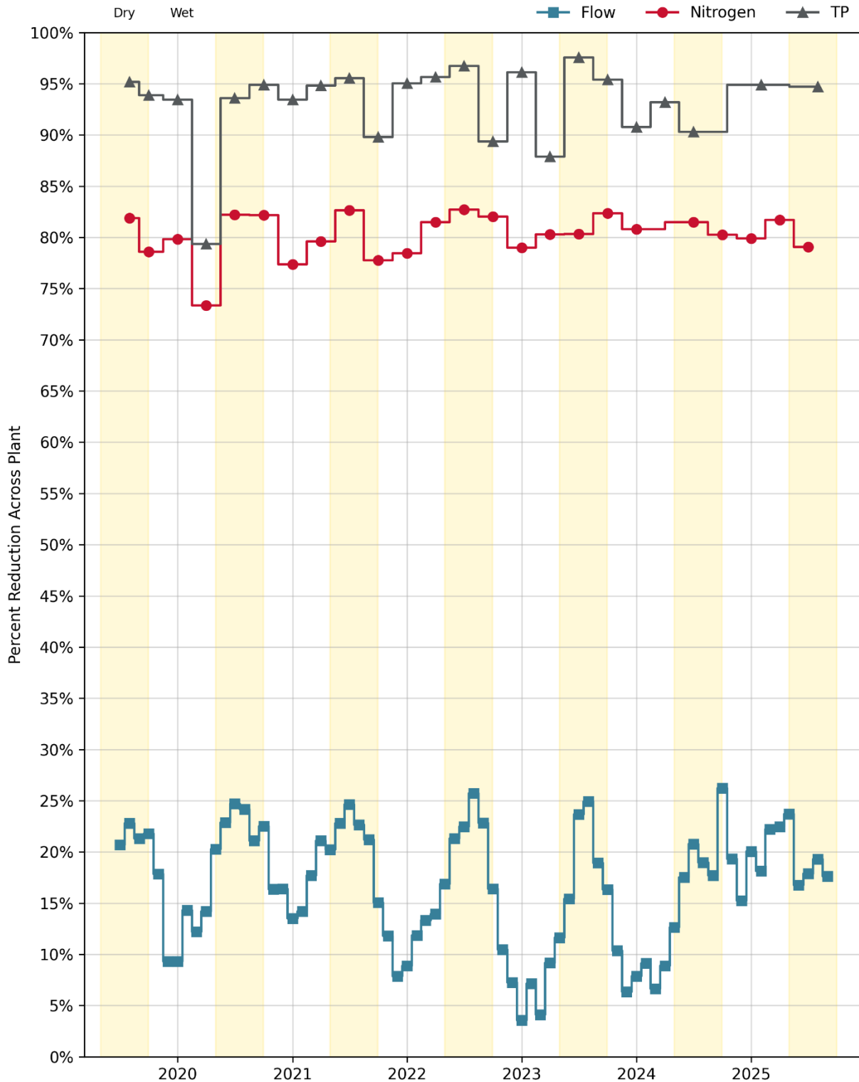
Figure 19-2. Influent: San Jose Monthly Reductions Across the Plant
