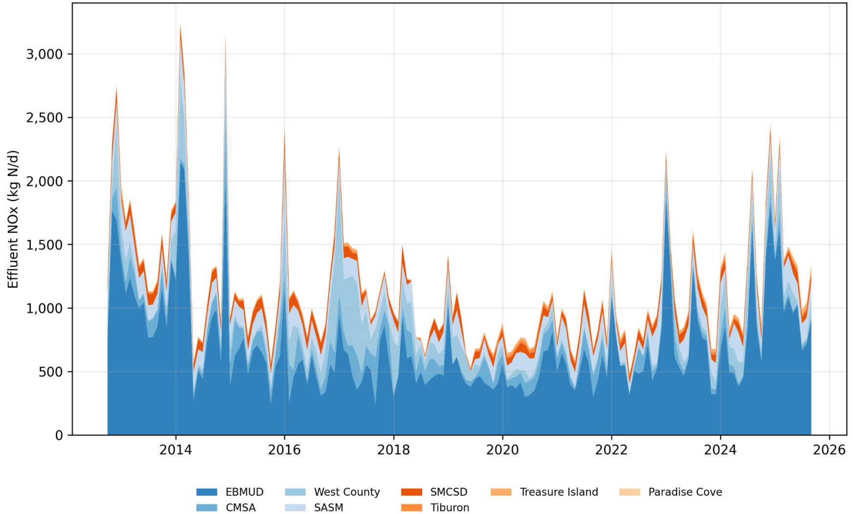
Figure C-13. NOx Load Contribution by Discharger to Central Bay
