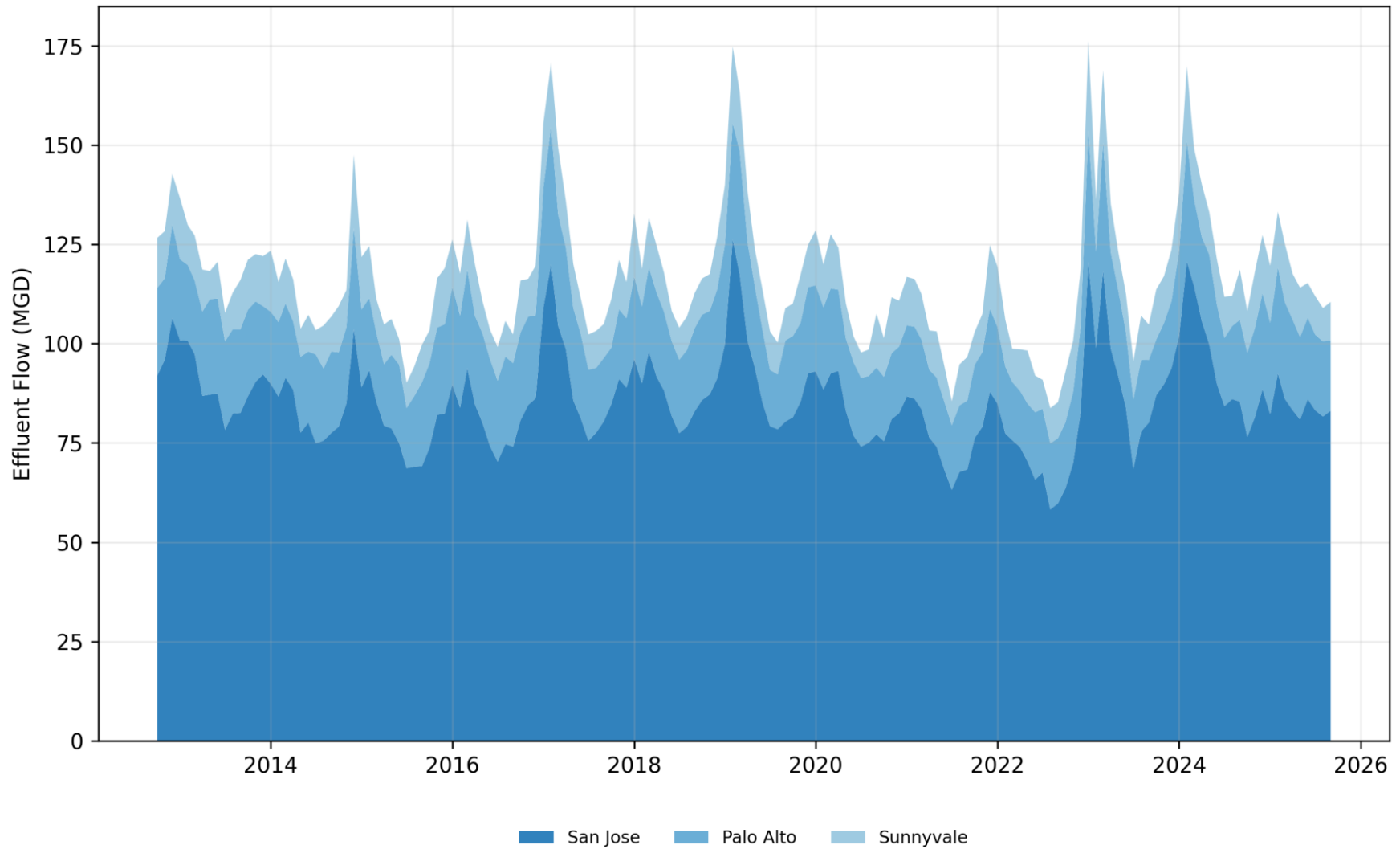
Figure C-21. Flow Contribution by Discharger to Lower South Bay
