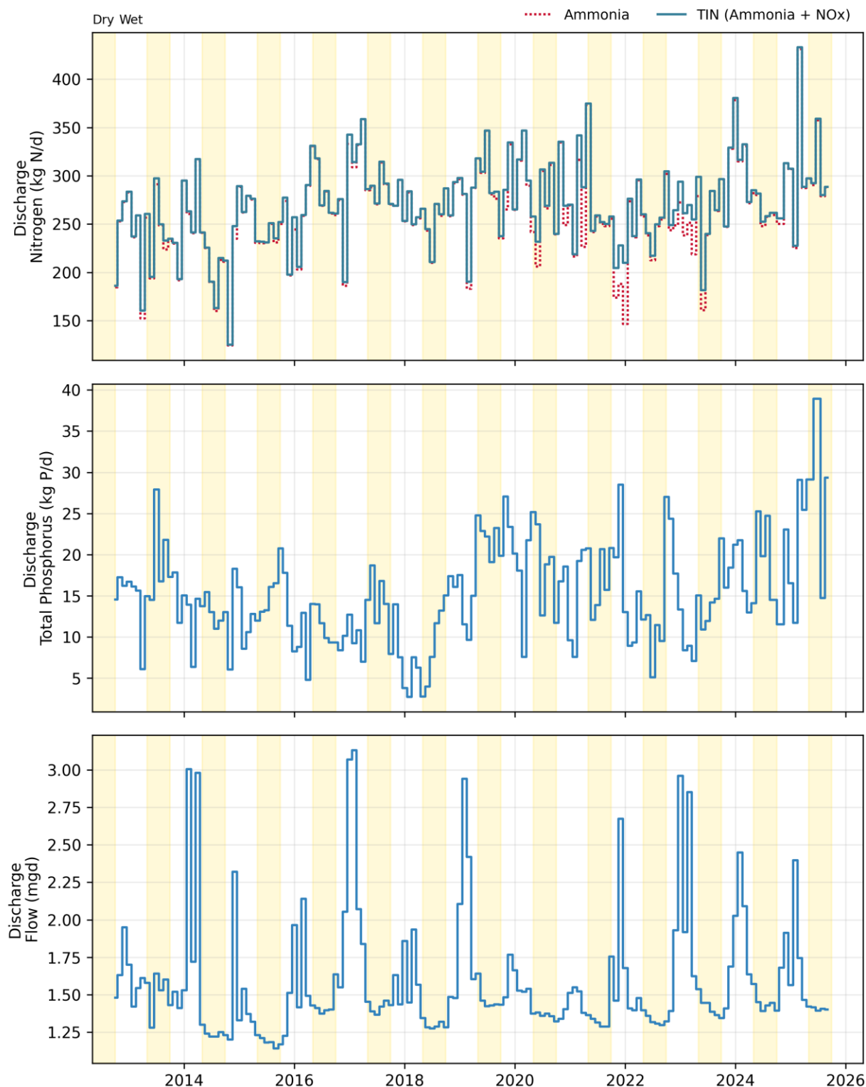
Figure 11-1. Discharge: Millbrae Monthly Flows and Loads
