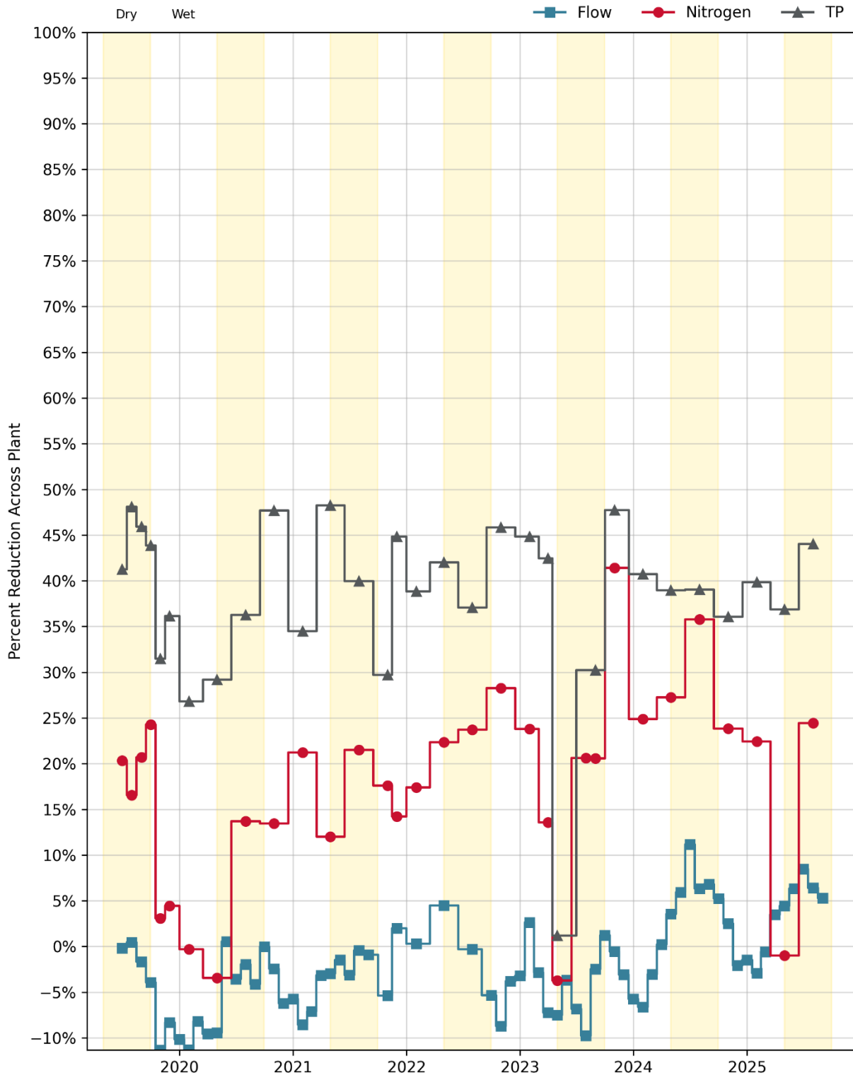
Figure 27-2. Influent: SVCW Monthly Reductions Across the Plant
