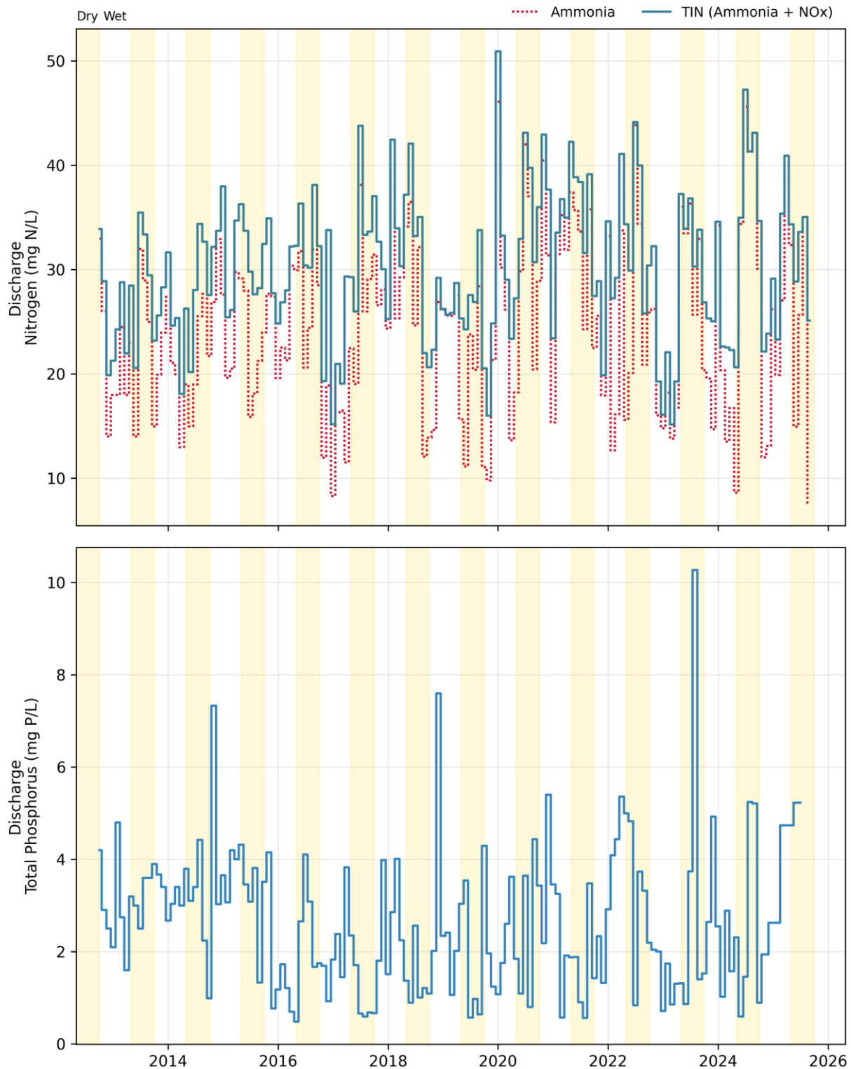
Figure 2-2. Discharge: Benicia Monthly Concentrations
