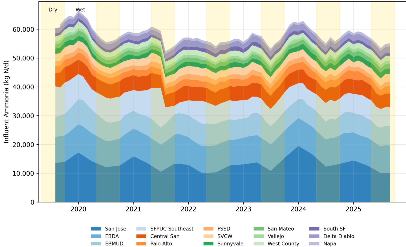
Figure A-2. Influent: Historical Average Quarterly Total Ammonia Loads
