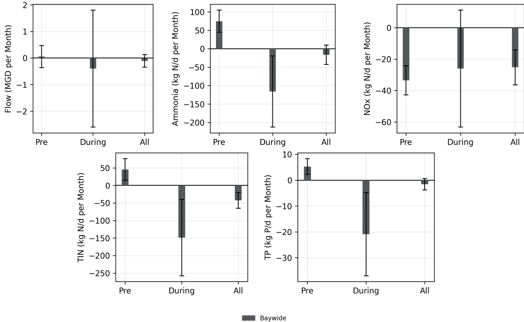
Figure 3-5. Flow and Load Trends for Pre-Pandemic, During Pandemic, and Across All Time for San Francisco Bay with 95% Confidence Interval
