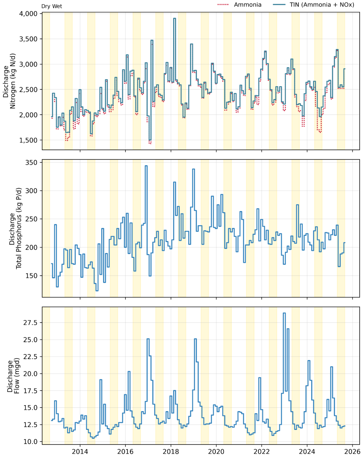
Figure 27-3. Discharge: SVCW Monthly Flows and Loads
