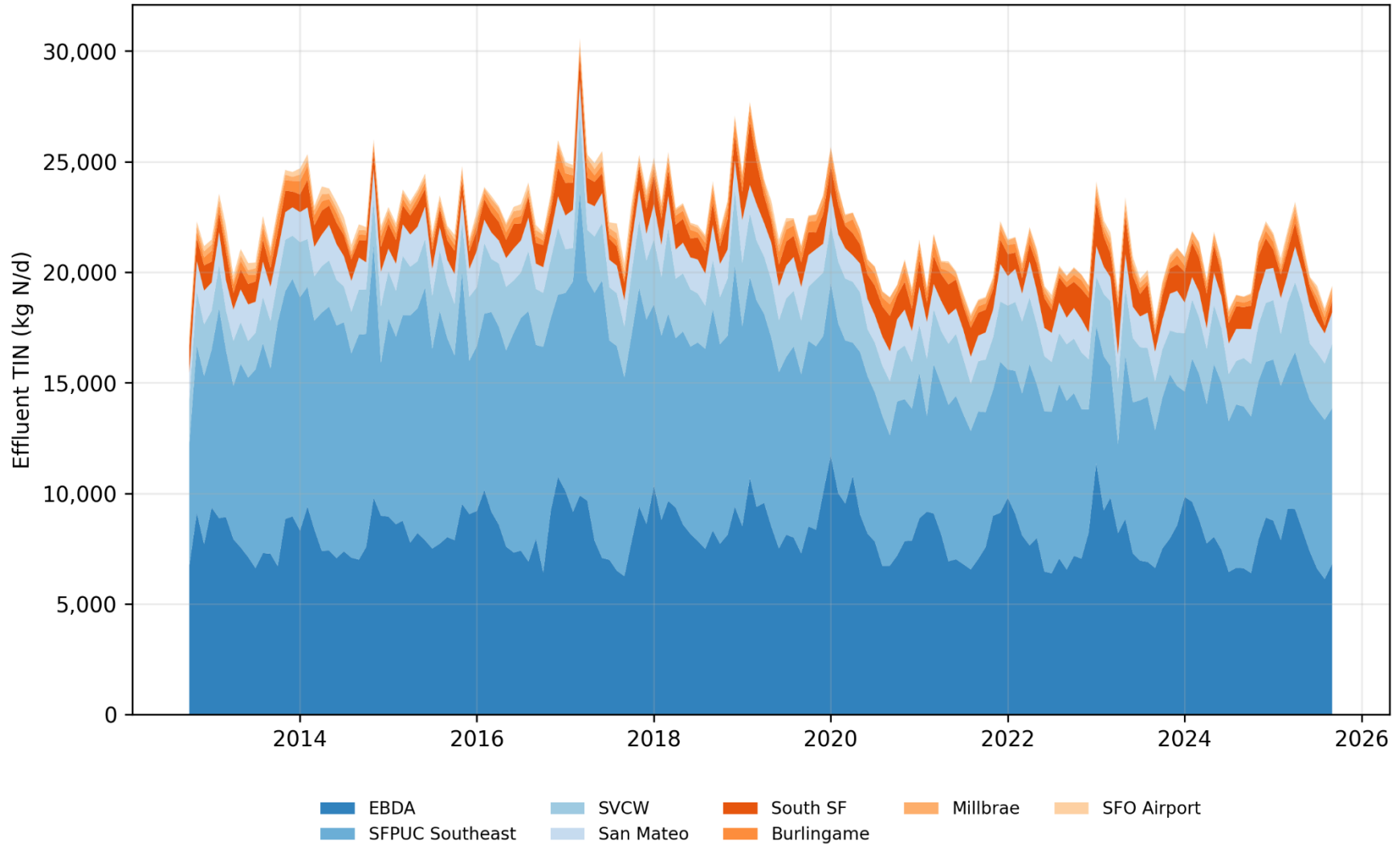
Figure C-19. TIN Load Contribution by Discharger to South Bay
