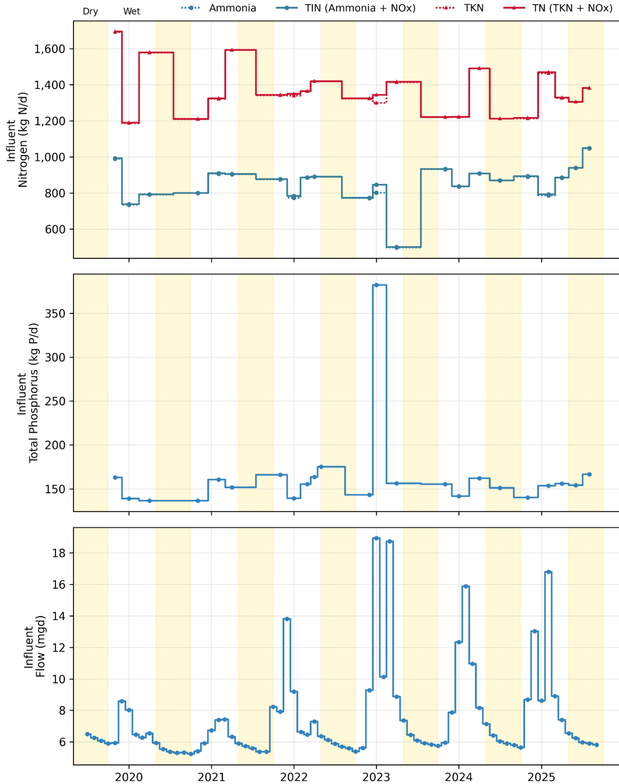
Figure 13-1. Influent: Napa Sanitation District Monthly Flows and Loads
