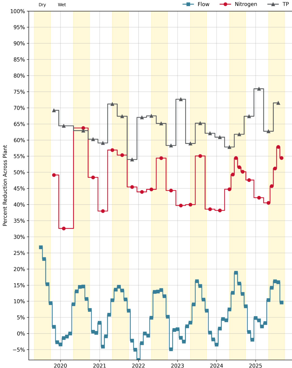
Figure 8-2. Influent: EBDA Monthly Reductions Across the Plants*
