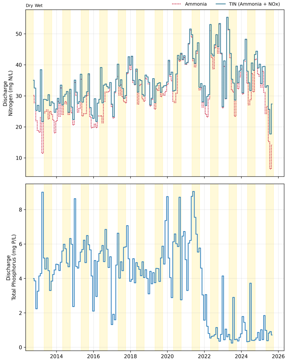
Figure 25-4. Discharge: South SF-San Bruno Monthly Concentrations
