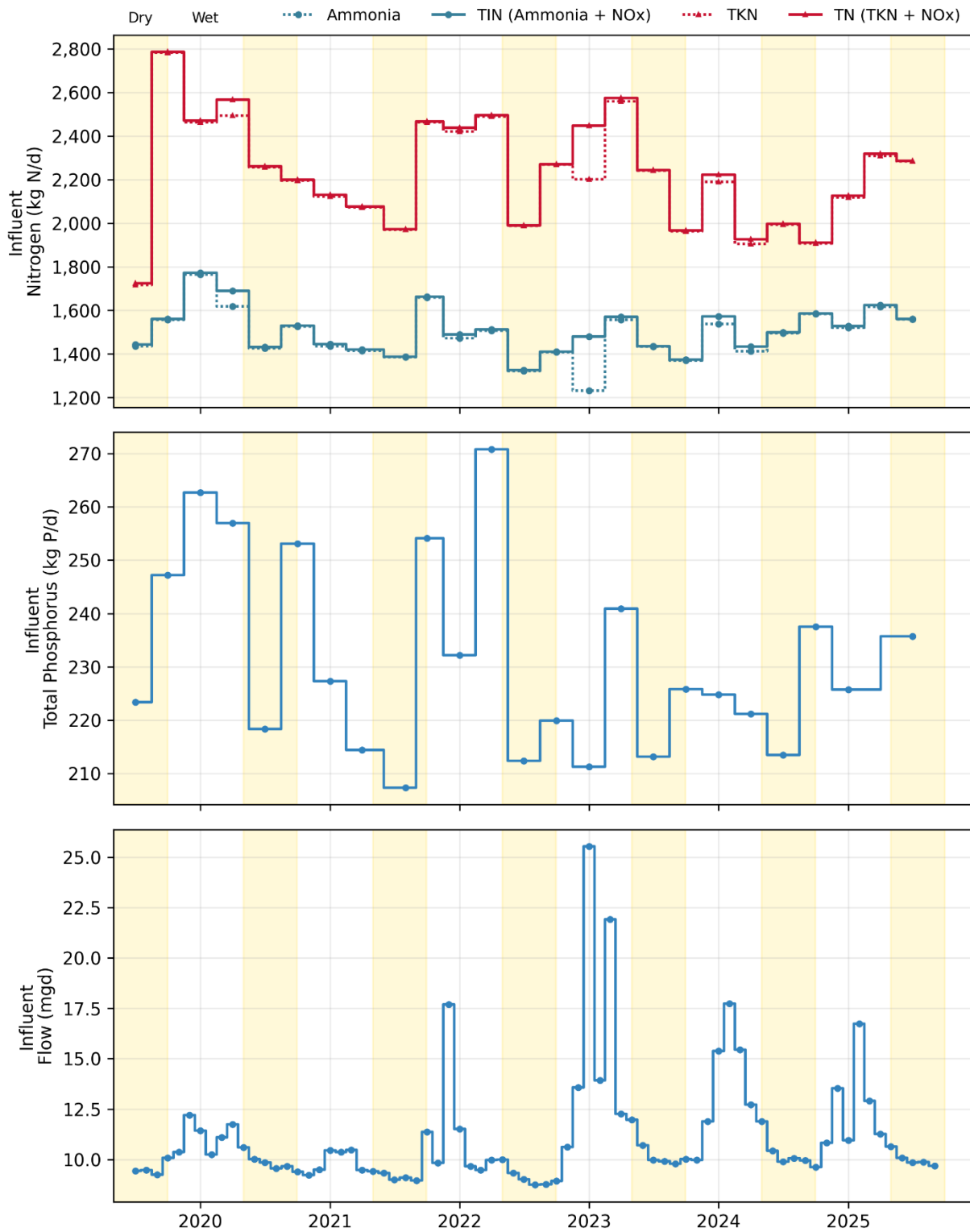
Figure 20-1. Influent: San Mateo Monthly Flows and Loads
