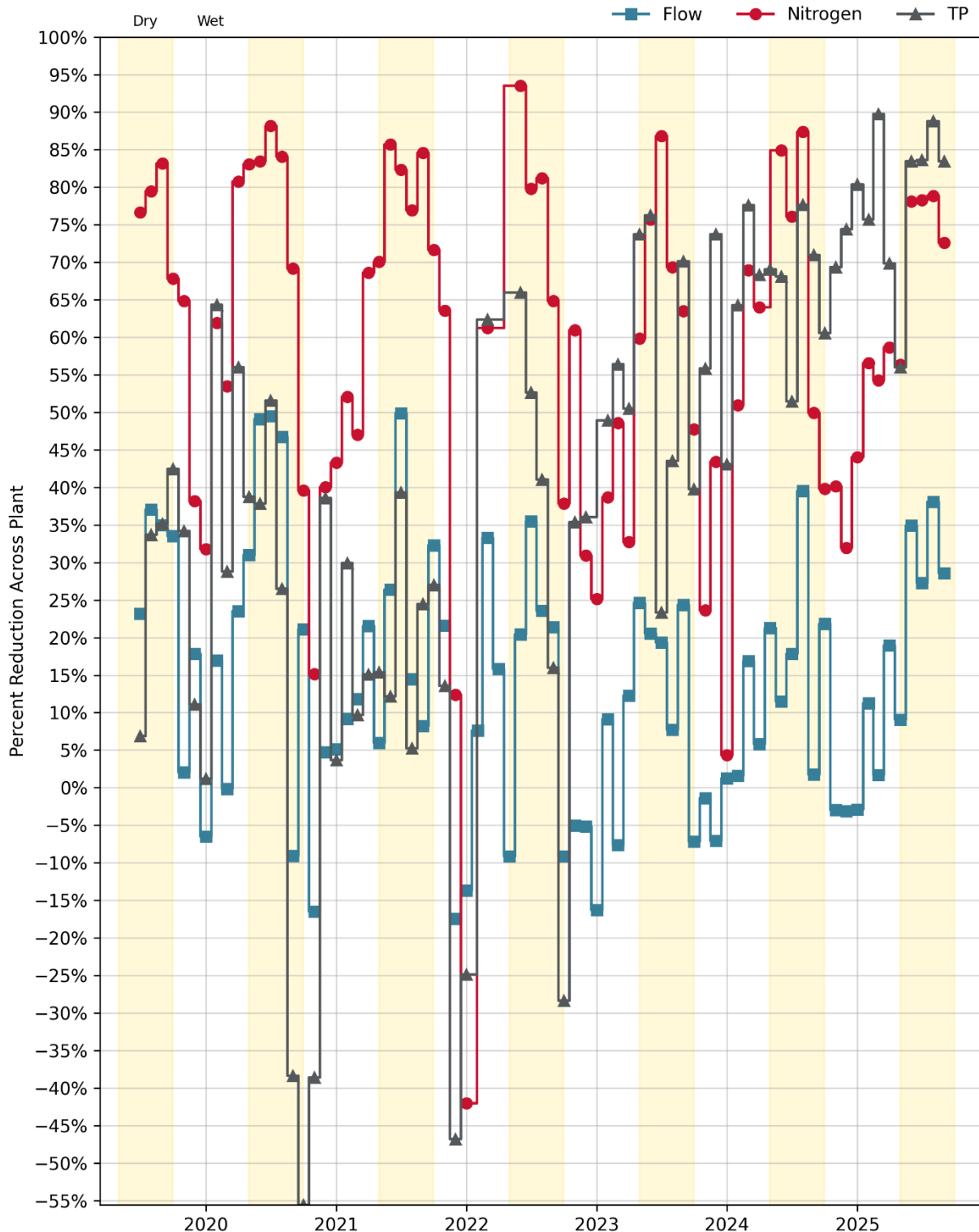
Figure 26-2. Influent: Sunnyvale Monthly Reductions Across the Plant*
