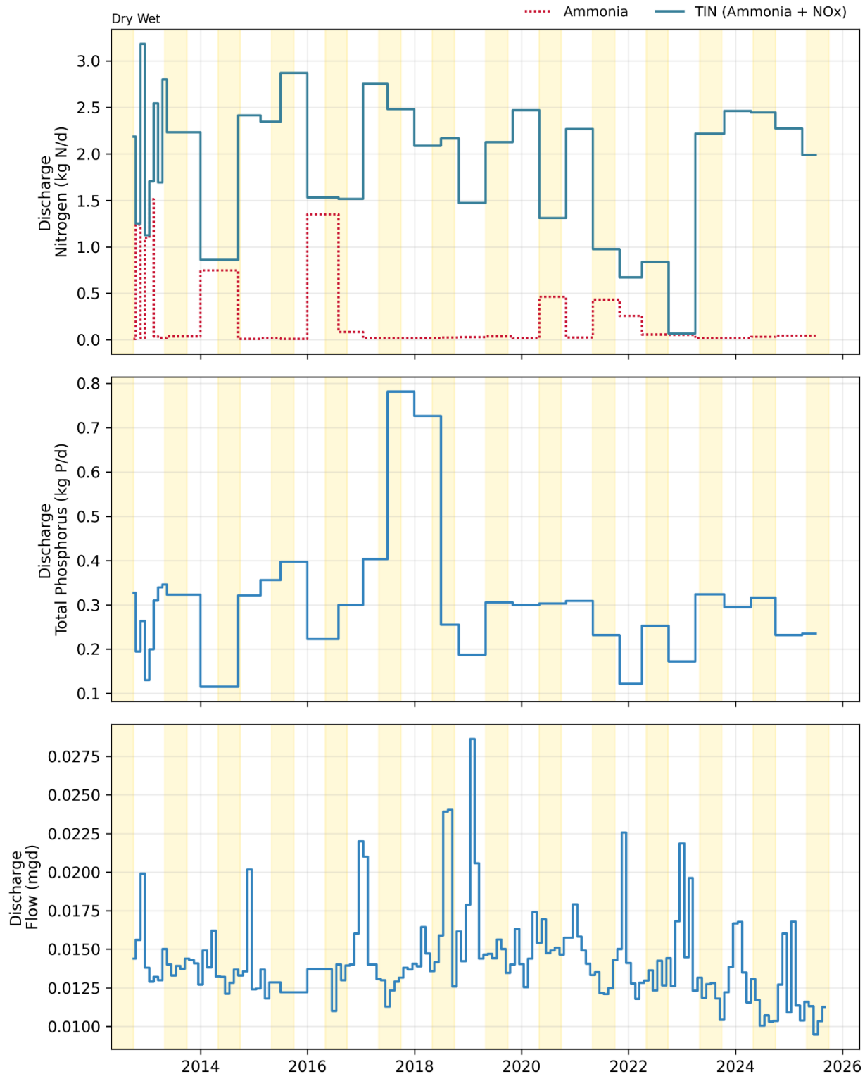
Figure 16-1. Discharge: Paradise Cove Monthly Flows and Loads
