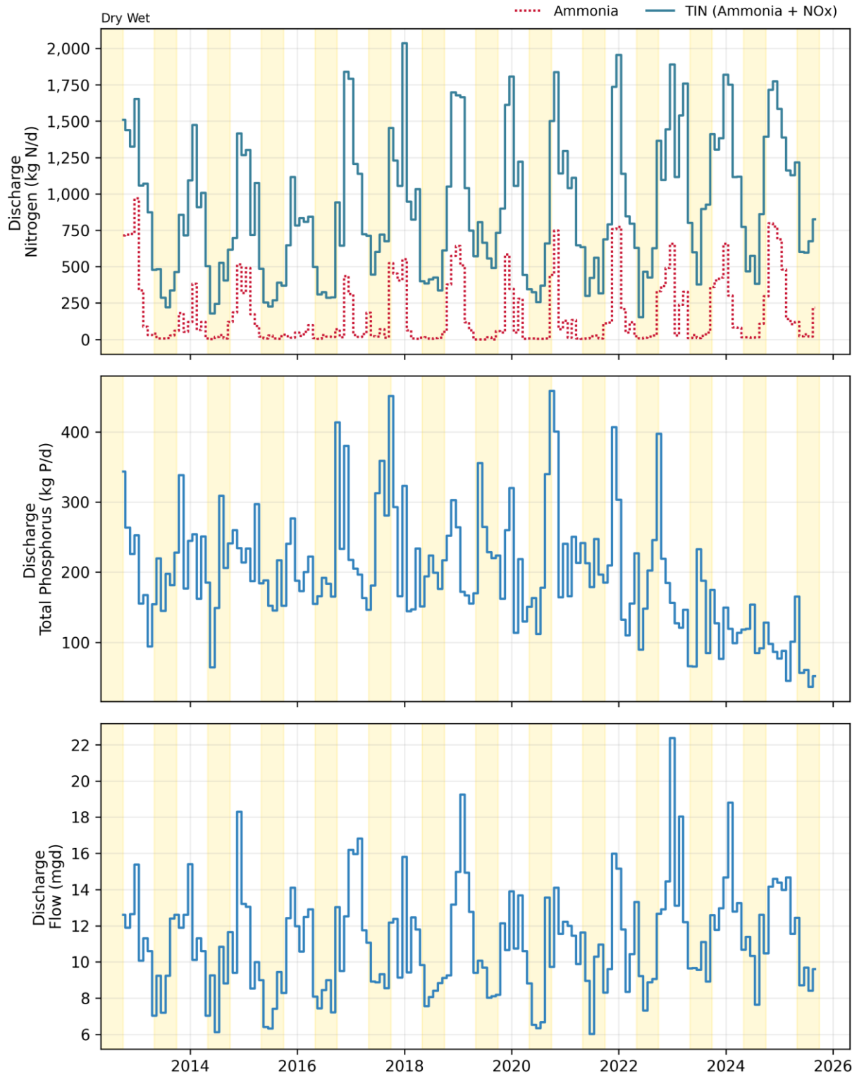
Figure 26-3. Discharge: Sunnyvale Monthly Flows and Loads
