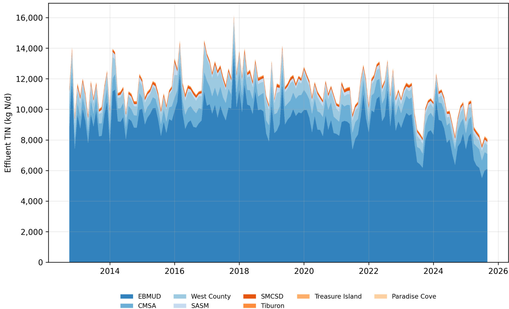
Figure C-14. TIN Load Contribution by Discharger to Central Bay
