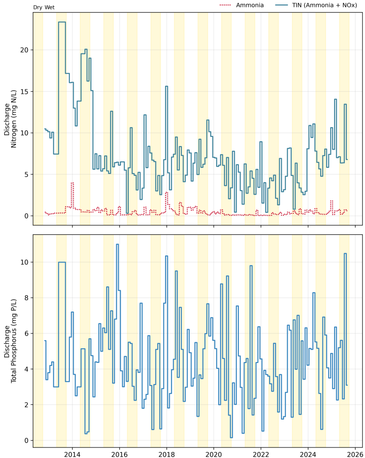
Figure 1-2. Discharge: American Canyon Monthly Nutrient Concentrations
