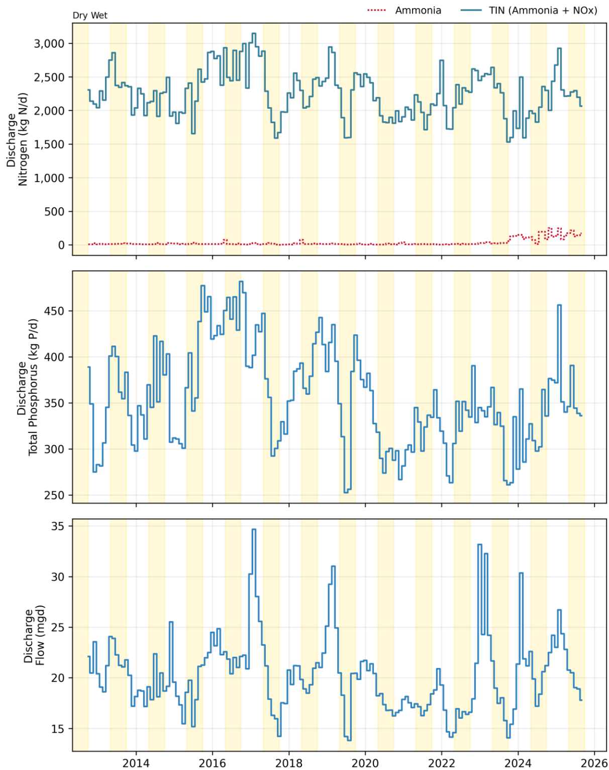
Figure 15-3. Discharge: Palo Alto Monthly Flows and Loads
