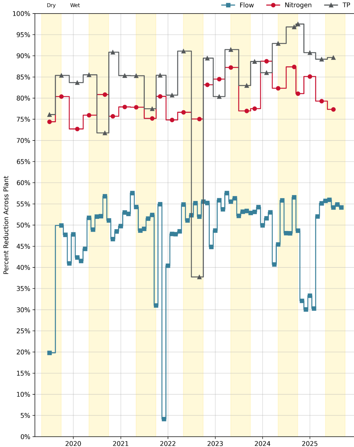
Figure 31-2. Influent: Monthly Reductions Across Both Treatment Plants
