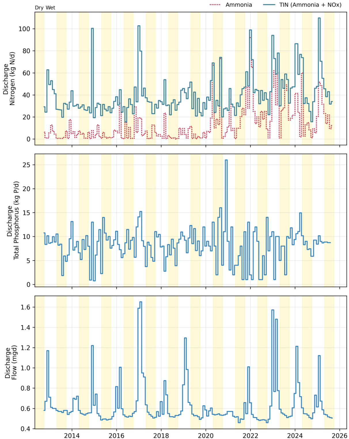
Figure 18-1. Discharge: Rodeo Monthly Flows and Loads
