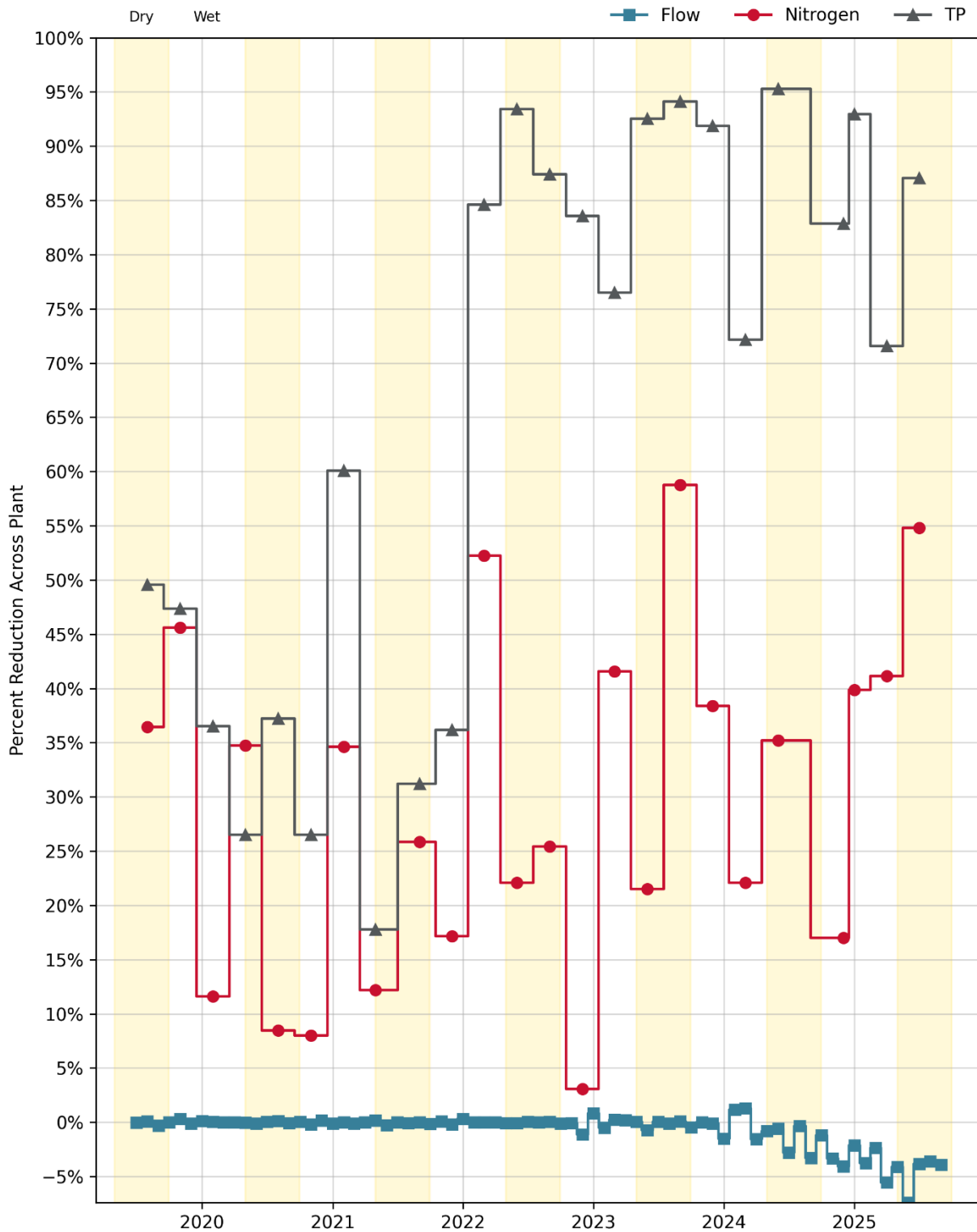
Figure 25-2. Influent: South SF-San Bruno Monthly Reductions Across the Plant*
