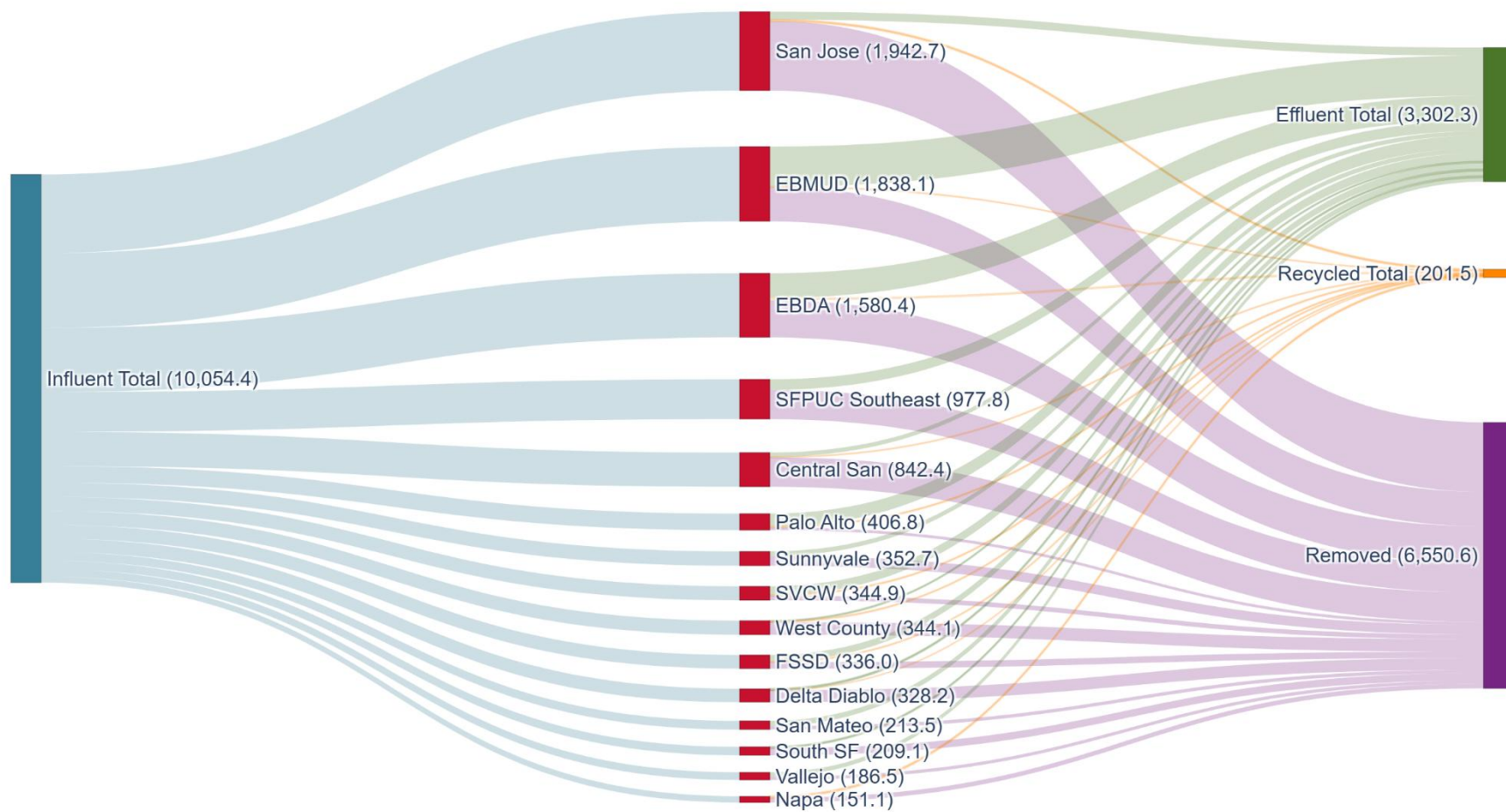
Figure 3-10. Dry Season Influent, Effluent, and Recycled Water TP Loads (kg P/d)
