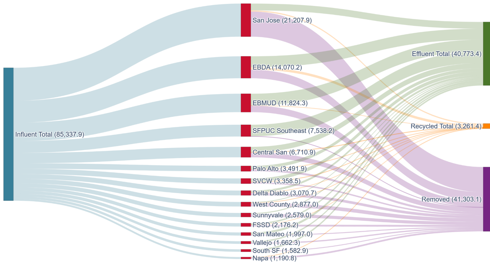
Figure 3-9. Dry Season Influent (TN), Effluent (TIN), and Recycled Water (TIN) Loads (kg N/d)
