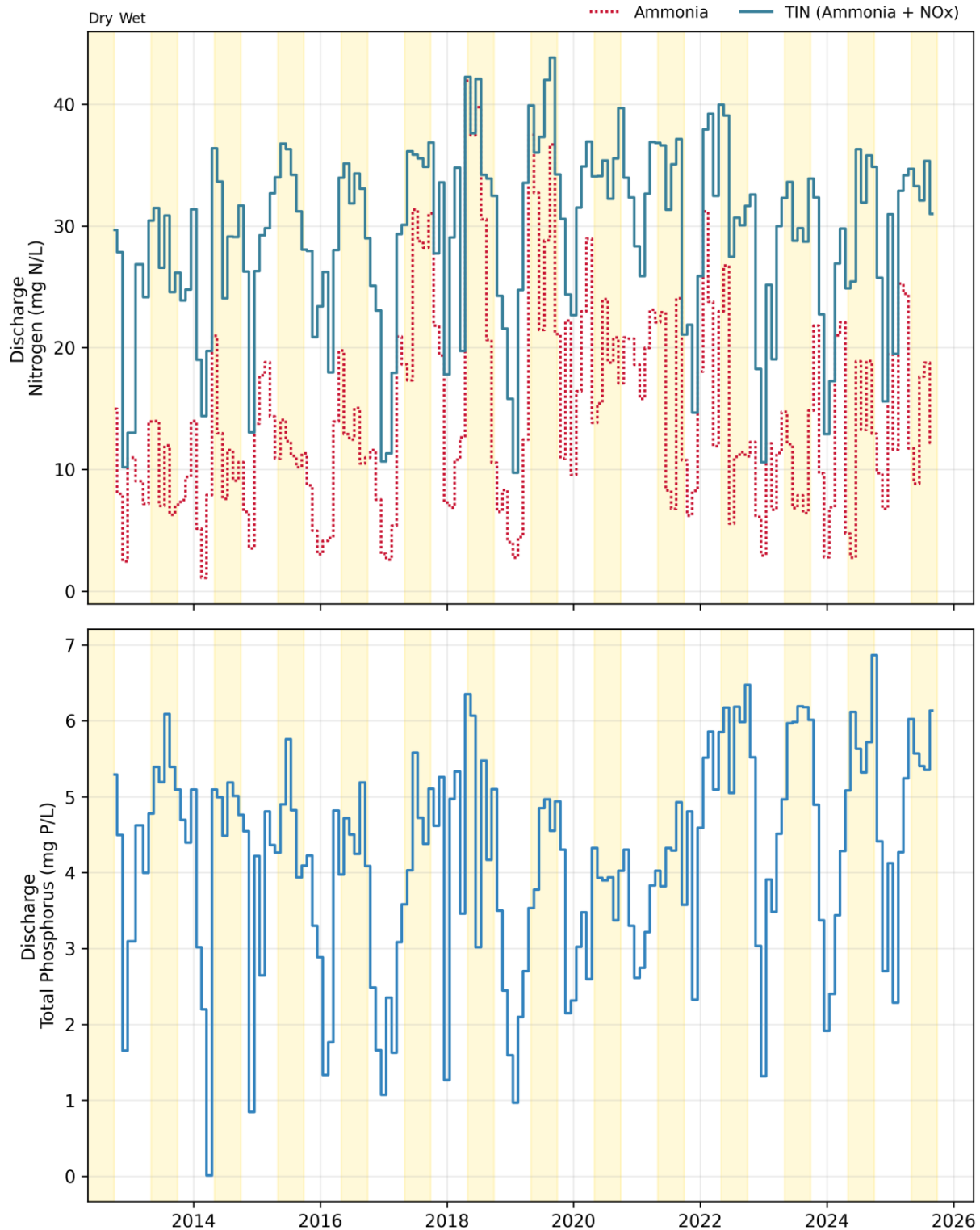
Figure 24-2. Discharge: SMCSO Monthly Concentrations
