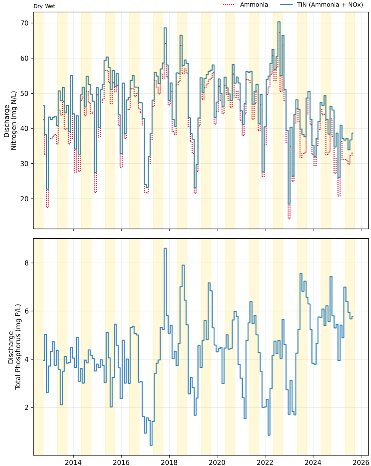
Figure 9-3. Discharge: EBMUD Monthly Concentrations
