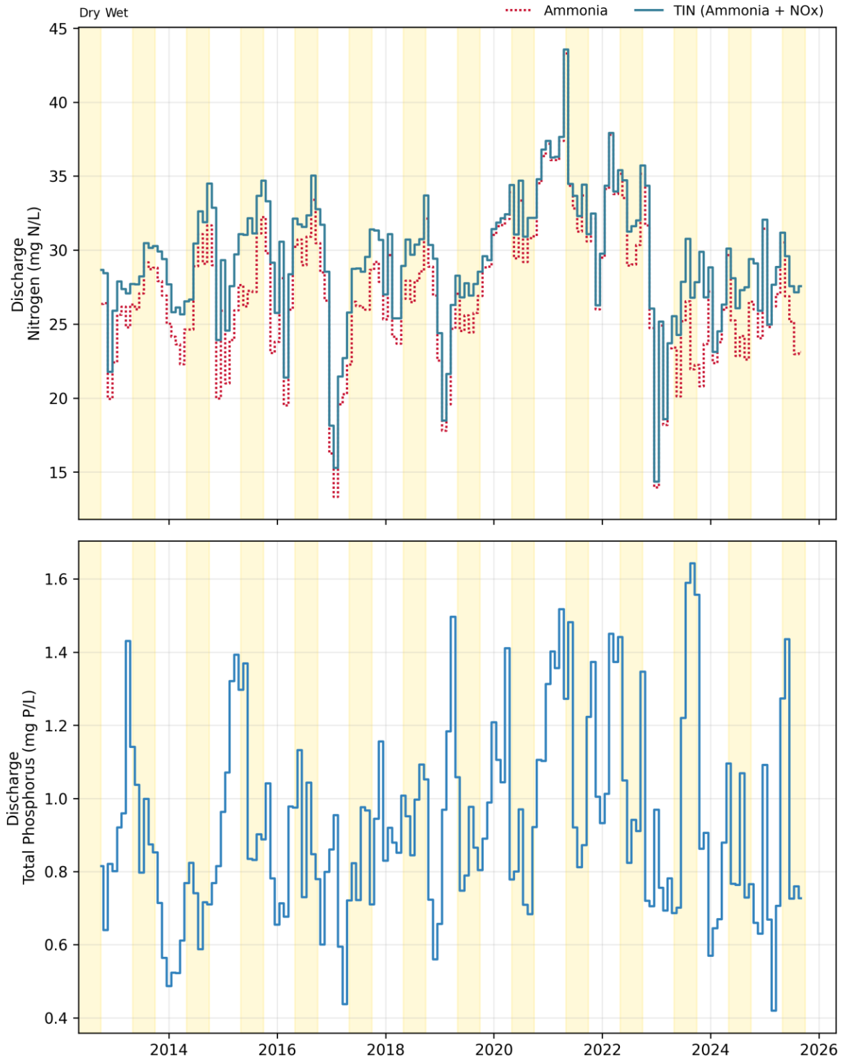
Figure 4-4. Discharge: Central San Monthly Concentrations
