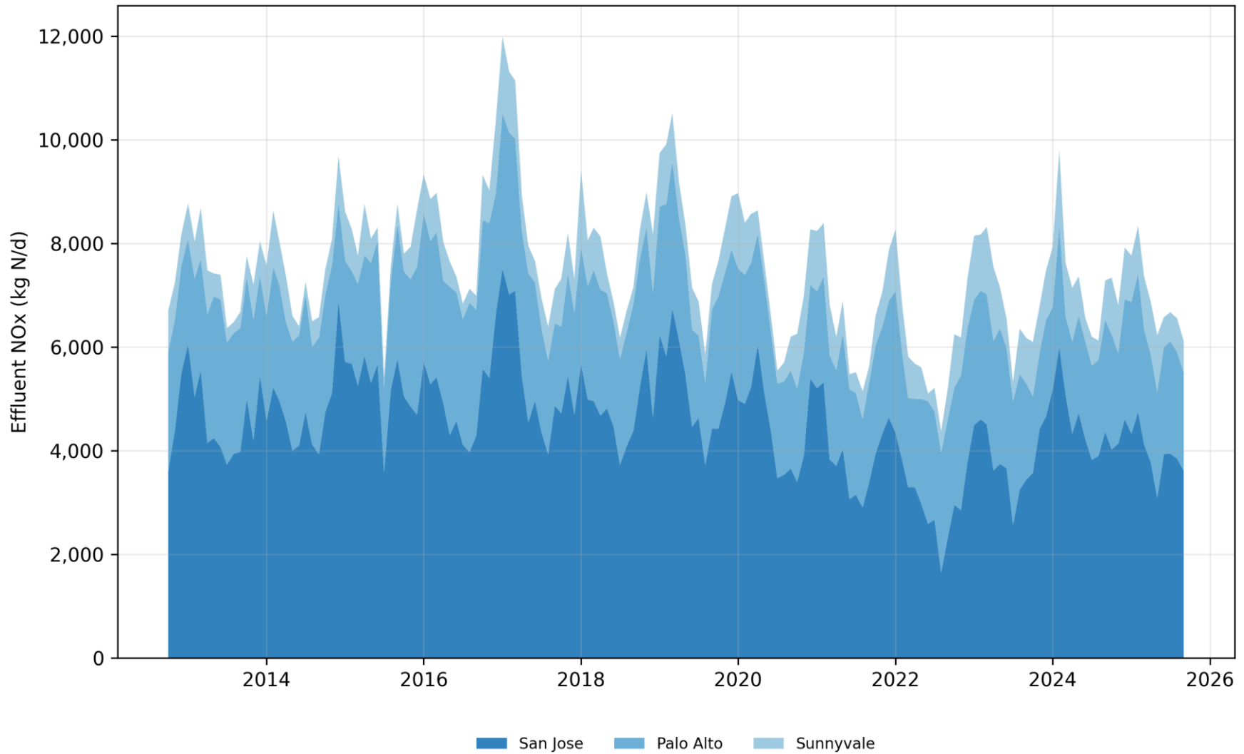
Figure C-23. Ammonia Load Contribution by Discharger to Lower South Bay
