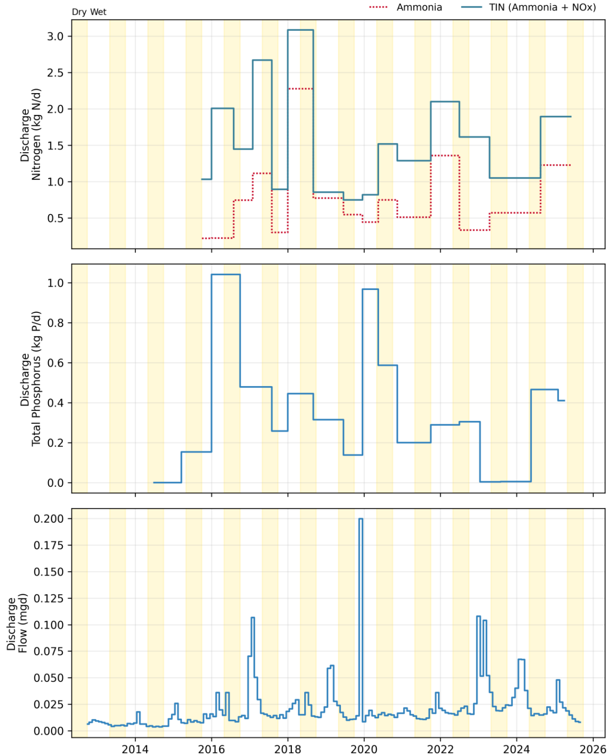
Figure 6-1. Discharge: Port Costa Monthly Flows and Loads
