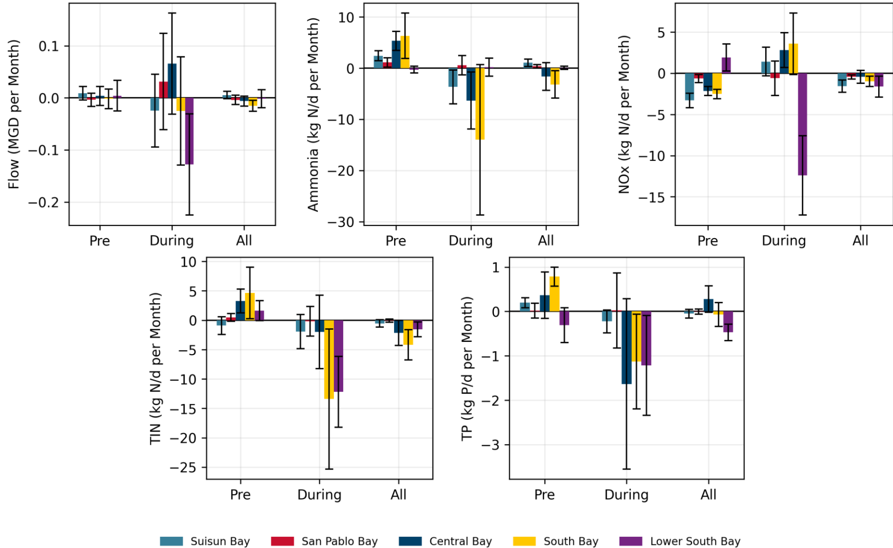
Figure 3-6. Flow and Load Trends for Subembayments Pre-Pandemic, During Pandemic, and Throughout the Study Period Without Accounting for the Pandemic (All), with 95% Confidence Interval
