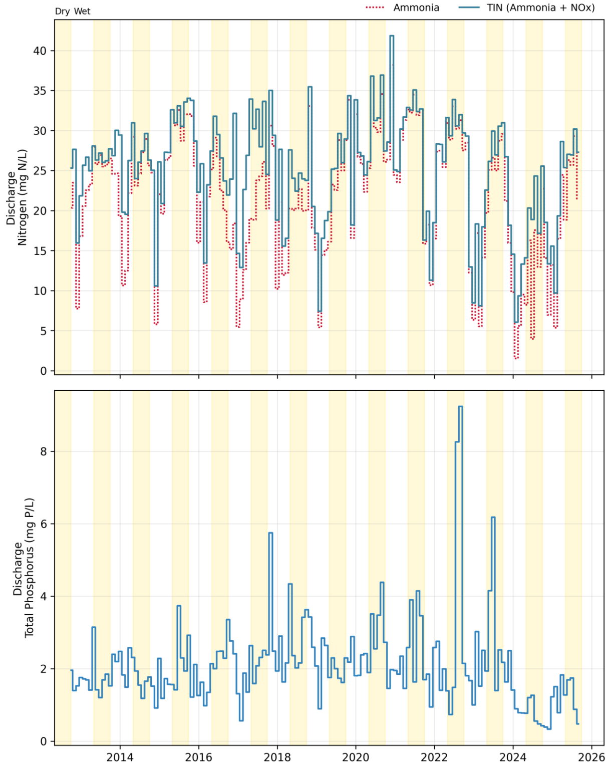
Figure 31-4. Discharge: Monthly Concentrations for Both Treatment Plants at the Common Outfall
