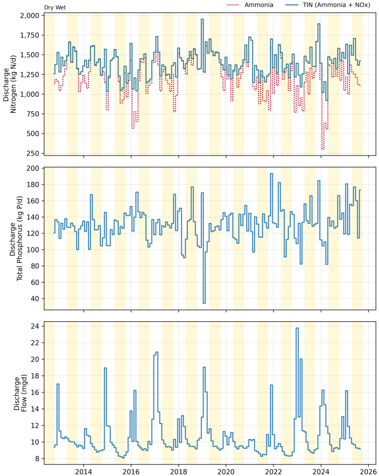
Figure 20-3. Discharge: San Mateo Monthly Flows and Loads
