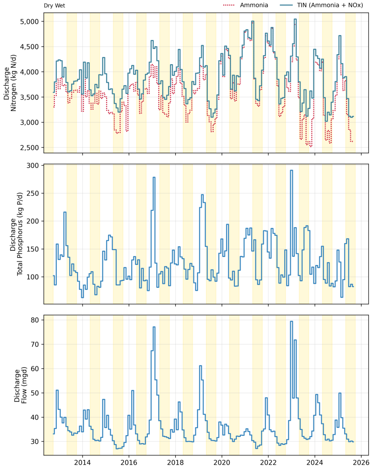
Figure 4-3. Discharge: Central San Monthly Flows and Loads
