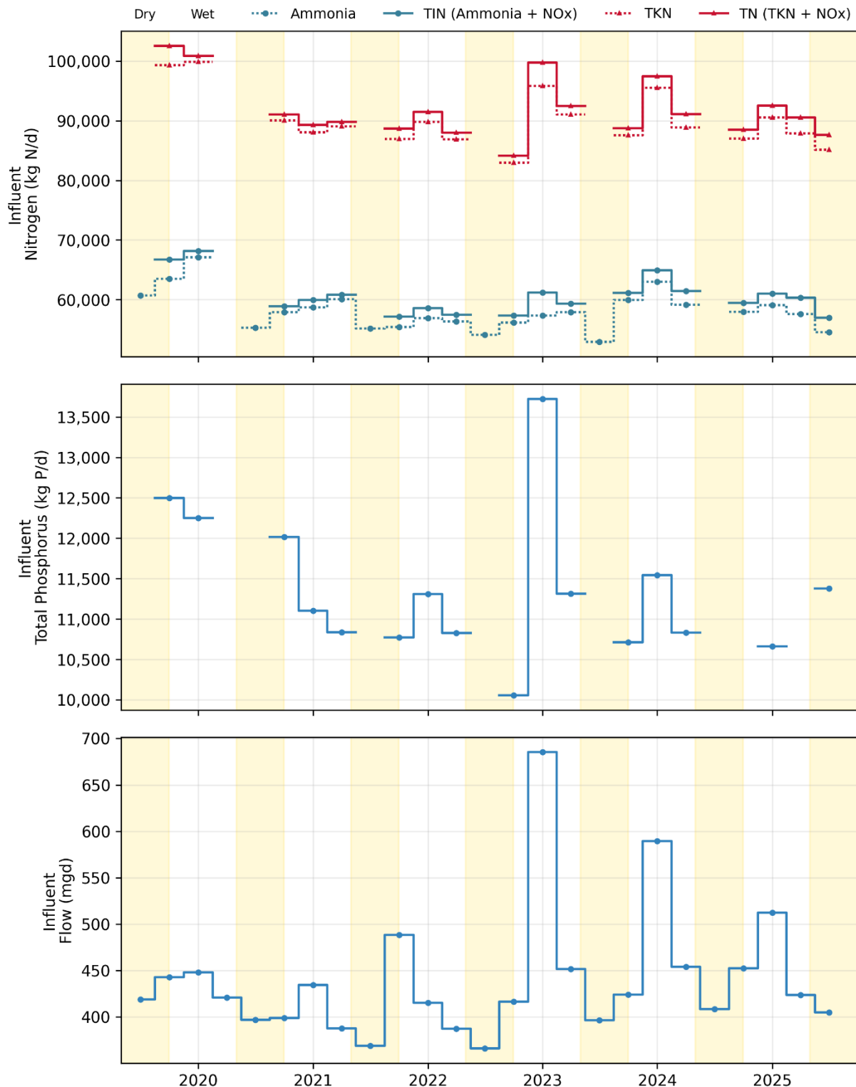
Figure 3-1. Historical Average Quarterly Influent Flows and Loads for Facilities Required to Report Influent Concentrations
