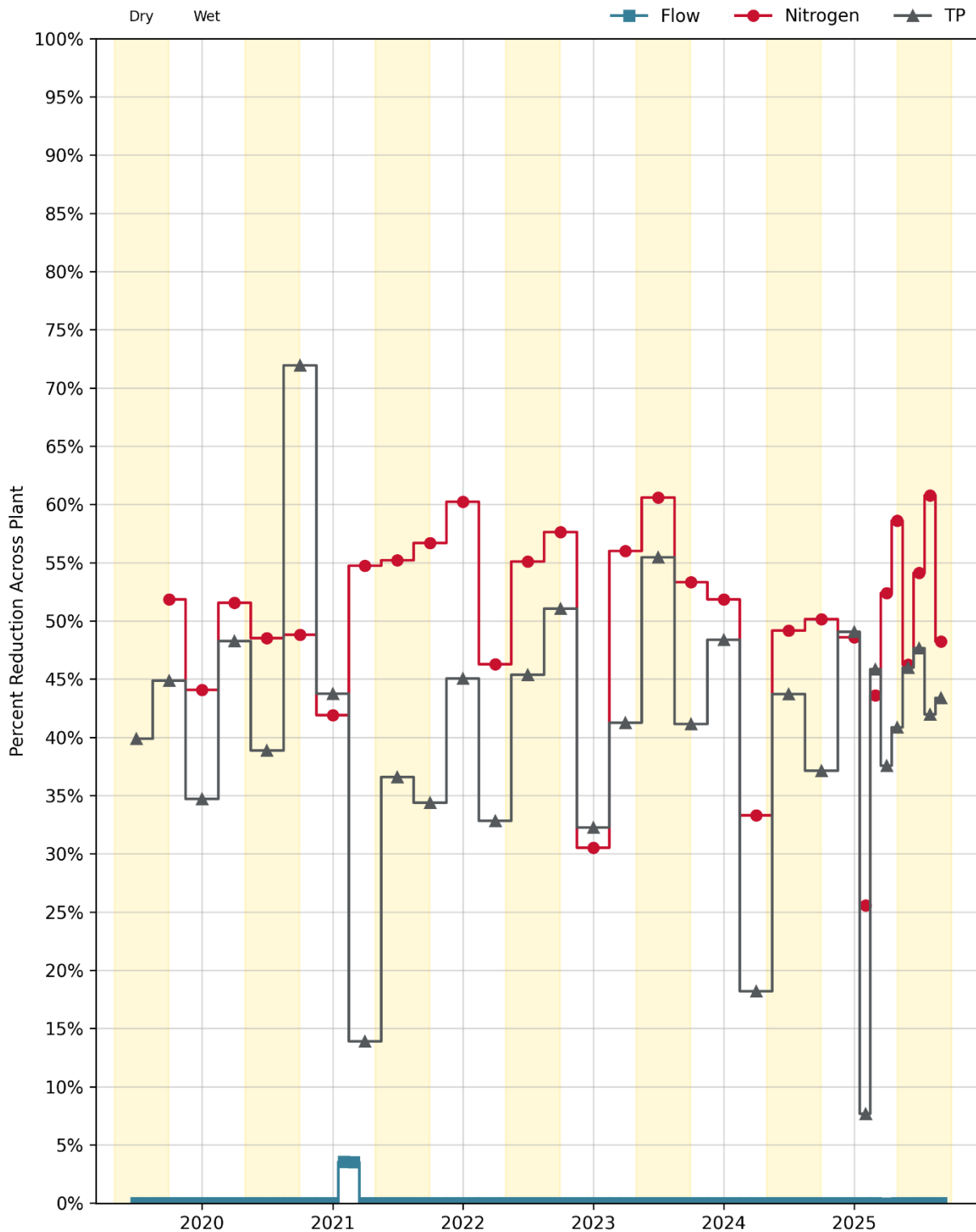
Figure 30-2. Influent: Vallejo Monthly Reductions Across the Plant
