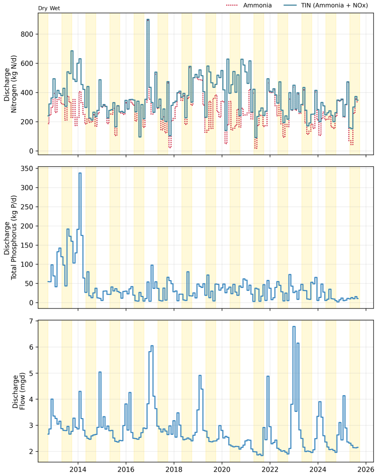
Figure 3-1. Discharge: Burlingame Monthly Flows and Loads
