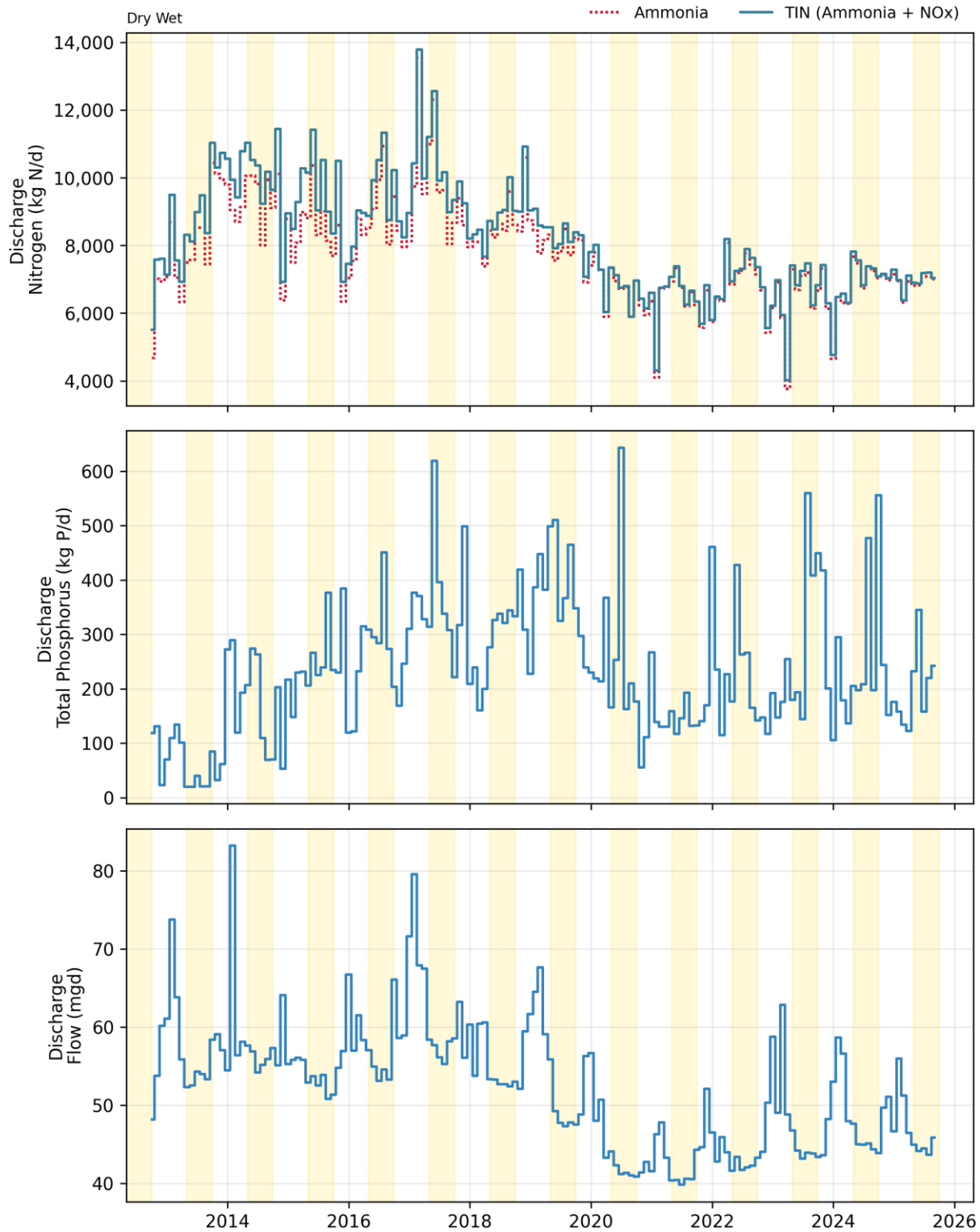
Figure 23-2. Discharge: SFPUC Southeast Monthly Flows and Loads
