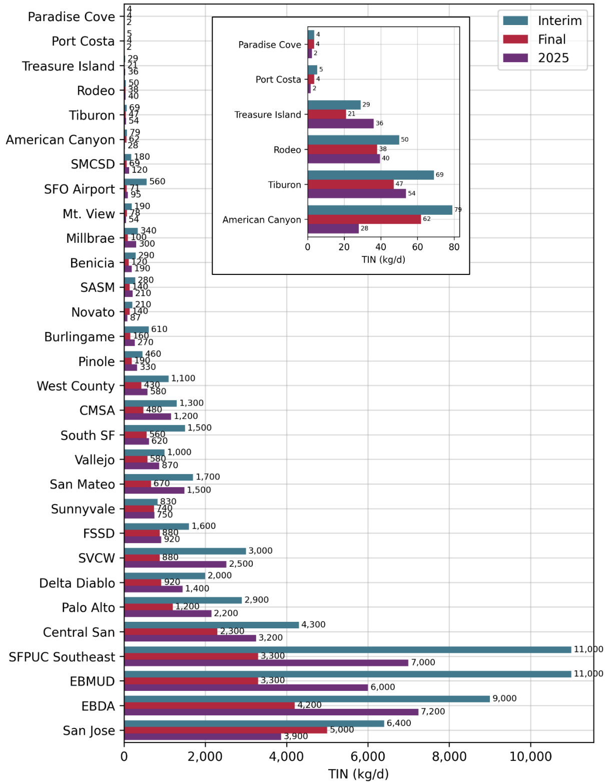
Figure 3-3. Individual Discharge Loads for 2025 Compared to the Dry Season TIN Limits (Interim and Final)
