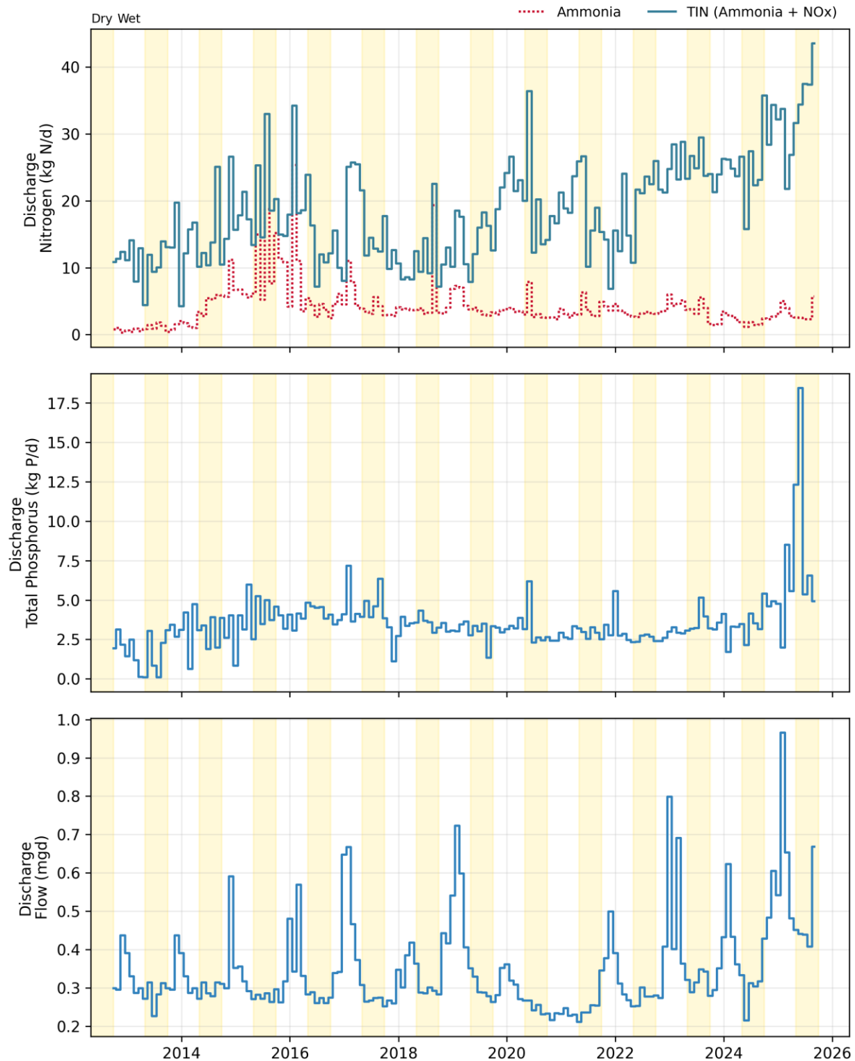
Figure 29-1. Discharge: Treasure Island Monthly Flows and Loads
