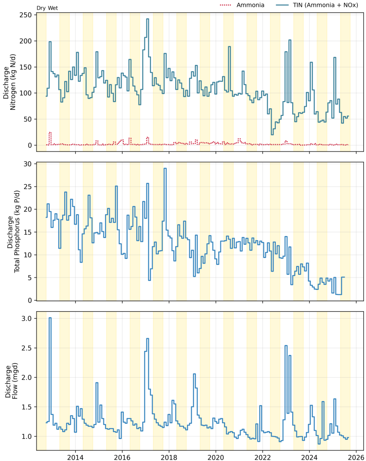
Figure 12-1. Discharge: Mt. View Sanitary District Monthly Flows and Loads
