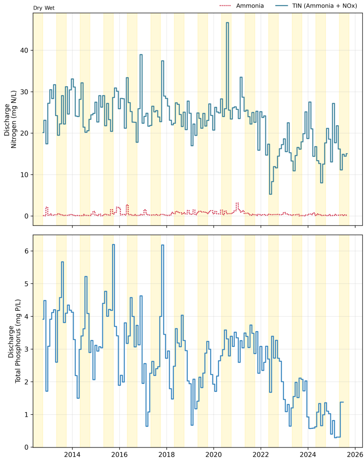
Figure 12-2. Discharge: Mt. View Sanitary District Monthly Concentrations
