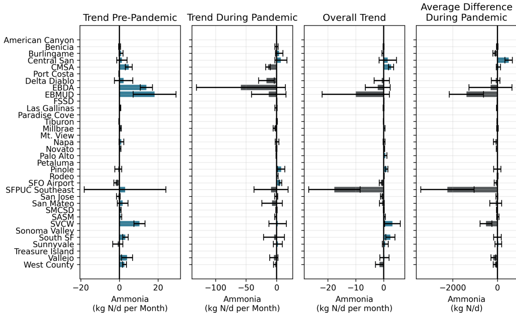
Figure B-4. Trend Coefficients for Ammonia (95% Confidence Interval Shown in Black).
