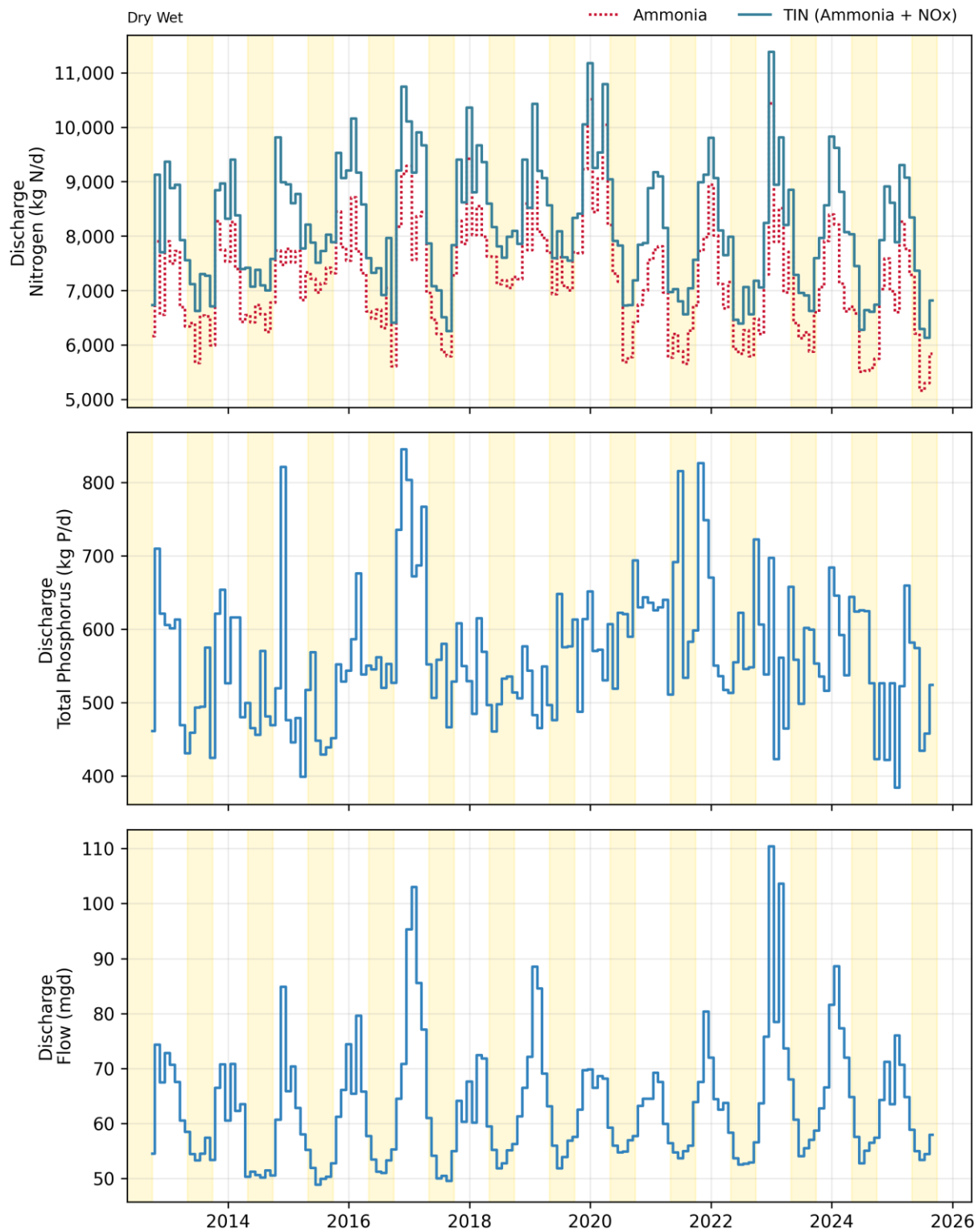
Figure 8-3. Discharge: EBDA Monthly Flows and Loads
