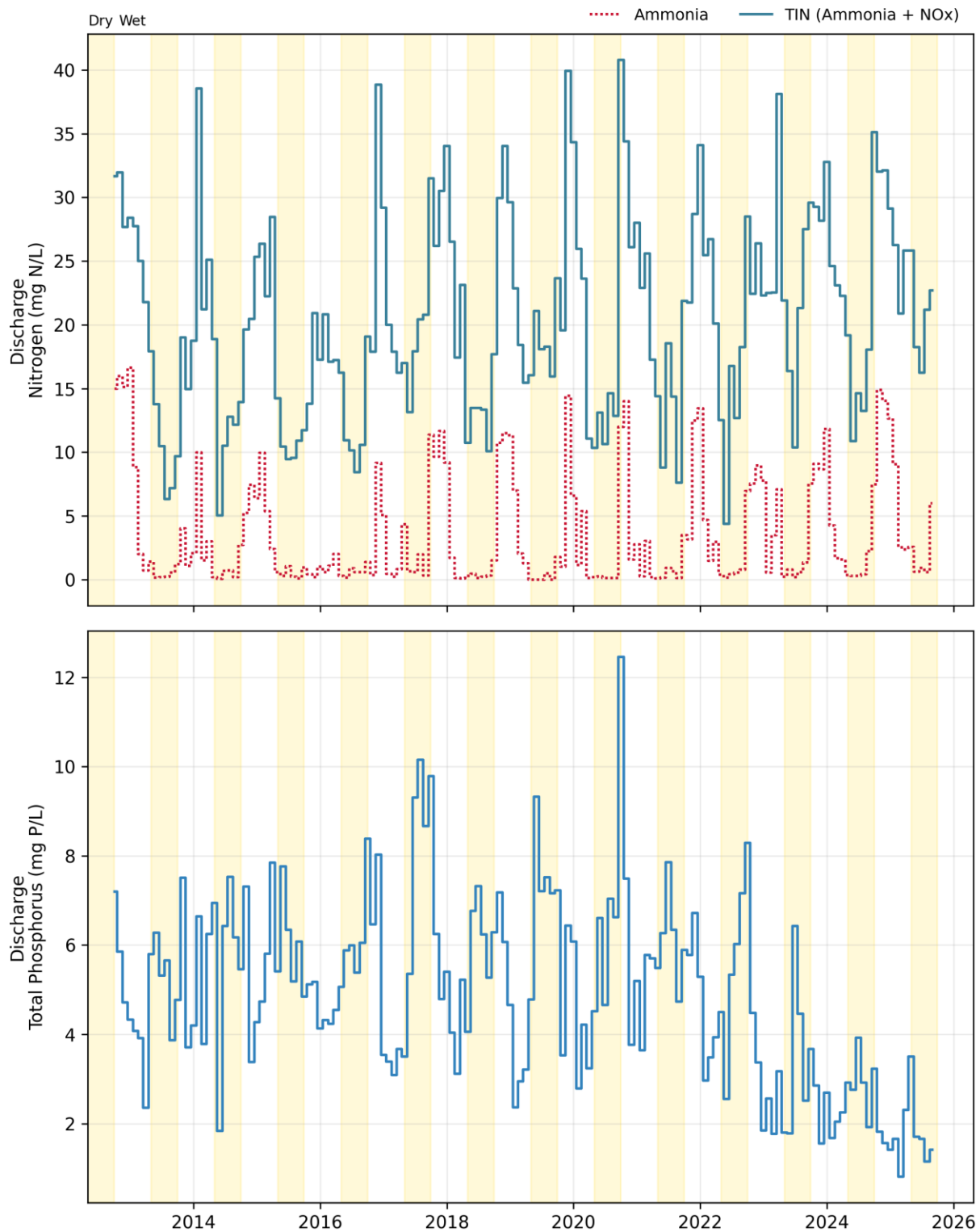
Figure 26-4. Discharge: Sunnyvale Monthly Concentrations
