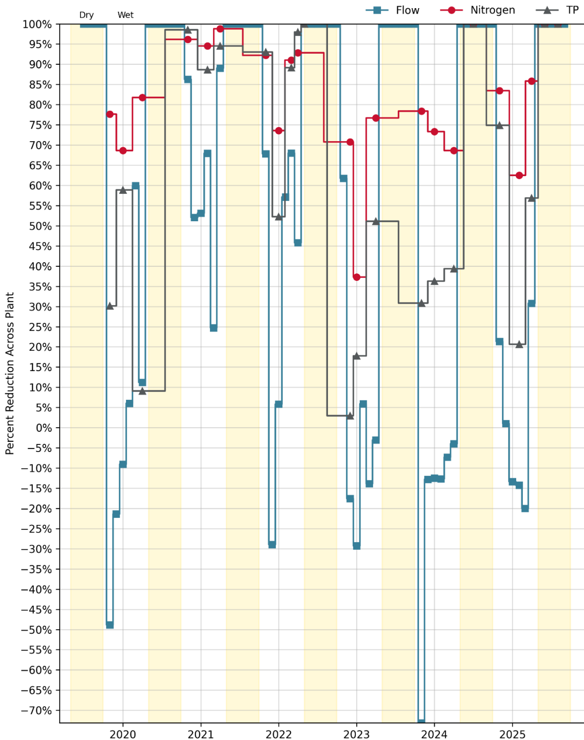
Figure 13-2. Influent: Napa Sanitation District Monthly Reductions Across the Plant*
