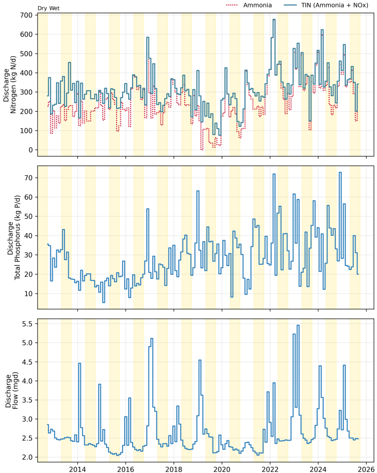
Figure 17-1. Discharge: Pinole Monthly Flows and Loads
