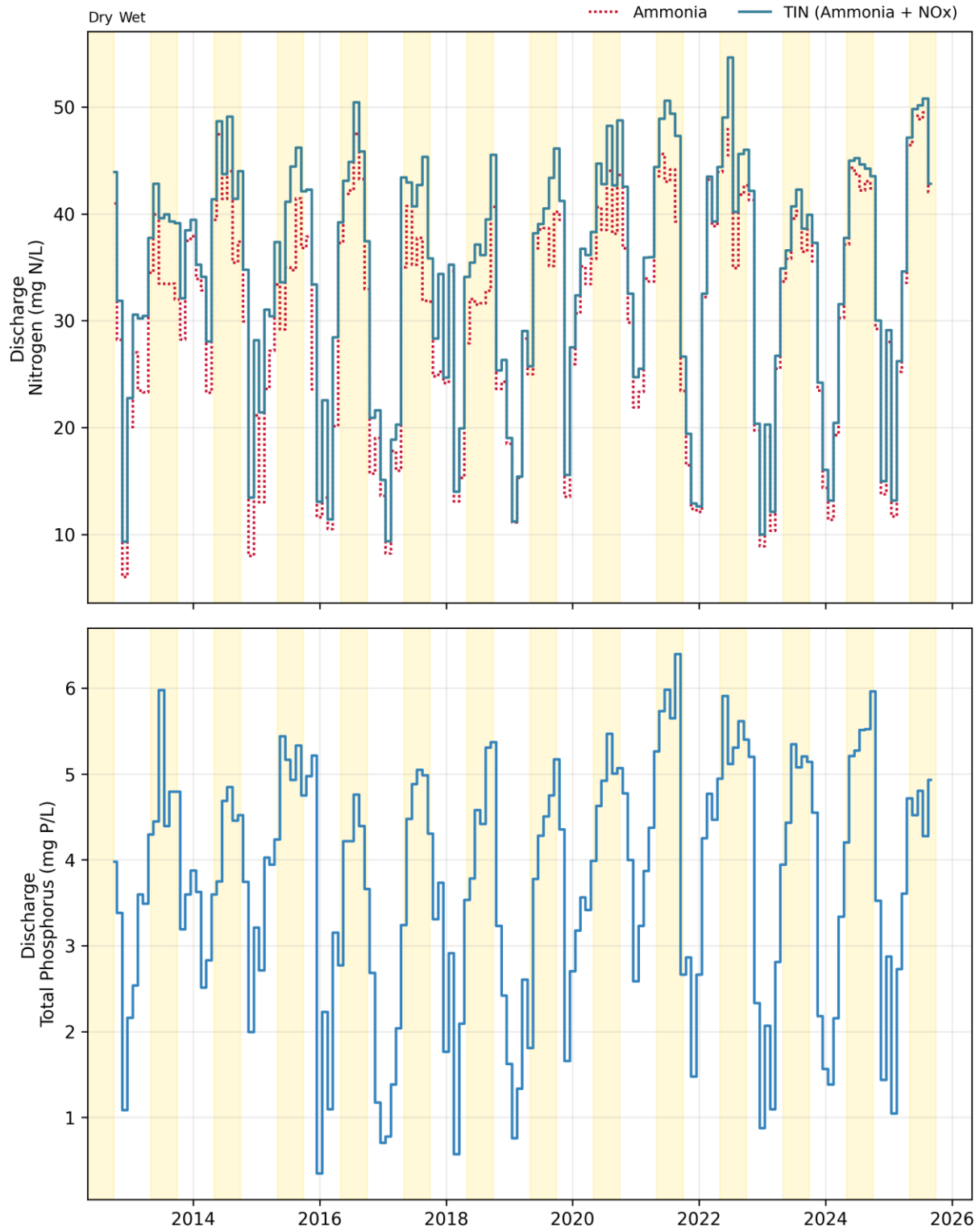
Figure 5-2. Discharge: CWSA Monthly Concentrations
