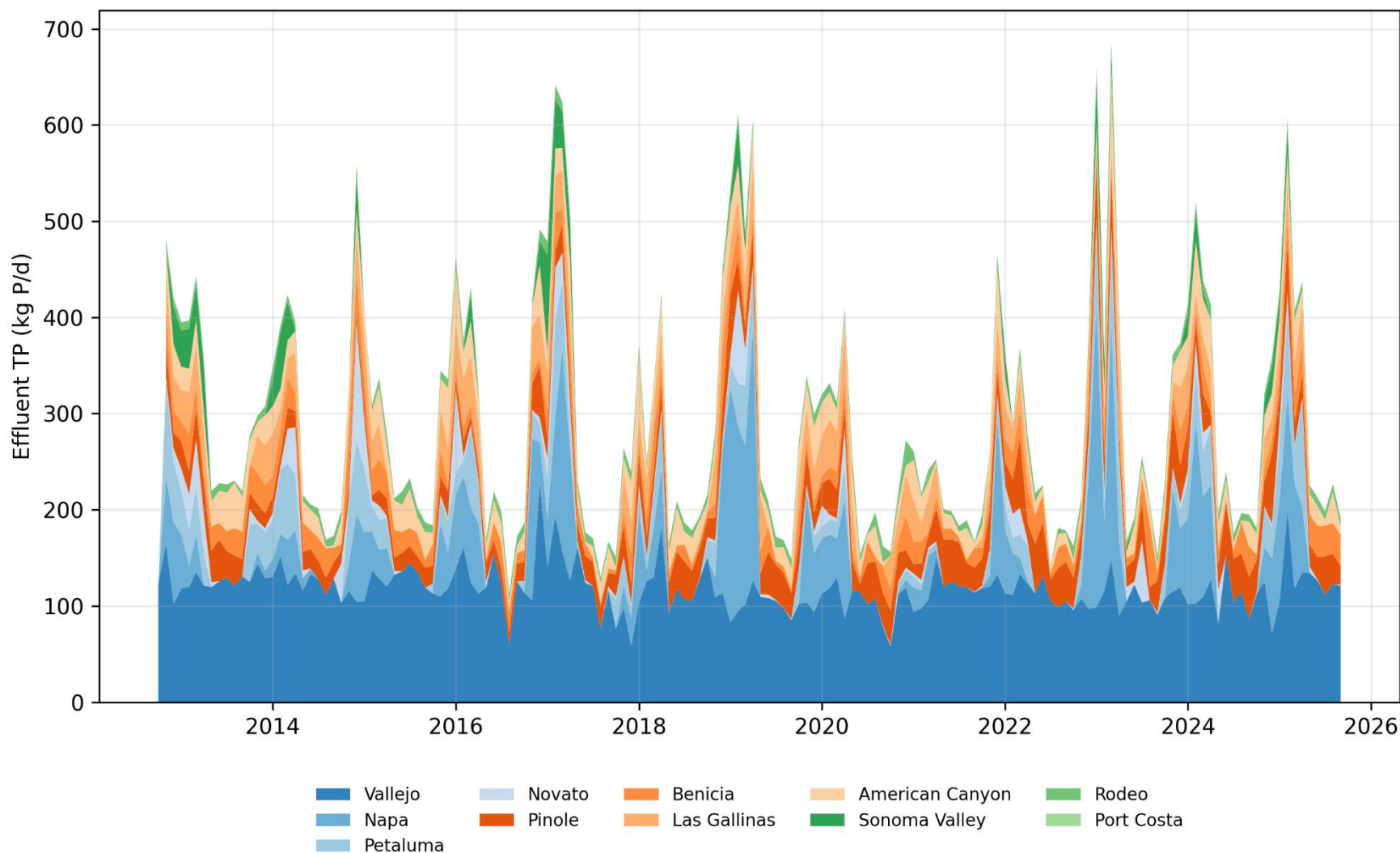
Figure C-10. TP Load Contribution by Discharger to San Pablo Bay
