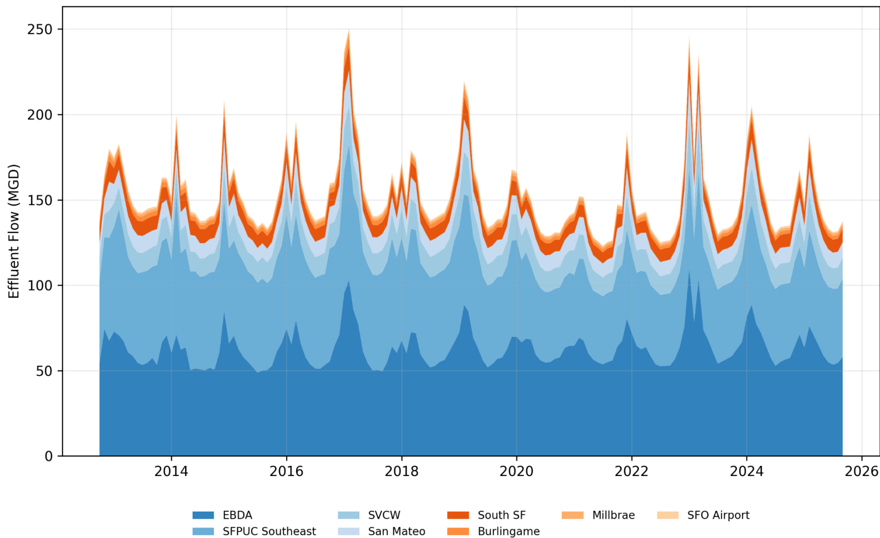
Figure C-16. Flow Contribution by Discharger to South Bay
