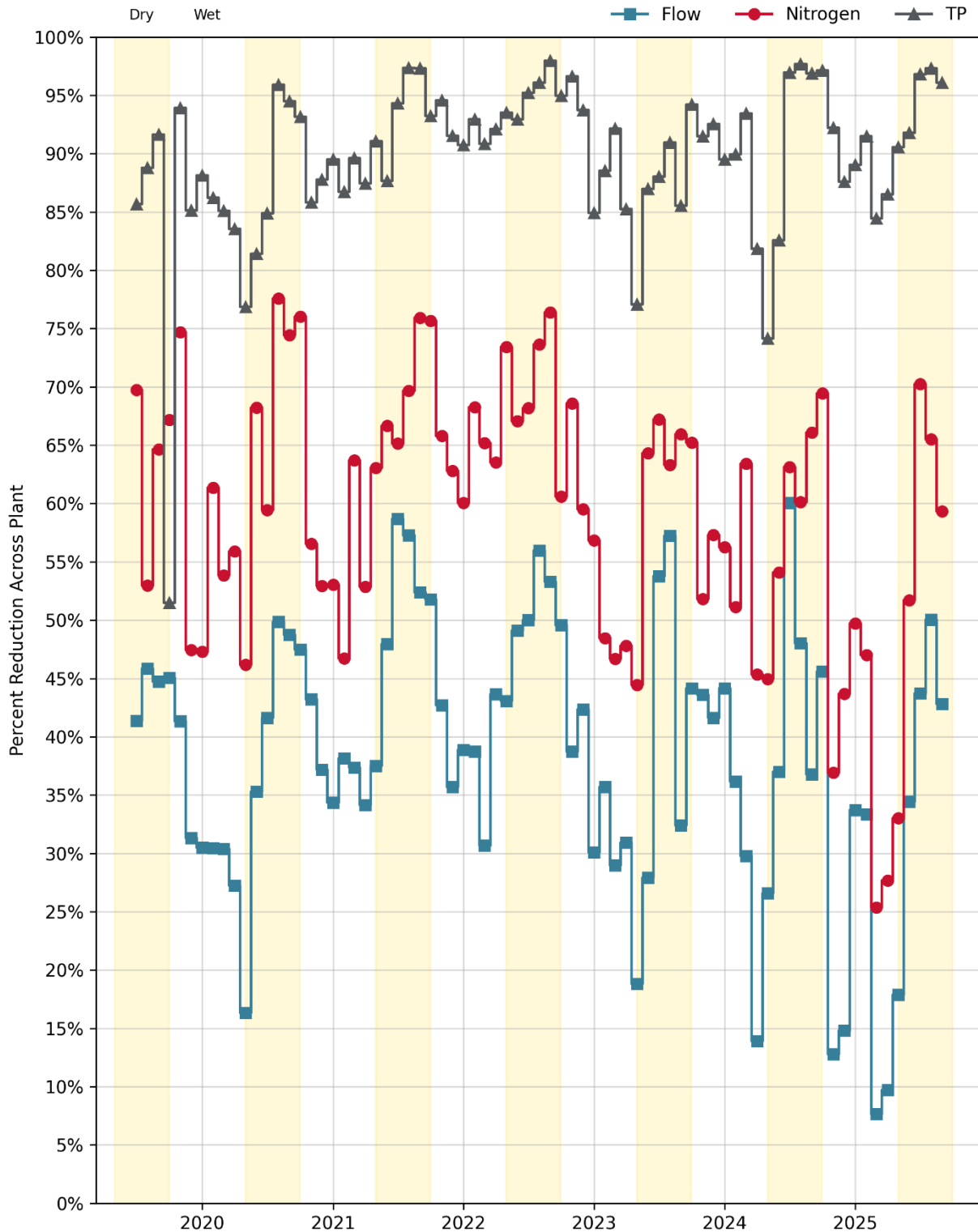
Figure 7-2. Influent: Delta Diablo Monthly Reductions Across the Plant
