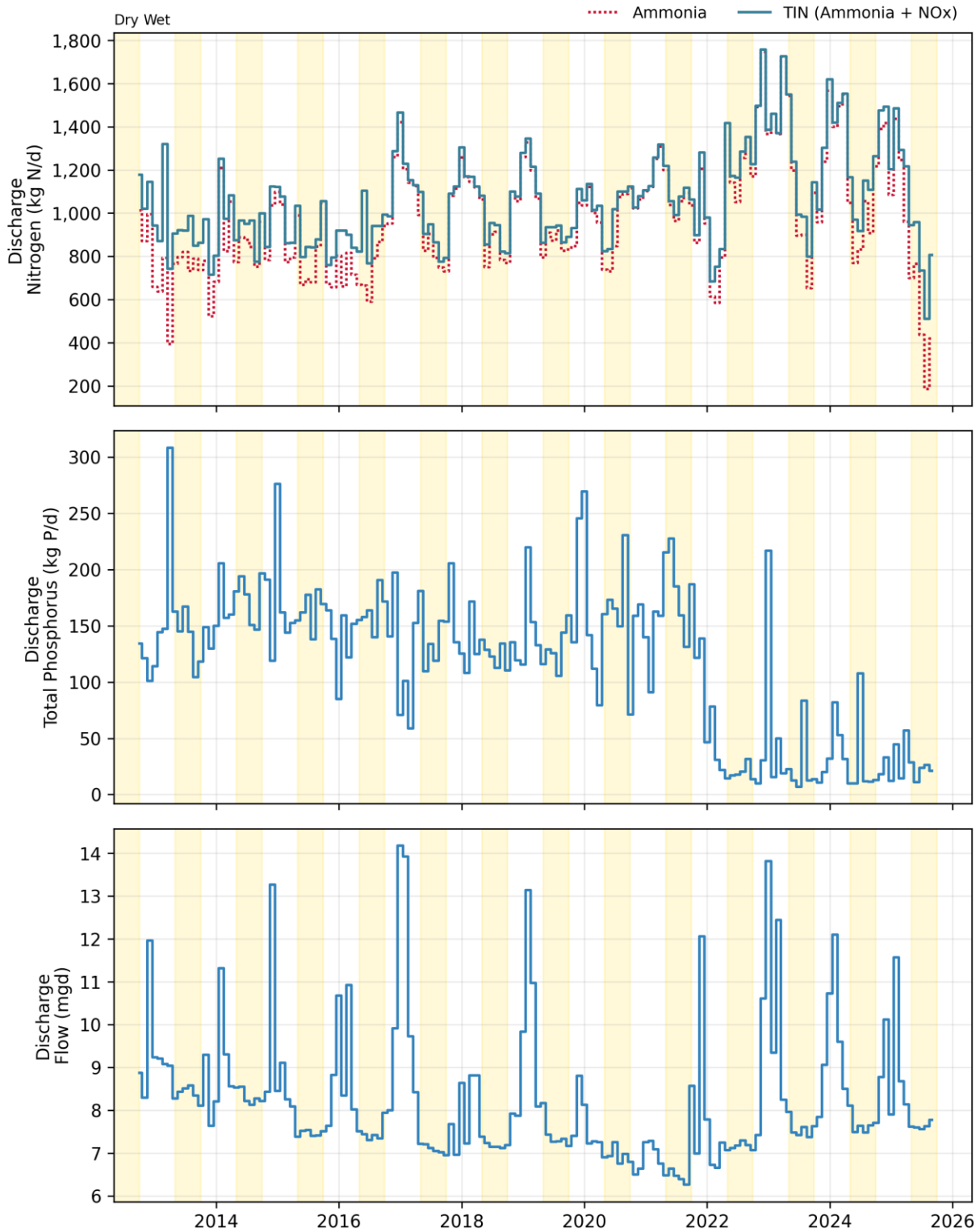
Figure 25-3. Discharge: South SF-San Bruno Monthly Flows and Loads
