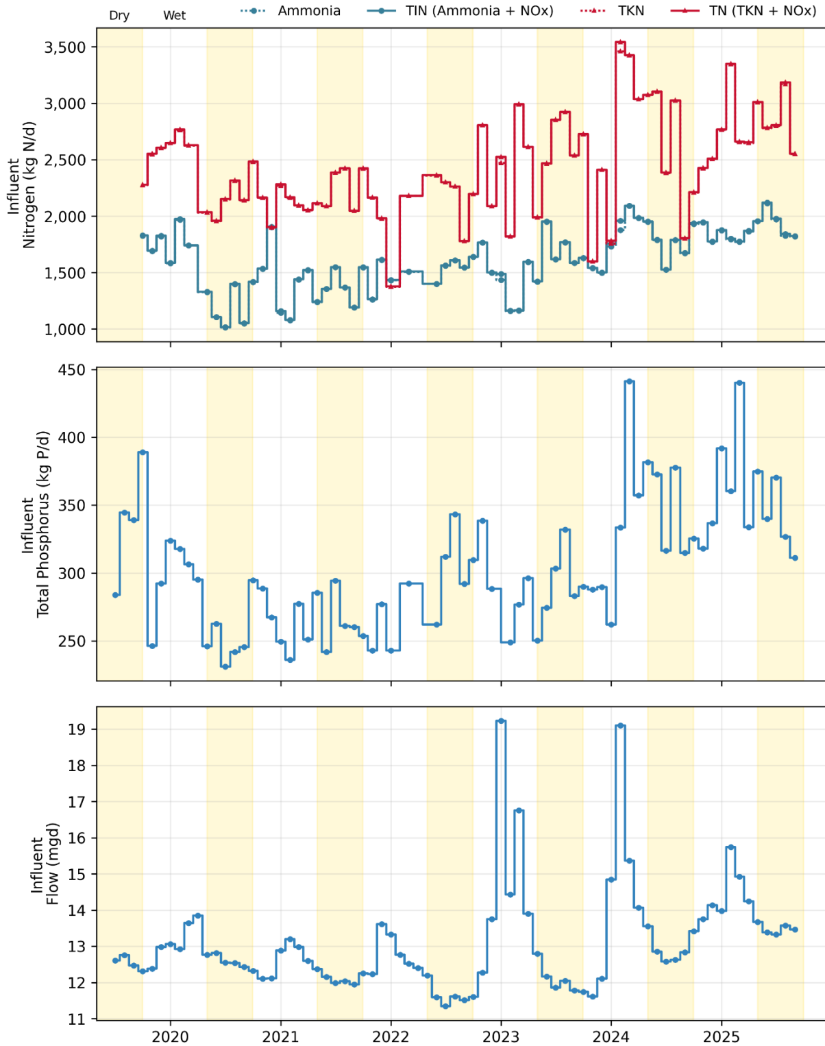
Figure 26-1. Influent: Sunnyvale Monthly Flows and Loads
