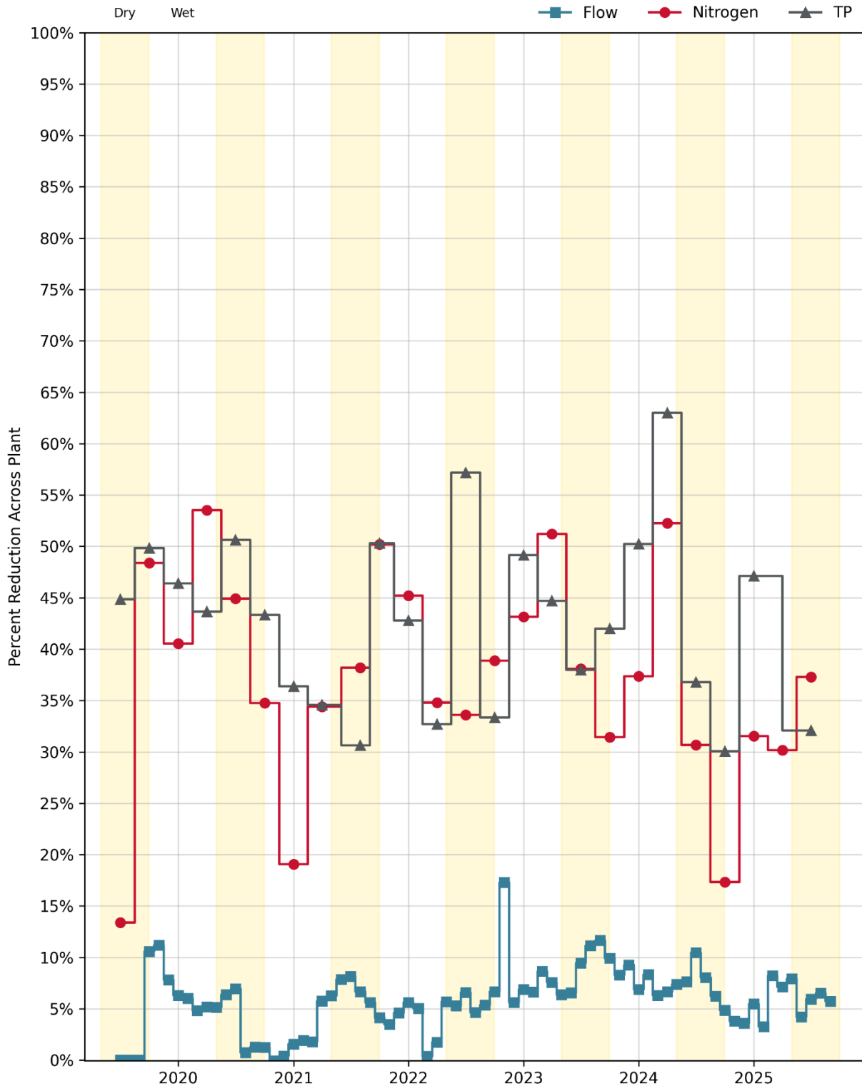
Figure 20-2. Influent: San Mateo Monthly Reductions Across the Plant
