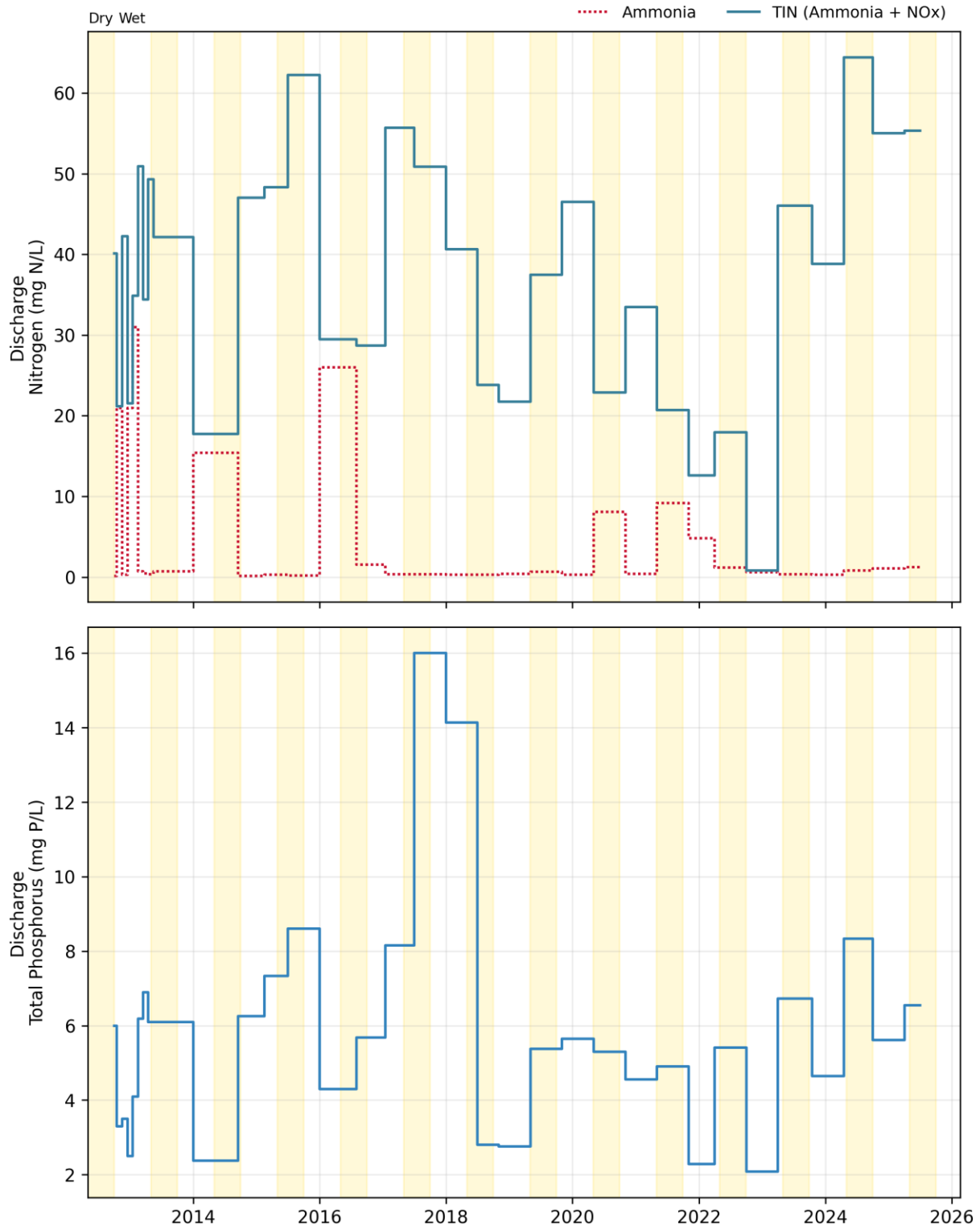
Figure 16-2. Discharge: Paradise Cove Monthly Concentrations
