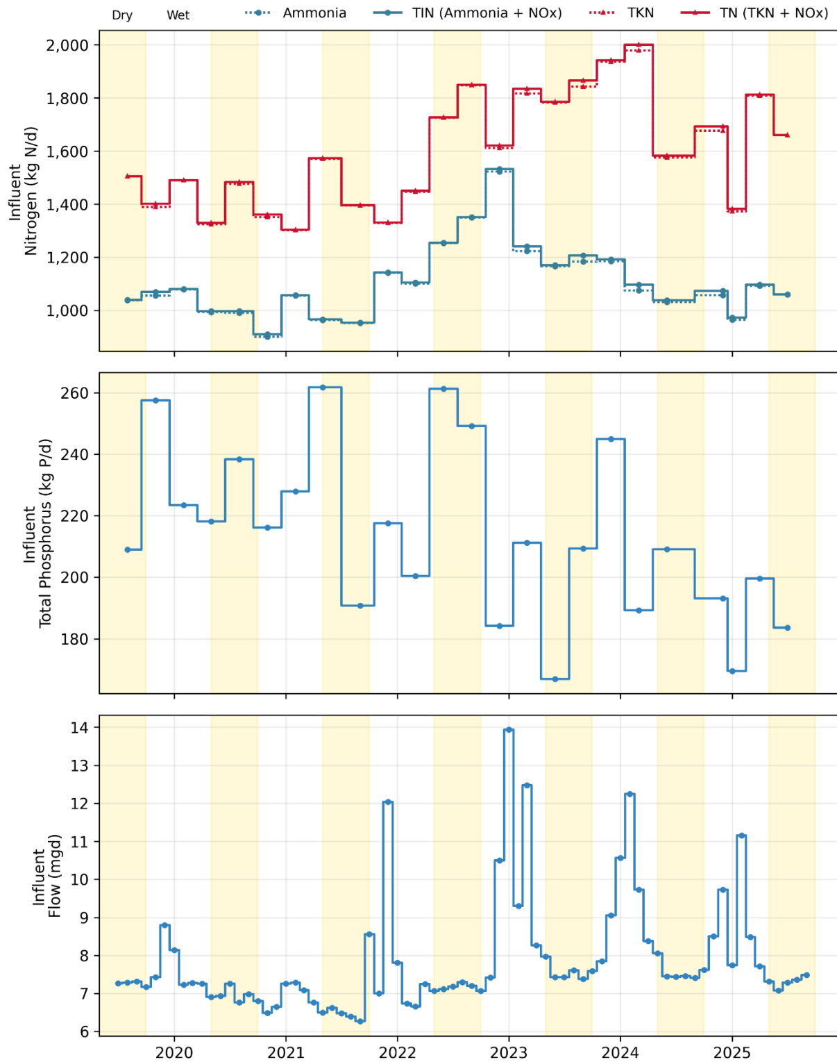
Figure 25-1. Influent: South SF-San Bruno Monthly Flows and Loads
