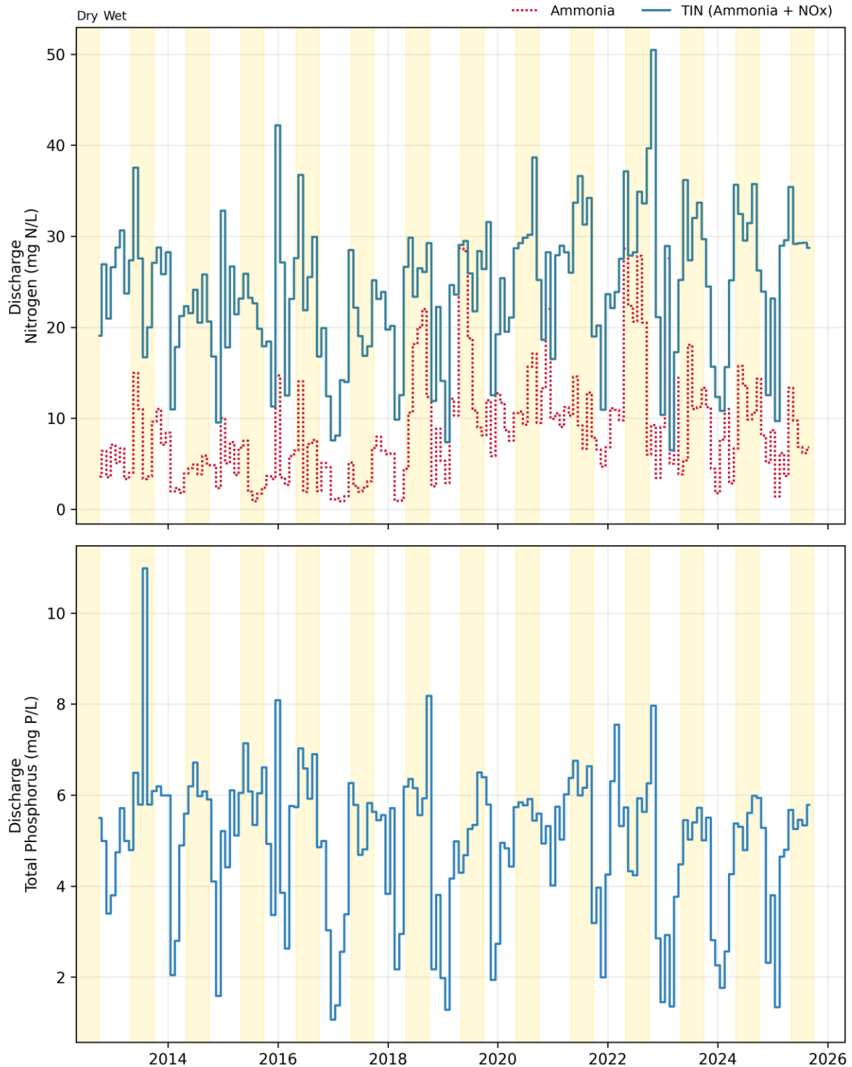
Figure 21-2. Discharge: SASM Monthly Concentrations
