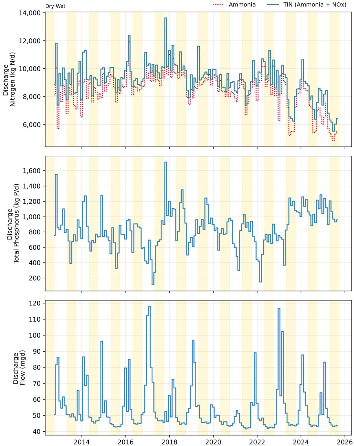
Figure 9-2. Discharge: EBMUD Monthly Flows and Loads
