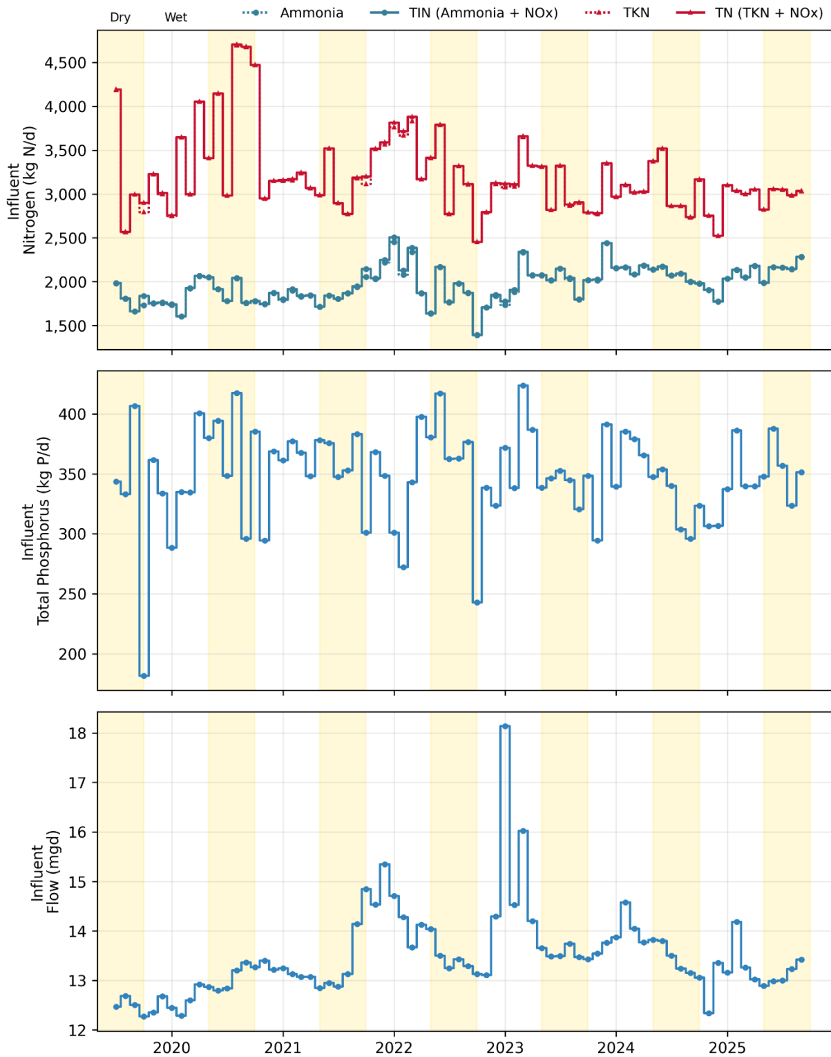
Figure 7-1. Influent: Delta Diablo Monthly Flows and Loads
