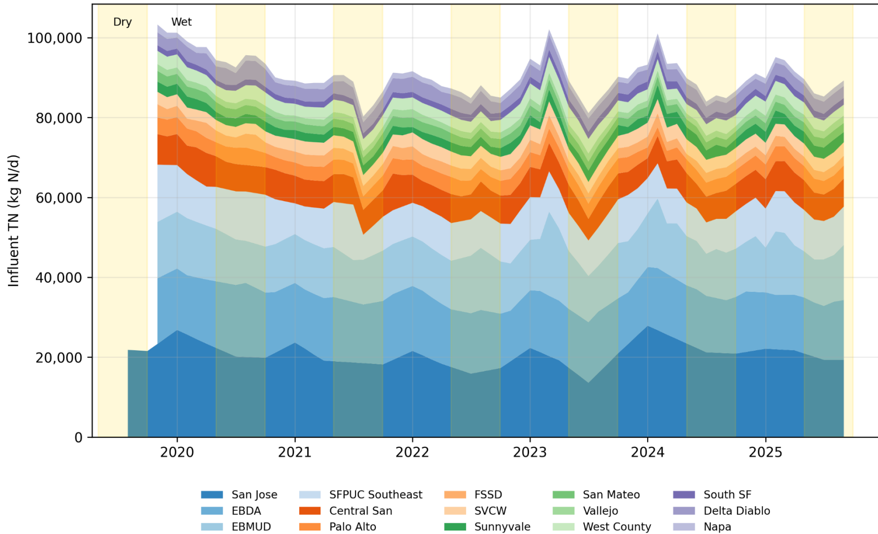
Figure A-6. Influent: Historical Average Quarterly TN Loads
