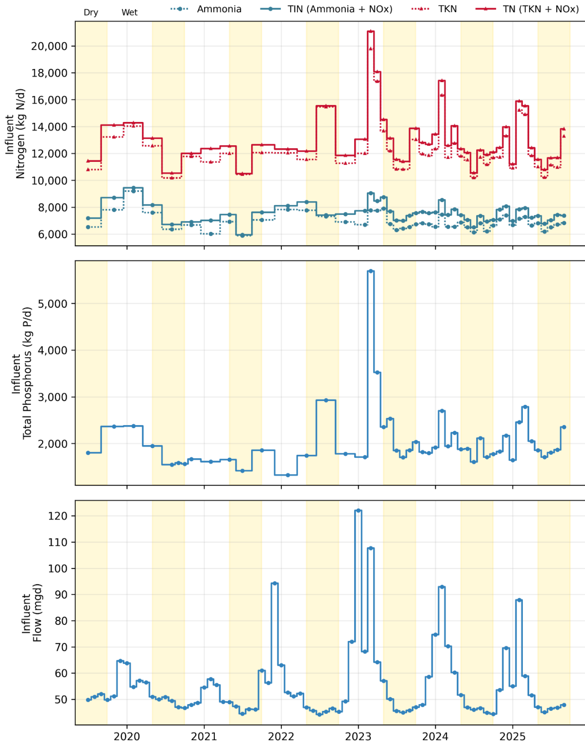
Figure 9-1. Influent: EBMUD Monthly Flows and Loads
