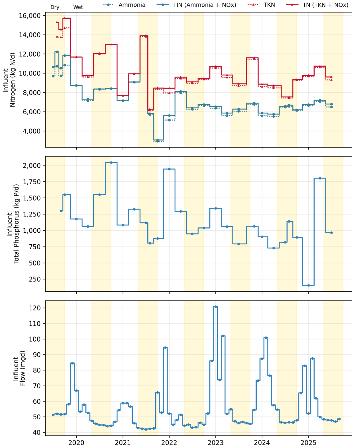
Figure 23-1. Influent: SFPUC Southeast Monthly Flows and Loads
