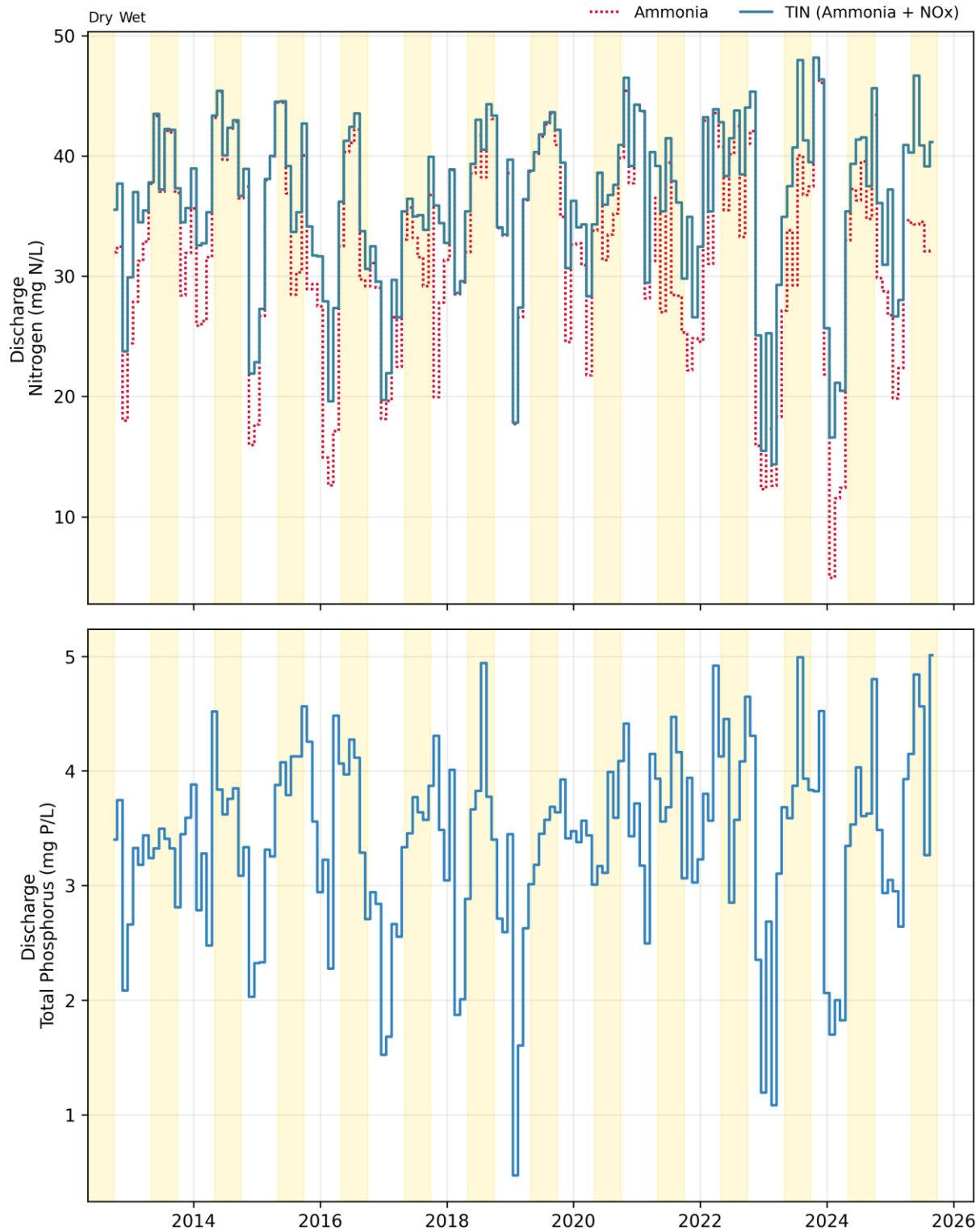
Figure 20-4. Discharge: San Mateo Monthly Concentrations
