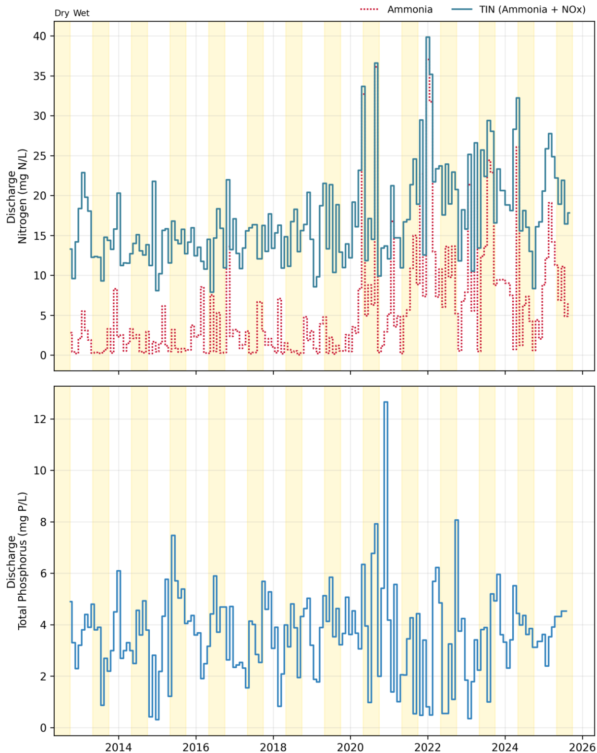
Figure 18-2. Discharge: Rodeo Monthly Concentrations
