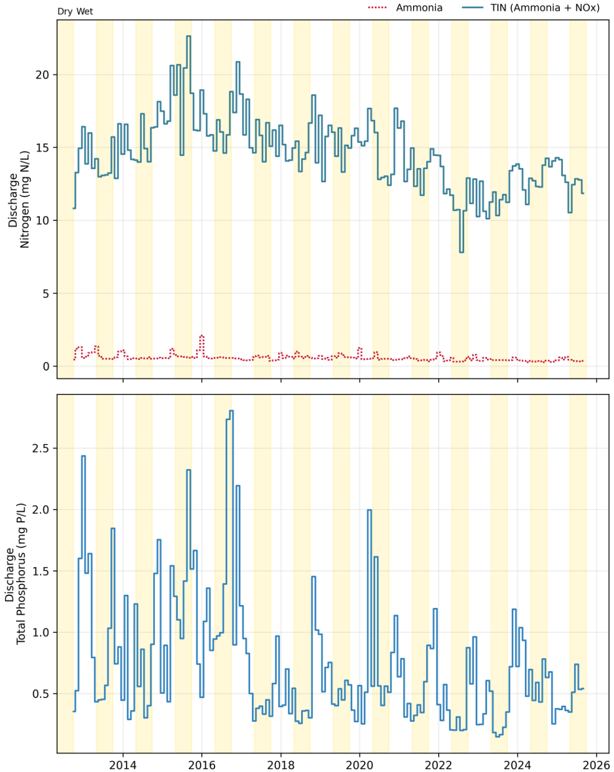
Figure 19-4. Discharge: San Jose Monthly Concentrations
