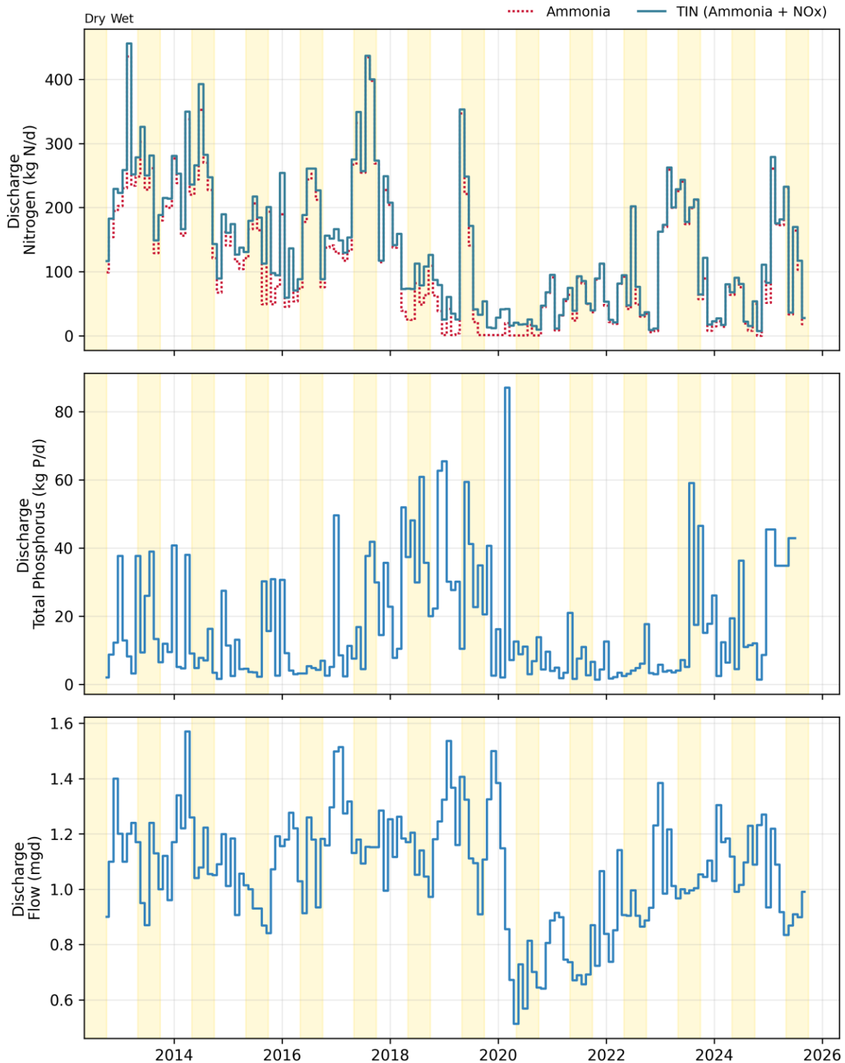
Figure 22-1. Discharge: SFO Airport Monthly Flows and Loads
