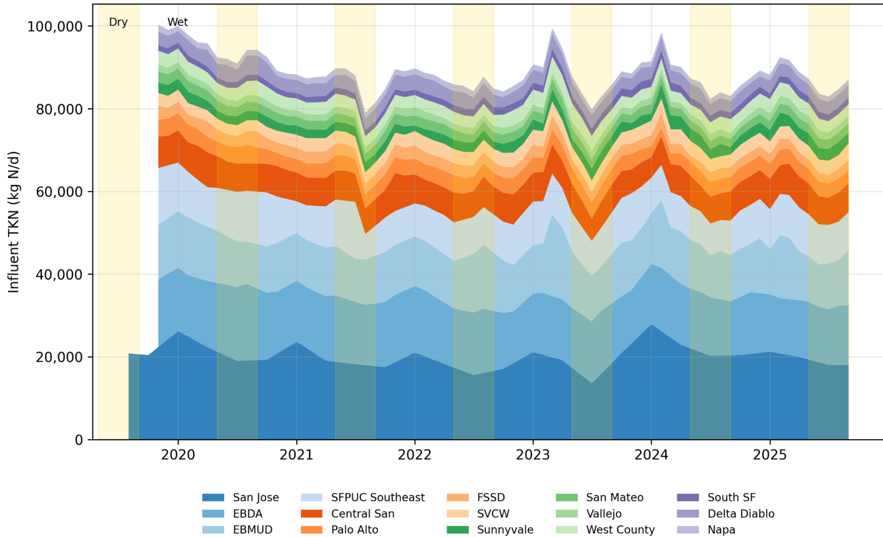
Figure A-5. Influent: Historical Average Quarterly TKN Loads
