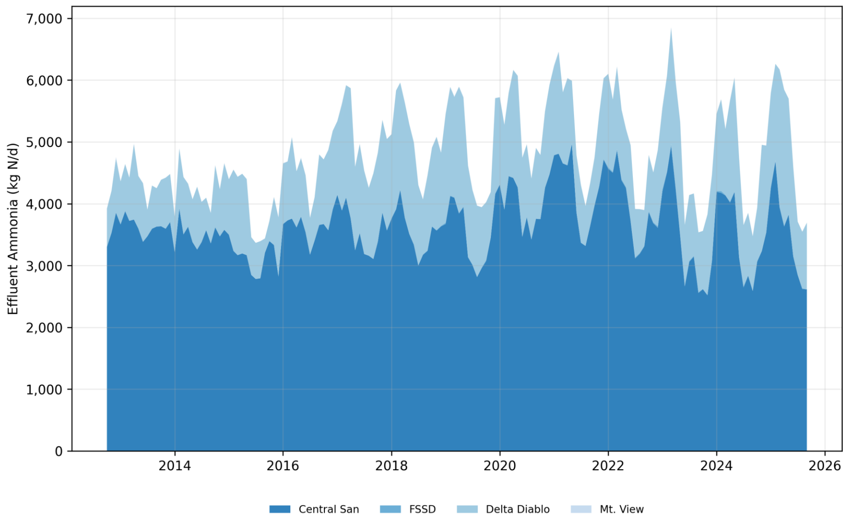
Figure C-2. Ammonia Load Contribution by Discharger to Suisun Bay
