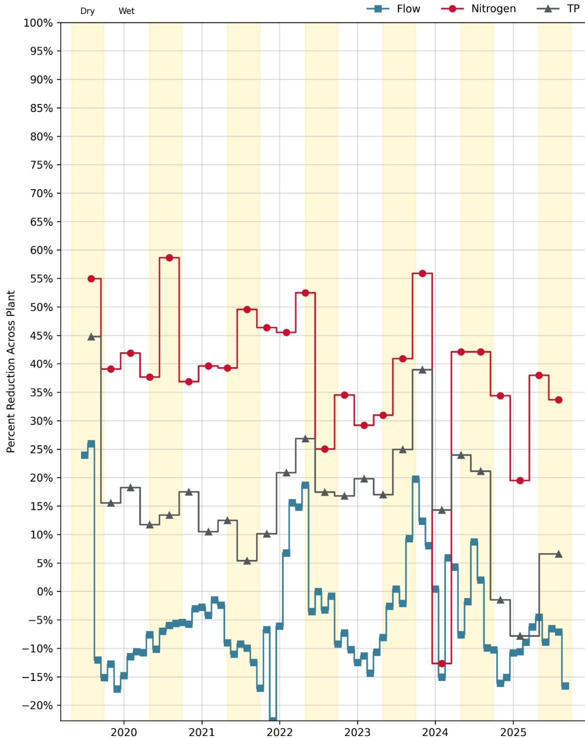
Figure 15-2. Influent: Palo Alto Monthly Reductions Across the Plant*
