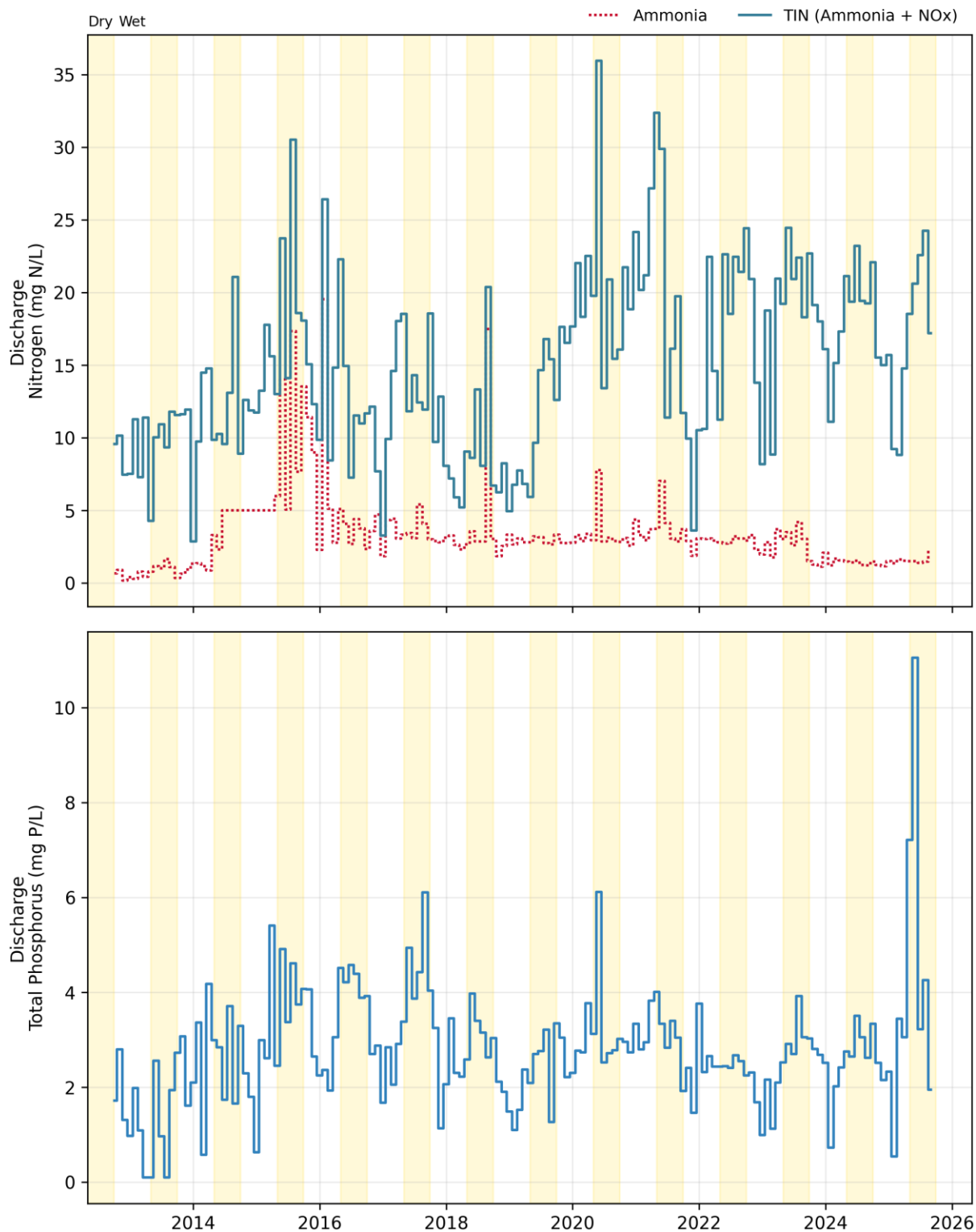
Figure 29-2. Discharge: Treasure Island Monthly Concentrations
