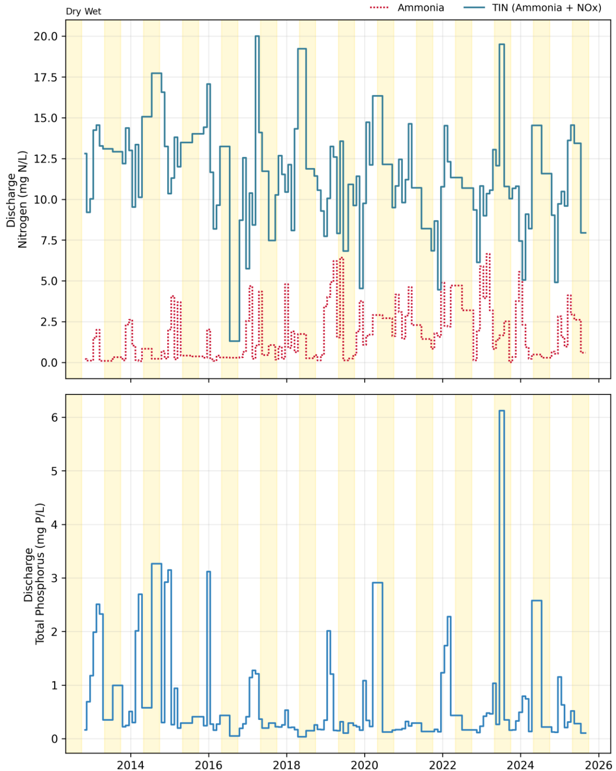
Figure 14-2. Discharge: Novato Monthly Concentrations
