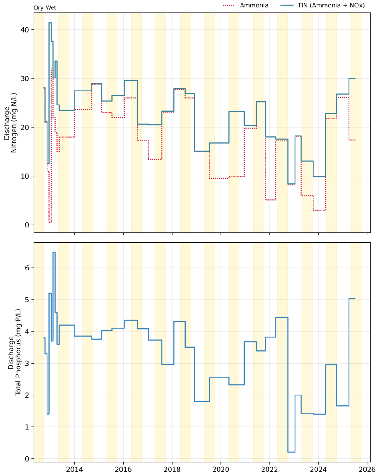
Figure 28-2. Discharge: Tiburon Monthly Concentrations
