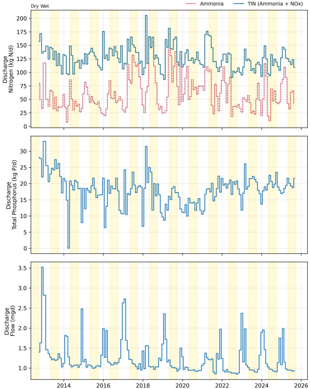
Figure 24-1. Discharge: SMCSD Monthly Flows and Loads
