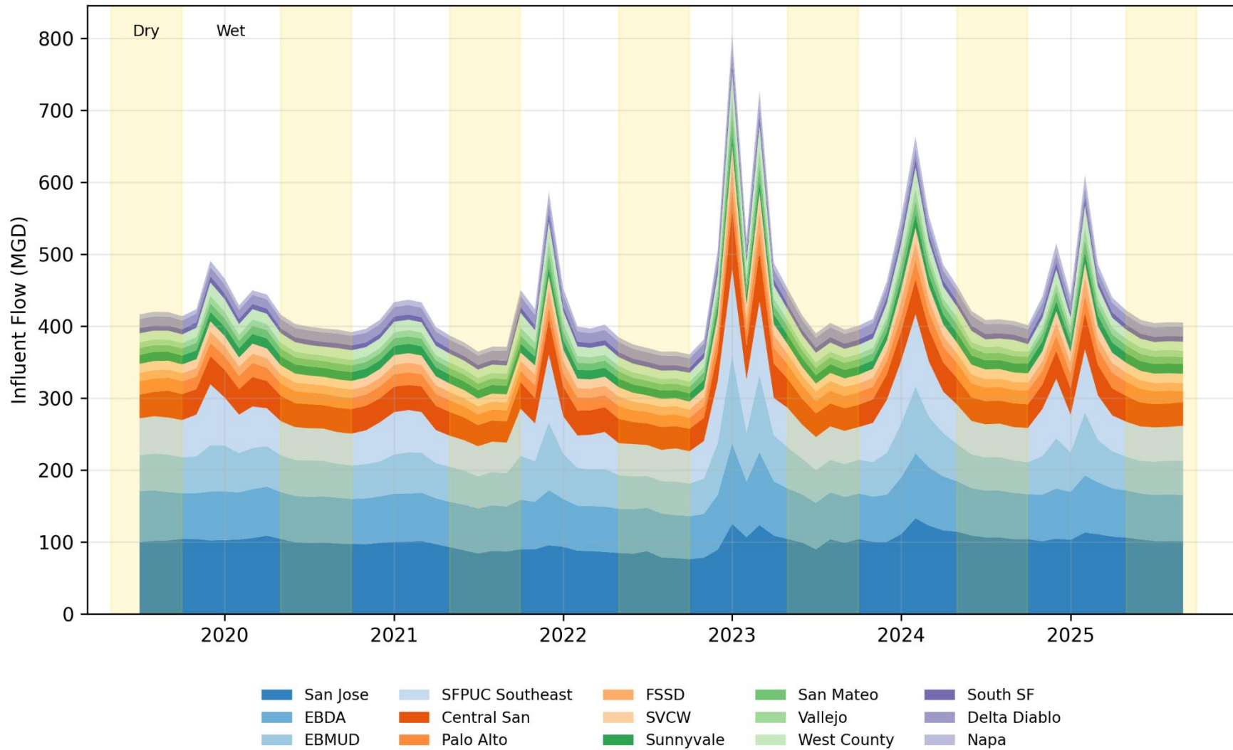
Figure A-1. Influent: Historical Average Quarterly Flow Values
