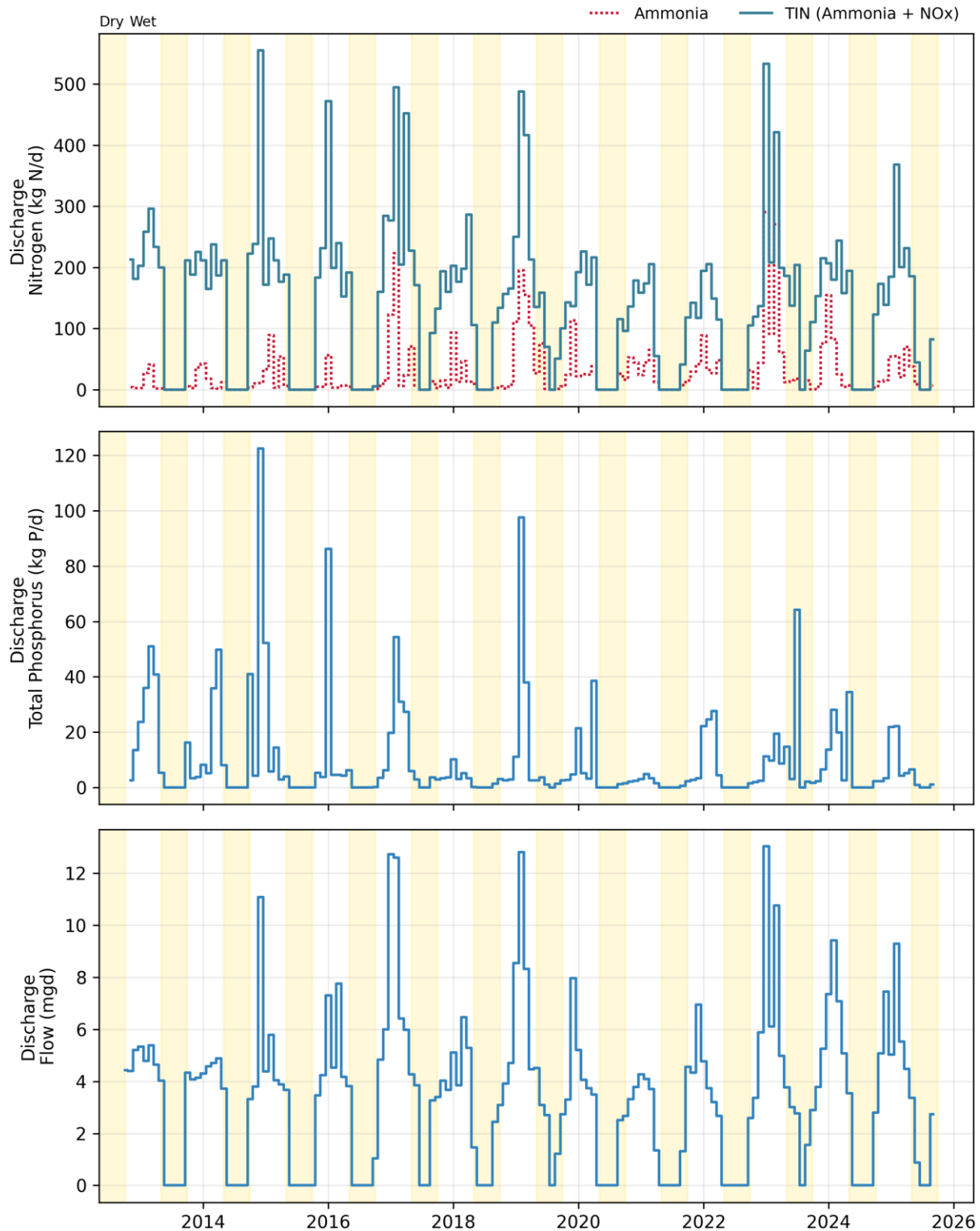
Figure 14-1. Discharge: Novato Monthly Flows and Loads
