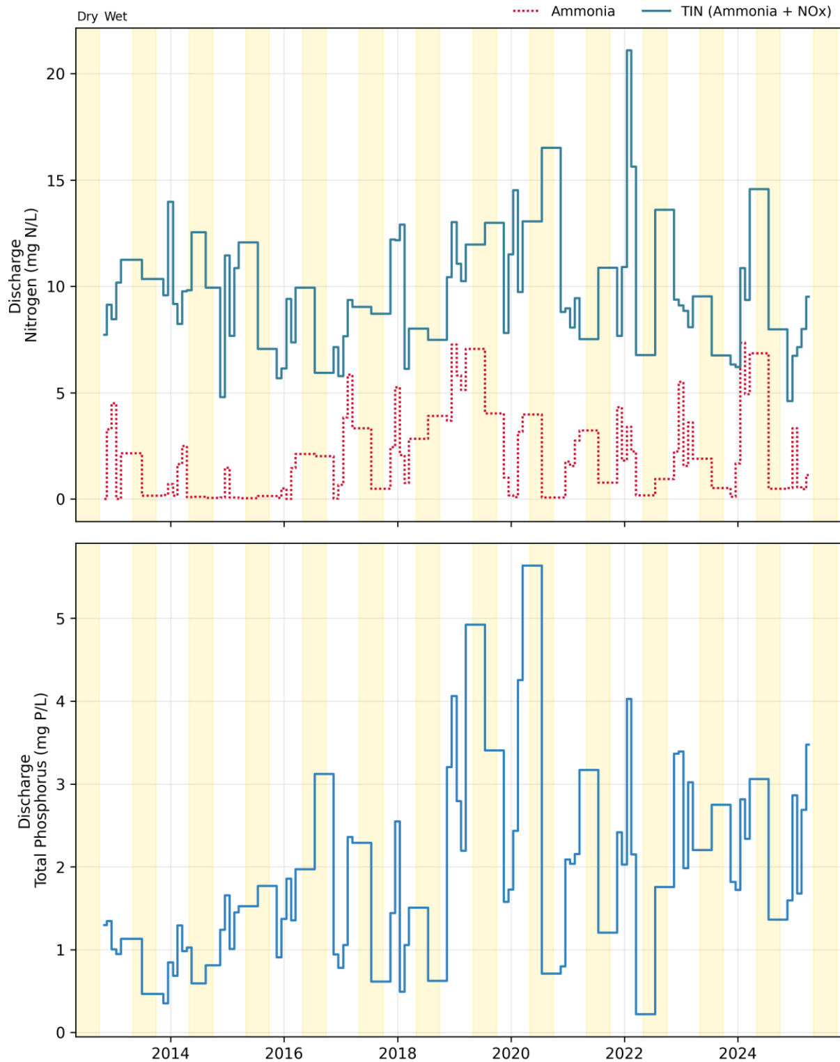
Figure 13-4. Discharge: Napa Sanitation District Monthly Concentrations
