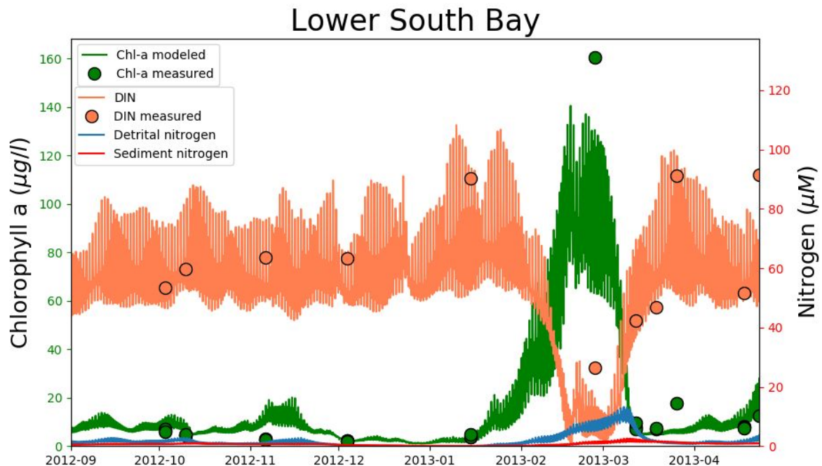
Figure 16 Measured and modeled concentrations of chlorophyll-a and DIN (nitrate (NO 3 ) + ammonium (NH 4 )) in Lower South Bay (LSB), September 2012-April 2013. Measured data is from samples collected during USGS cruises in Lower South Bay (combining s34 and s36). Modeled values are hourly data, predicted using the current version of the NMS' coupled hydrodynamic/biogeochemical model. The modeled concentrations are predictions for a fixed location in LSB (s36, Figure 1), and the large, high-frequency variations result from a combination of LSB's strong tides and spatial heterogeneity in water quality. Model output and observations suggest that the observed substantial DIN decrease beginning mid-February resulted from a major phytoplankton bloom
