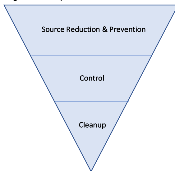
Fig. 3. Hierarchy of Efforts to Address Ocean Litter
