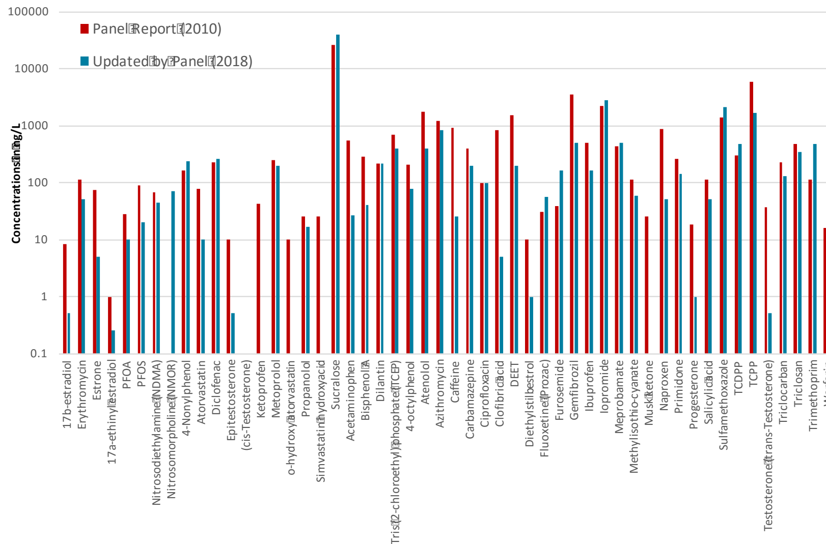
Figure 4.1. Comparison of 90 th percentile measured environmental concentrations (MECs) reported in secondary/tertiary treated effluents compiled during the 2010 and 2018 Panel reviews (concentrations in ng/L).
