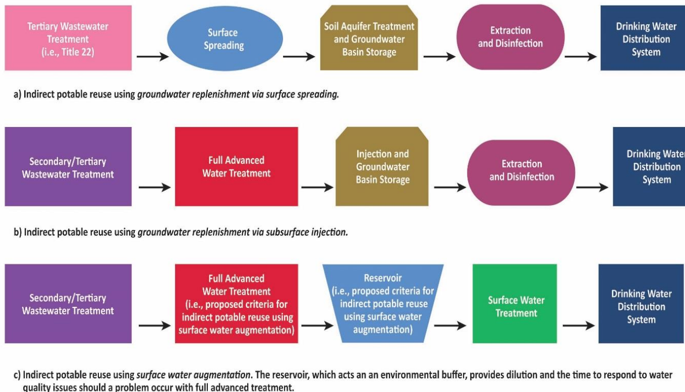
Figure 3.2. Schematics of (a,b) indirect potable reuse in California using groundwater replenishment and (c) surface water reservoir augmentation (per revised CWC, SWRCB 2017b). The environmental buffer is represented by a groundwater aquifer in (a) and (b), and by a reservoir in (c). Wastewater treatment could include either secondary or tertiary treatment. Tertiary treated wastewater per Title 22 involves well-oxidized, filtered, and disinfected wastewater. Soil-aquifer treatment involves the percolation of water through the vadose zone, which provides soil treatment. In California, full advanced treatment per Title 22 requires reverse osmosis and an oxidation treatment process. Drinking water treatment for surface water meets California drinking water standards (Olivieri et al., 2016).
