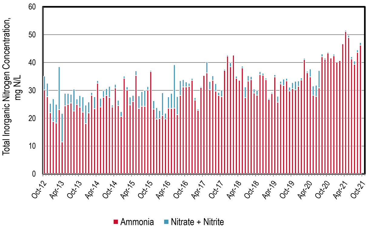
Figure 28-5. Discharge: South SF-San Bruno Monthly Nitrogen Concentrations
