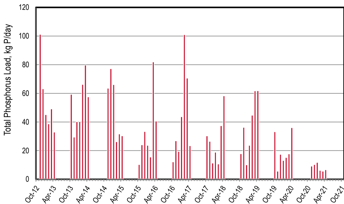
Figure 18-4. Discharge: Petaluma Monthly Phosphorus Loads
