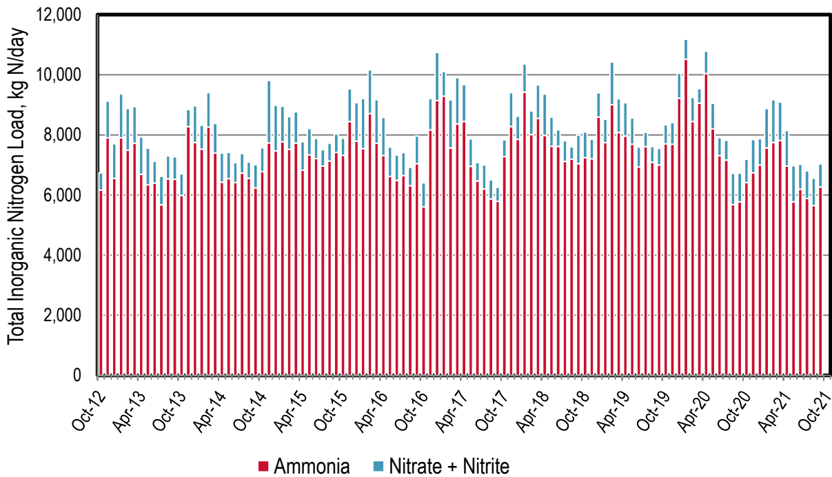
Figure 8-4. Discharge: EBDA Monthly Nitrogen Loads
