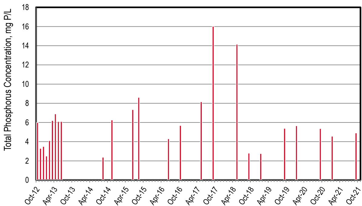
Figure 17-5. Discharge: Paradise Cove Monthly Phosphorus Concentrations
