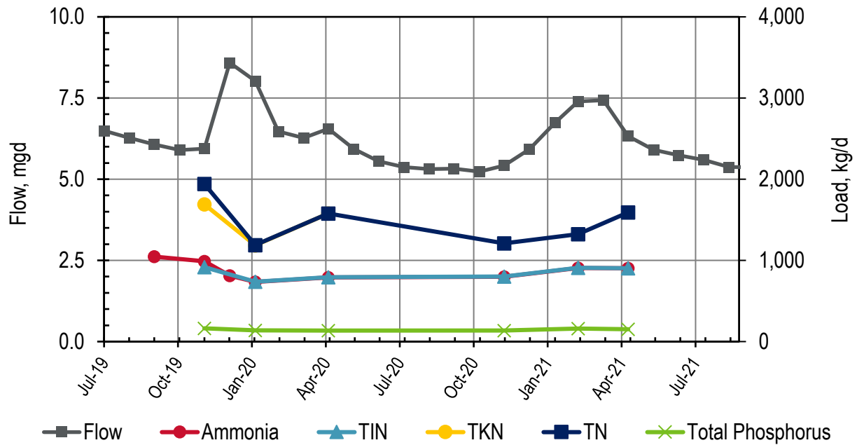
Figure 14-1. Influent: Napa Sanitation District Monthly Flows and Loads
