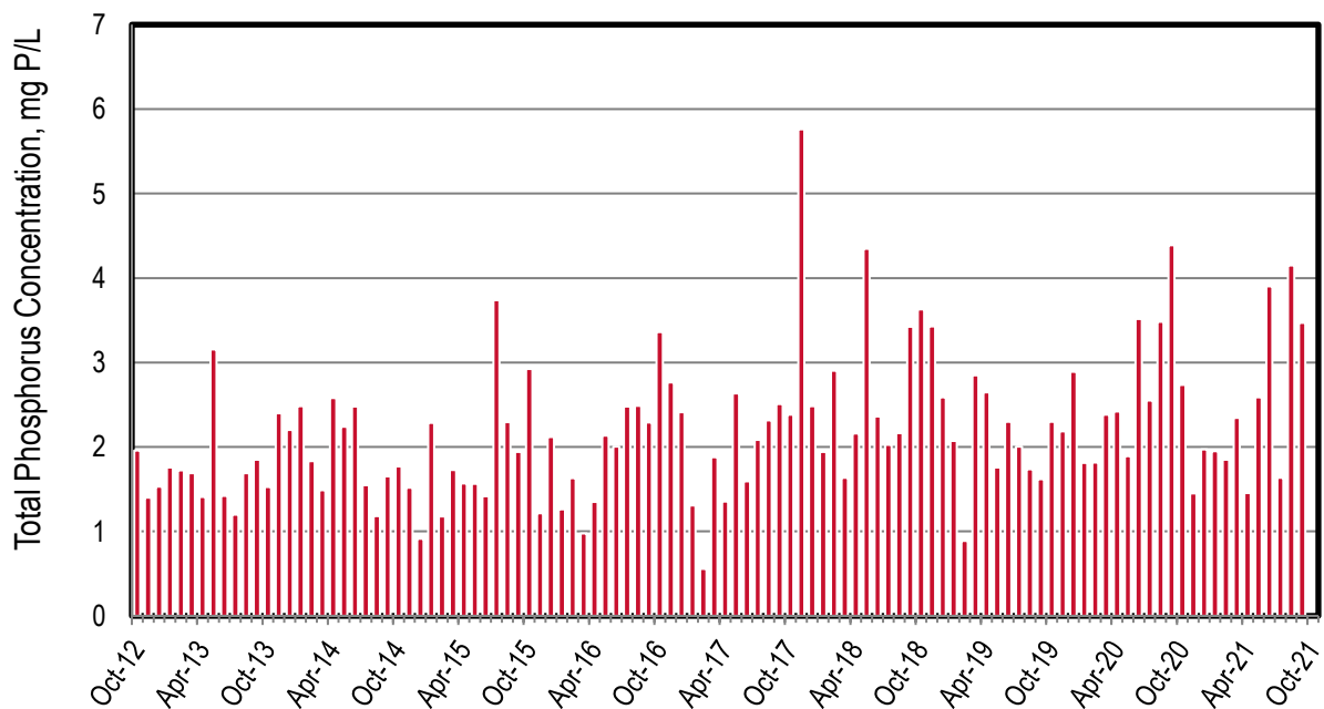
Figure 34-7. Discharge: West County Monthly Phosphorus Concentrations
