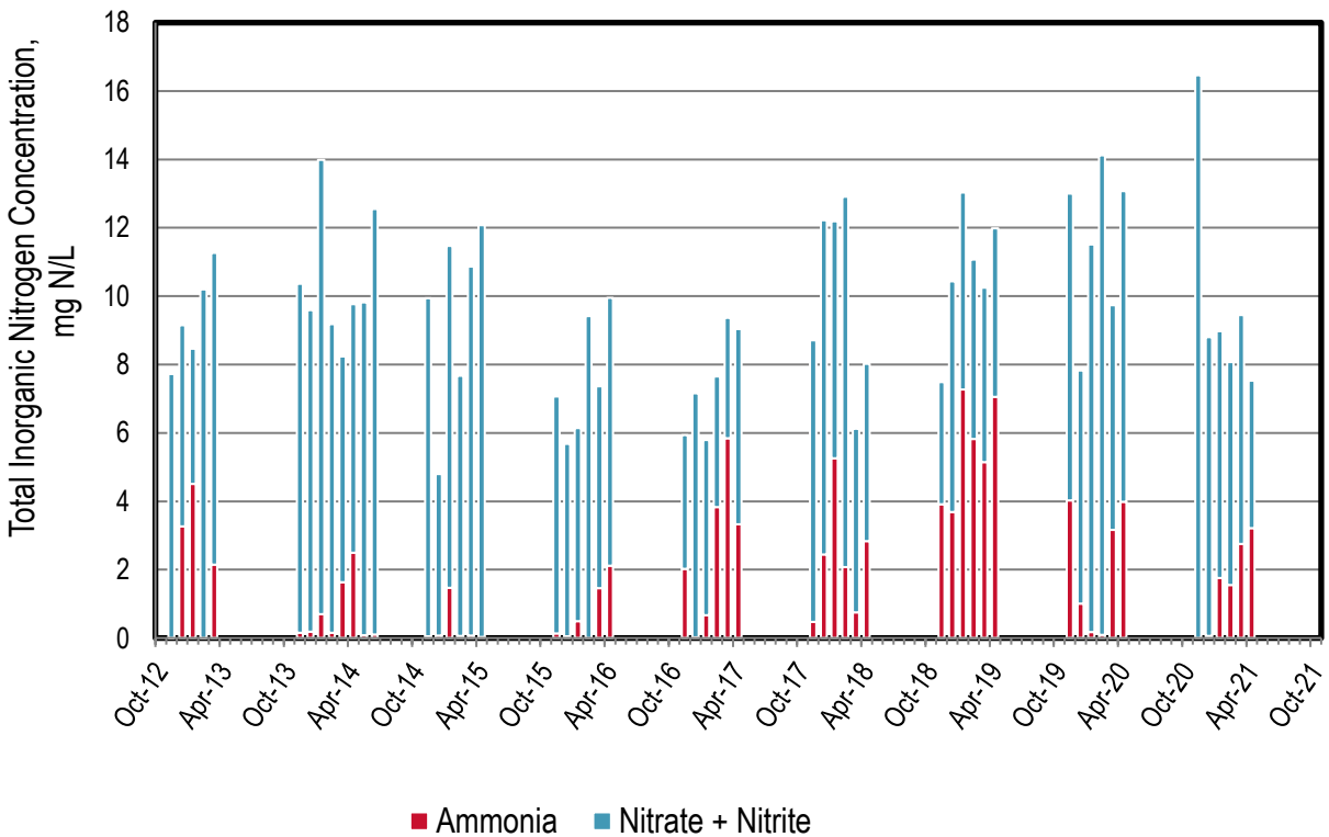
Figure 14-5. Discharge: Napa Sanitation District Monthly Nitrogen Concentrations
