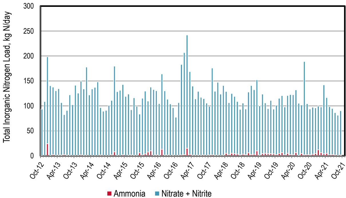
Figure 13-2. Discharge: Mt. View Sanitary District Monthly Nitrogen Loads
