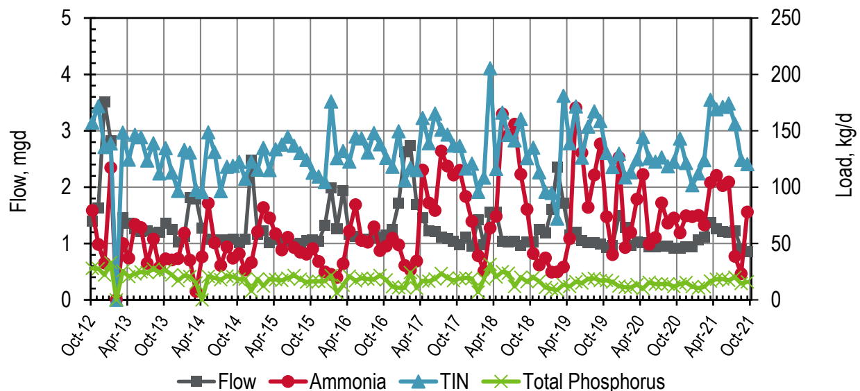
Figure 26-1. Discharge: SMCSD Monthly Flows and Loads
