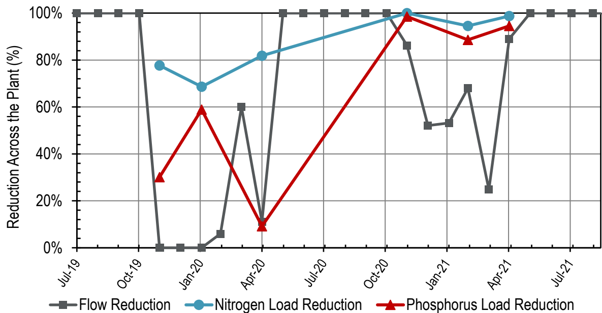
Figure 14-2. Influent: Napa Sanitation District Monthly Reductions Across the Plant
