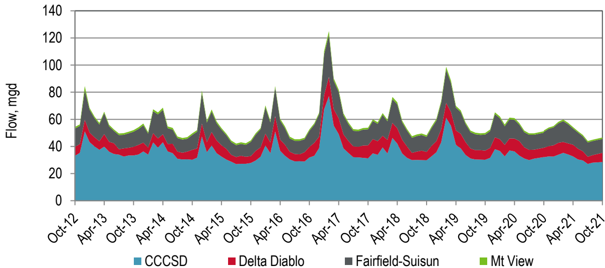
Figure 5-6. Flow Contribution by Discharger to Suisun Bay
