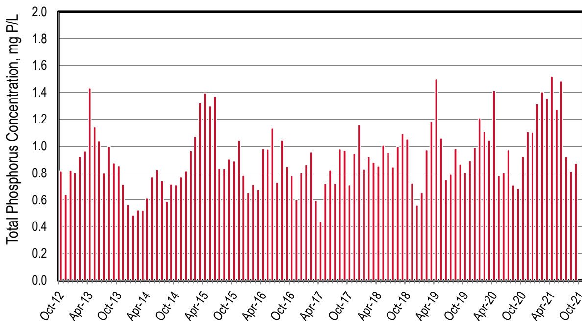
Figure 4-7. Discharge: Central San Monthly Phosphorus Concentrations
