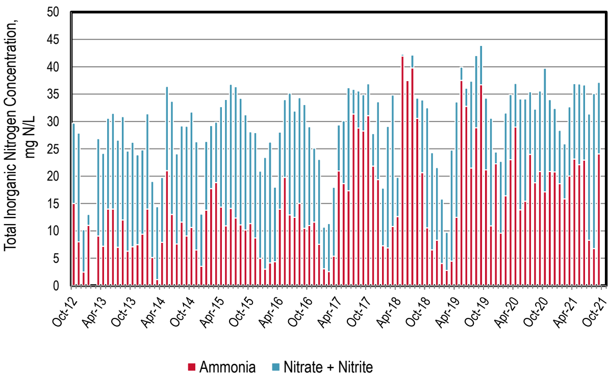
Figure 26-3. Discharge: SMCS Monthly Nitrogen Concentrations
