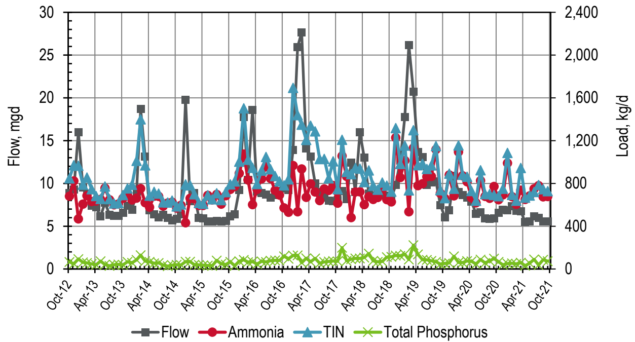
Figure 34-3. Discharge: West County Monthly Flows and Loads
