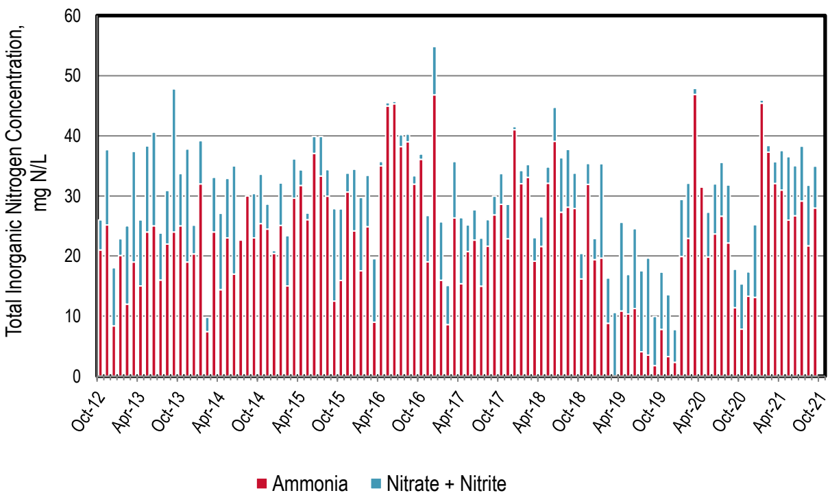
Figure 19-3. Discharge: Pinole Monthly Nitrogen Concentrations
