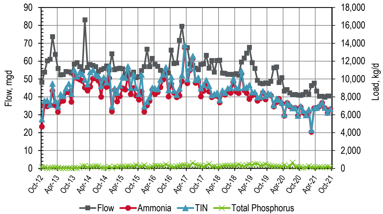
Figure 25-2. Discharge: SFPUC Southeast Monthly Flows and Loads
