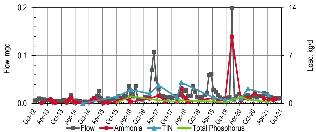
Figure 6-1. Discharge: Port Costa Monthly Flows and Loads
