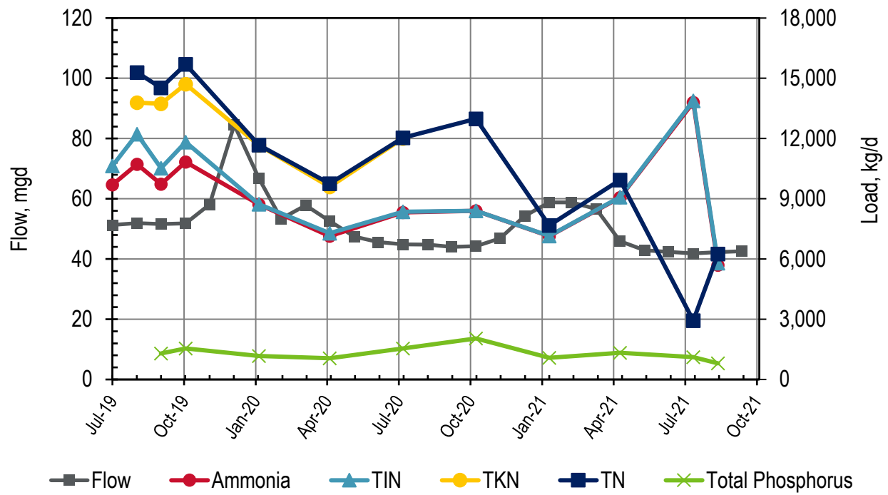
Figure 25-1. Influent: SFPUC Southeast Monthly Flows and Loads
