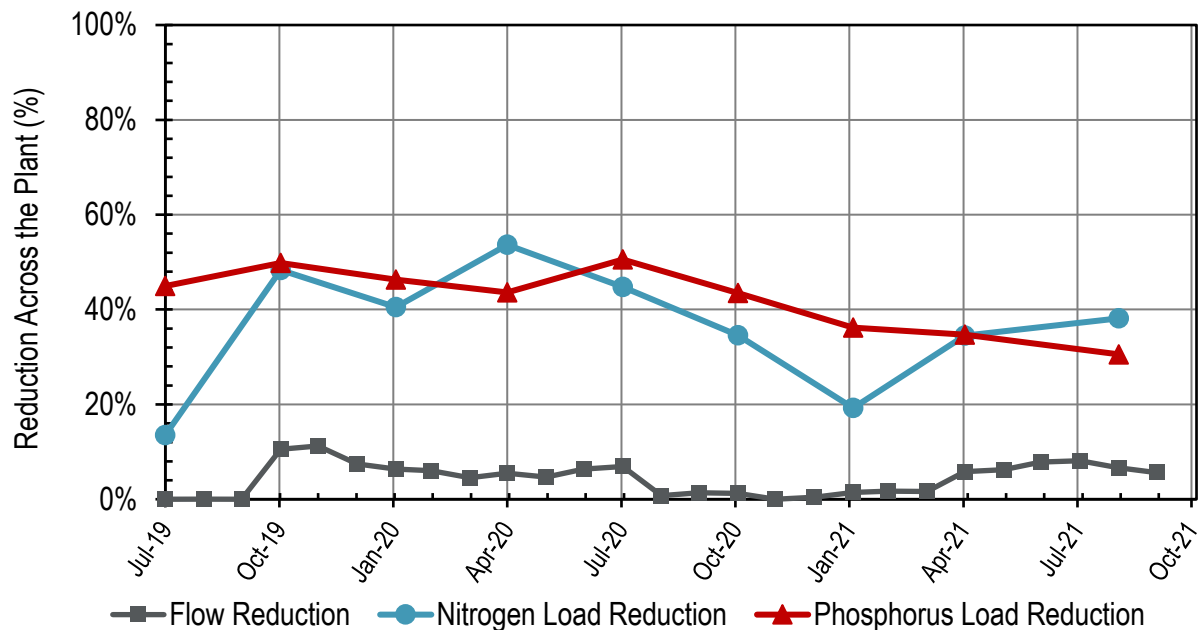
Figure 22-2. Influent: San Mateo Monthly Reductions Across the Plant
