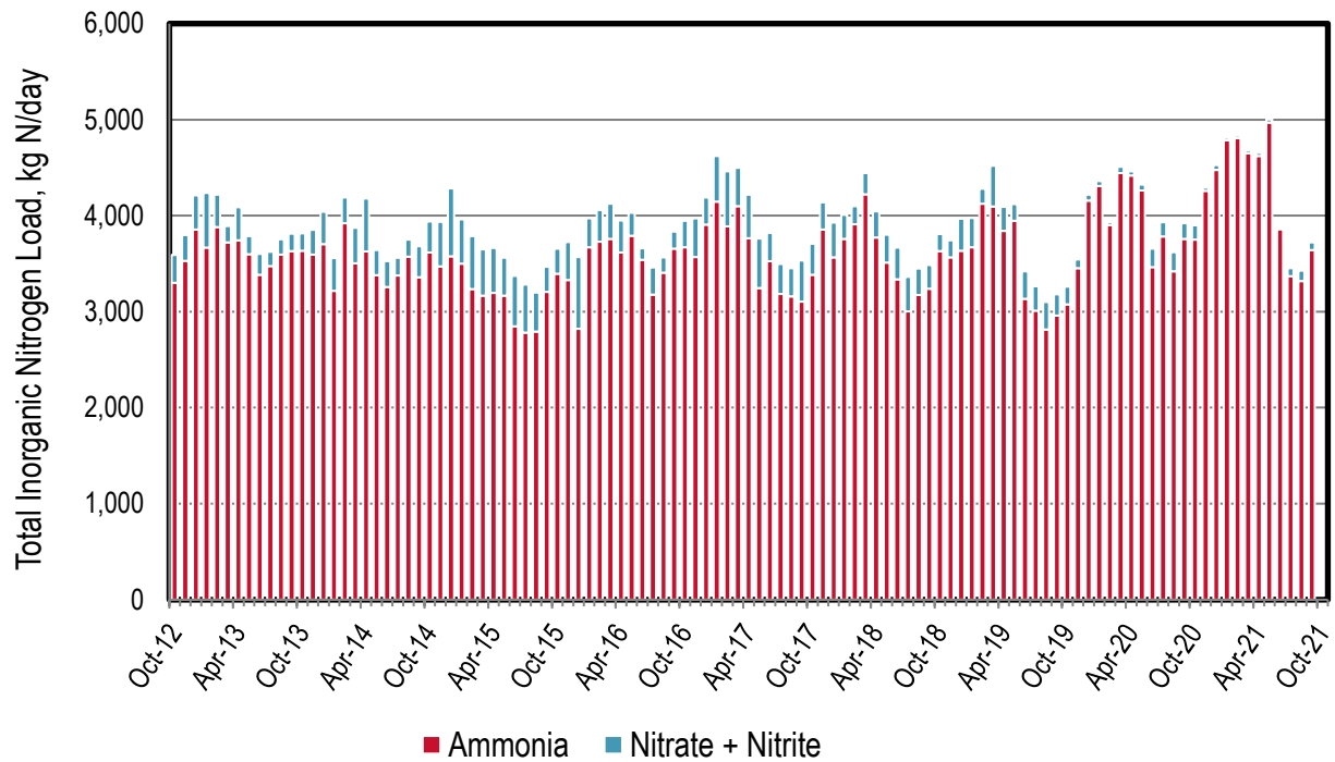
Figure 4-4. Discharge: Central San Monthly Nitrogen Loads
