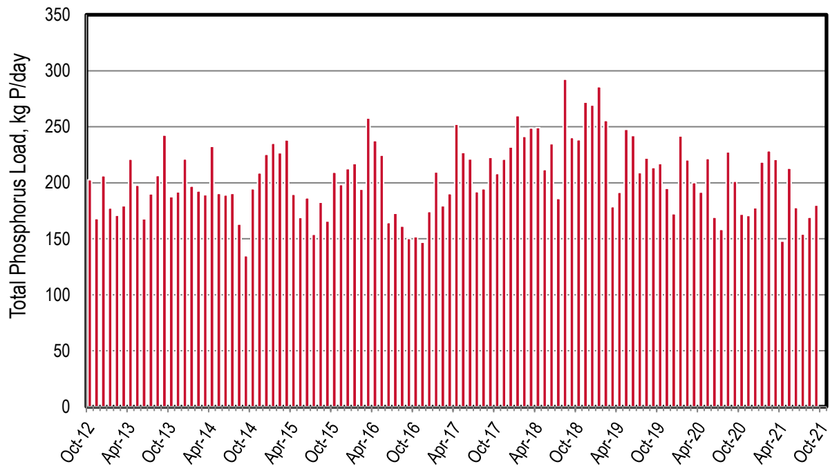
Figure 10-6. Discharge: FSSD Monthly Phosphorus Loads
