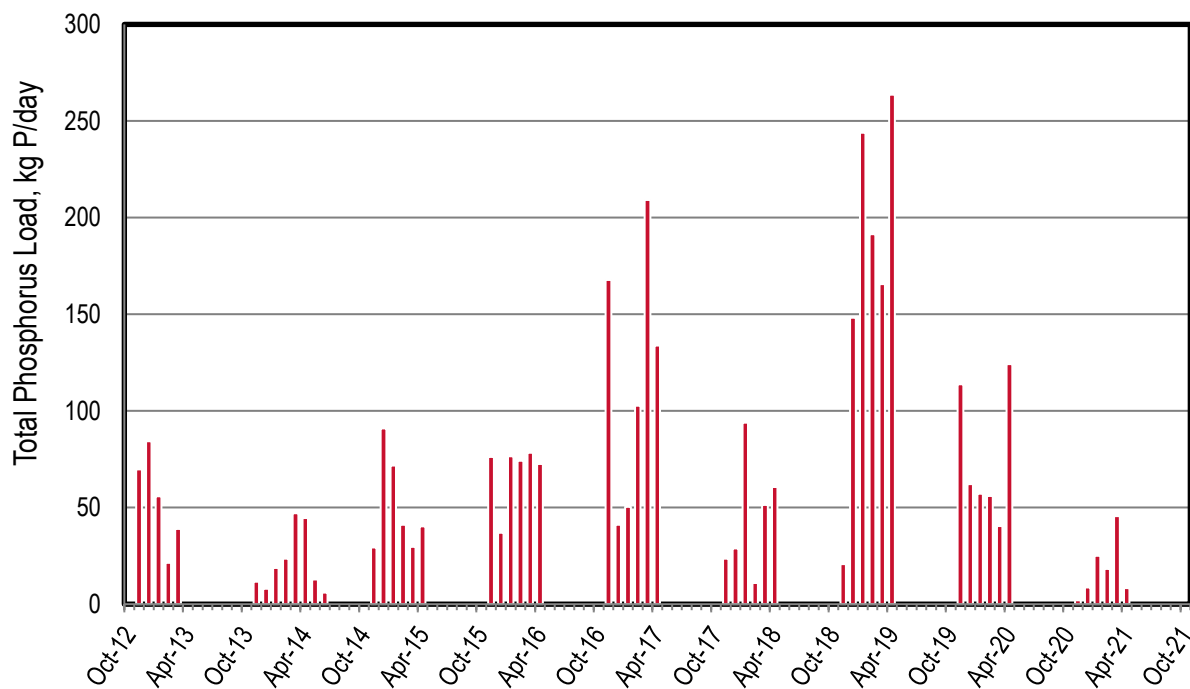
Figure 14-6. Discharge: Napa Sanitation District Monthly Phosphorus Loads
