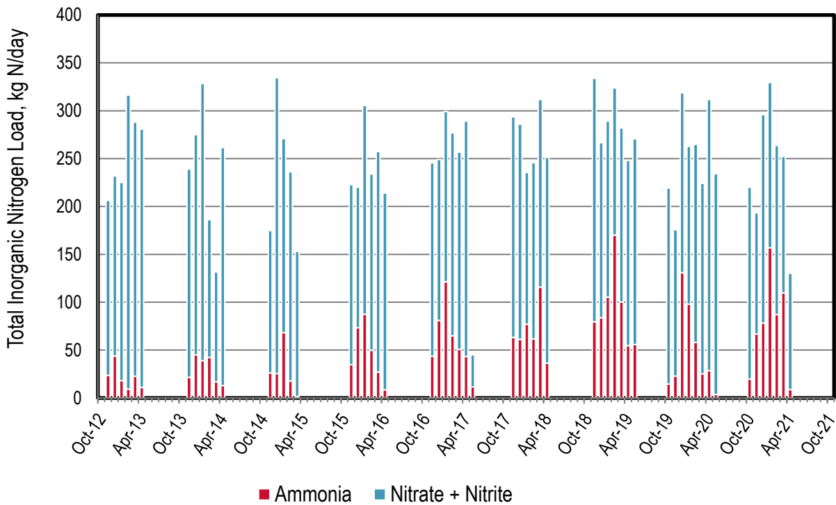
Figure 11-2. Discharge: Las Gallinas Monthly Nitrogen Loads
