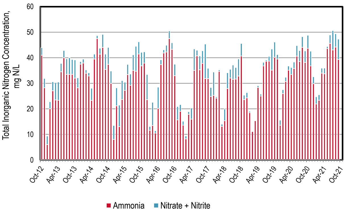
Figure 5-3. Discharge: CMSA Monthly Nitrogen Concentrations
