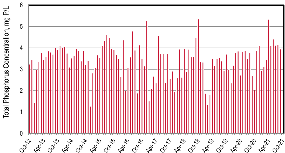
Figure 33-7. Discharge: Vallejo Monthly Phosphorus Concentrations
