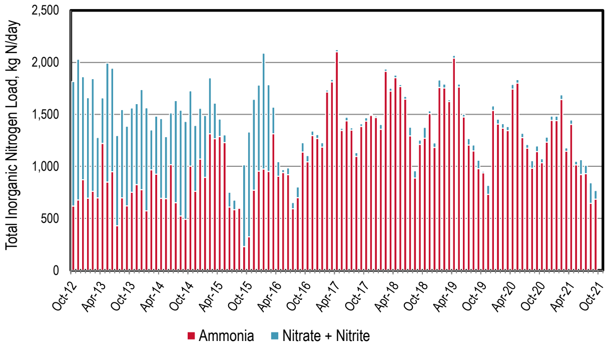
Figure 7-4. Discharge: Delta Diablo Monthly Nitrogen Loads
