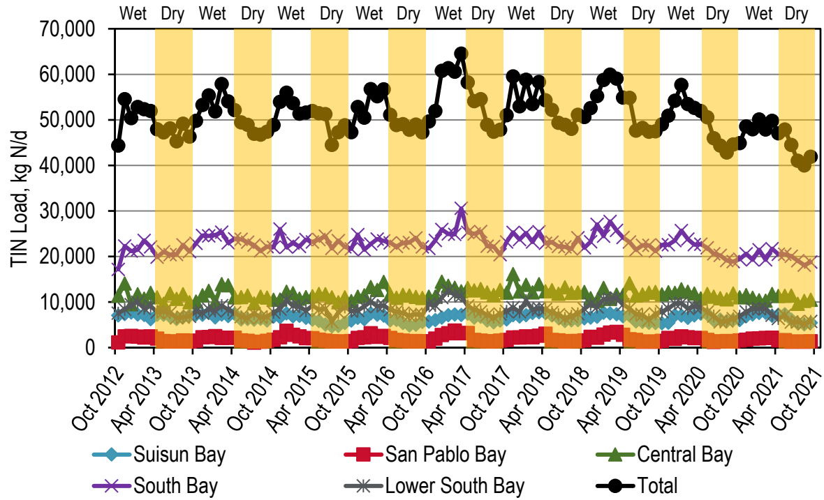
Figure 5-4. Discharge: Average Monthly Discharge TIN Loads
