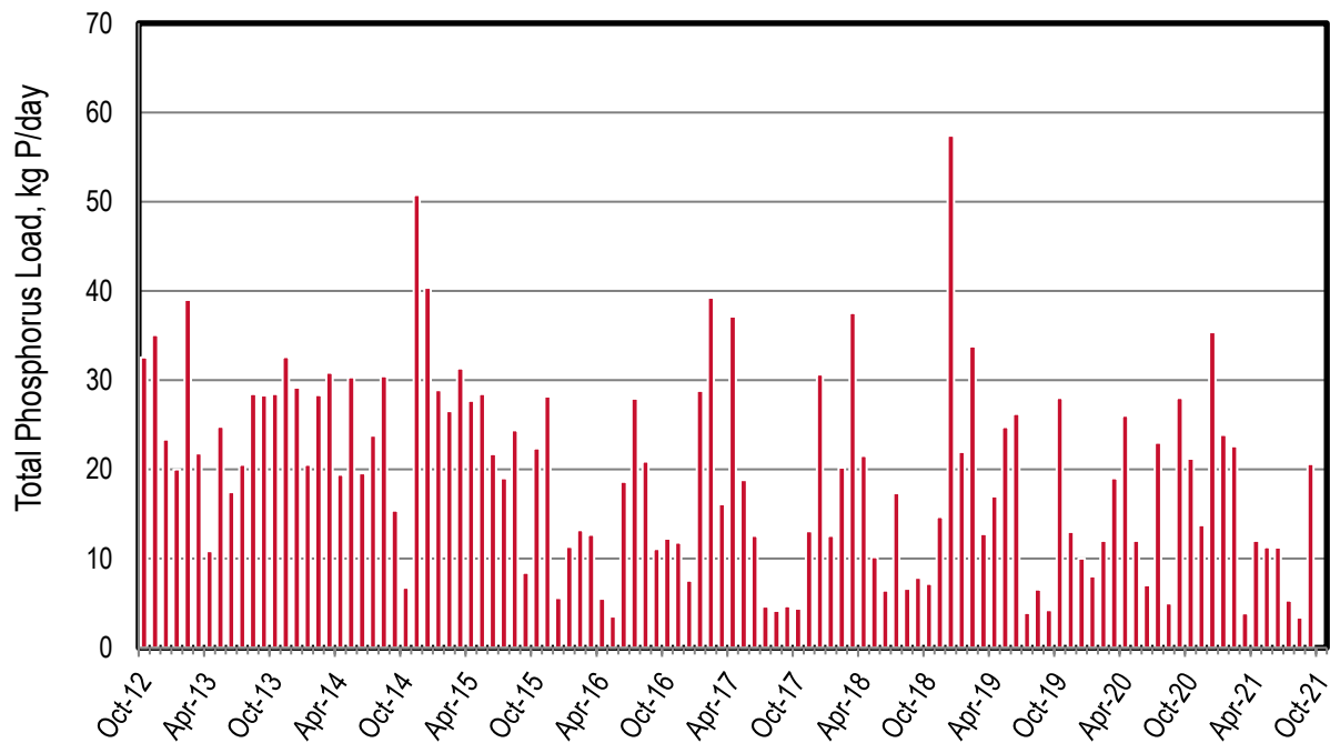
Figure 2-4. Discharge: Benicia Monthly Phosphorus Loads
