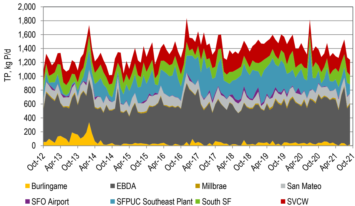
Figure 5-21. TP Load Contribution by Discharger to South Bay
