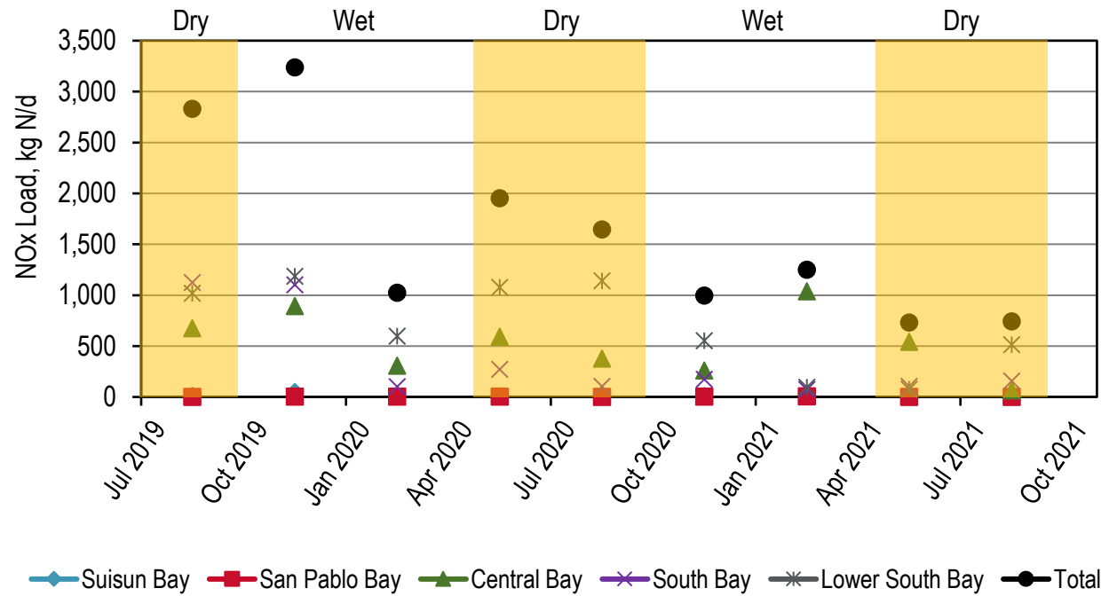
Figure 4-3. Influent: Historical Average Monthly NOx Loads
