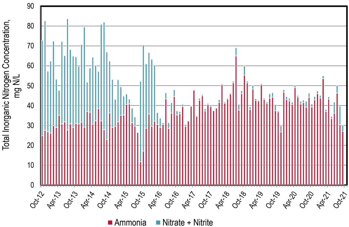
Figure 7-5. Discharge: Delta Diablo Monthly Nitrogen Concentrations
