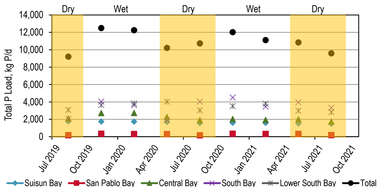
Figure 4-7. Influent: Historical Average Monthly Total P Loads for Evaluation Period
