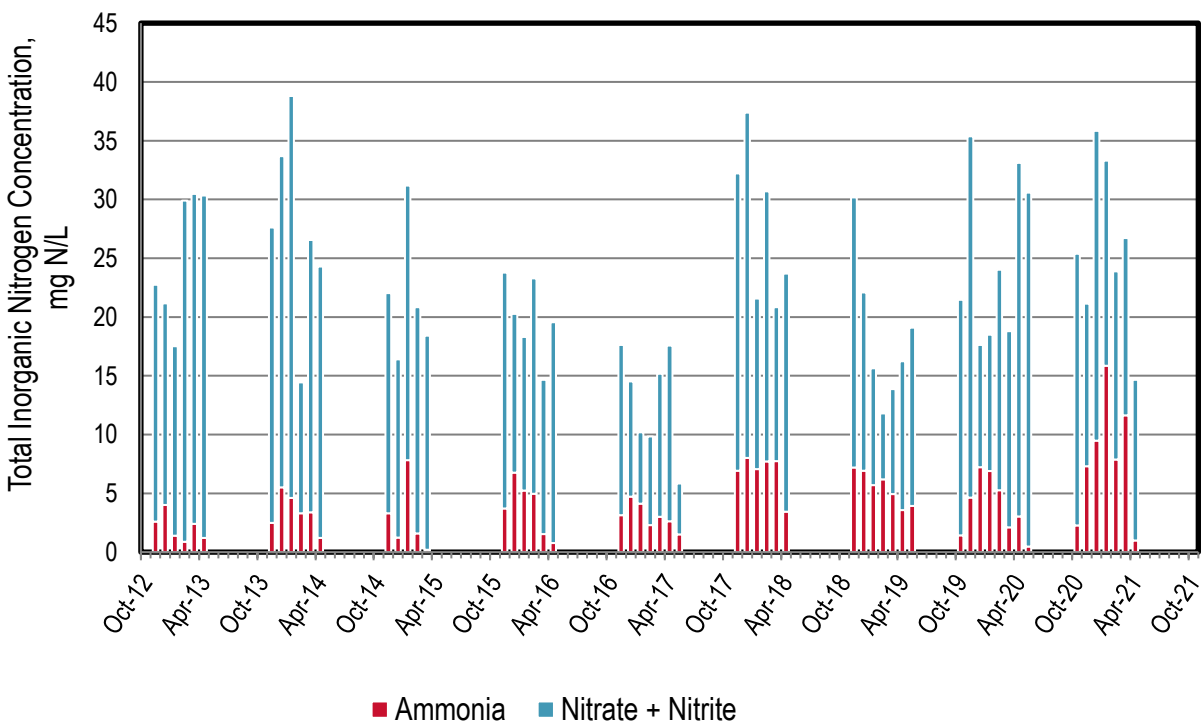
Figure 11-3. Discharge: Las Gallinas Monthly Nitrogen Concentrations
