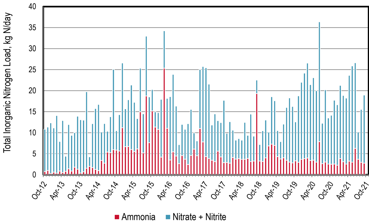
Figure 32-2. Treasure Island Monthly Nitrogen Loads
