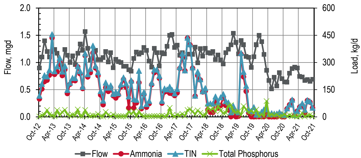
Figure 24-1. Discharge: SFO Airport Monthly Flows and Loads
