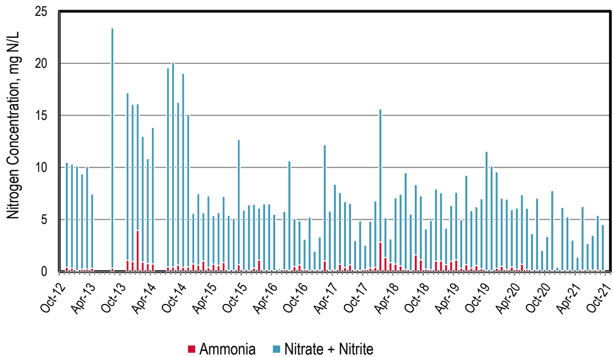
Figure 1-3. Discharge: American Canyon Monthly Nitrogen Concentrations
