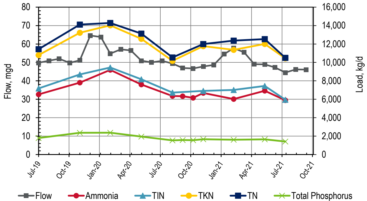
Figure 9-1. Influent: EBMUD Monthly Flows and Loads
