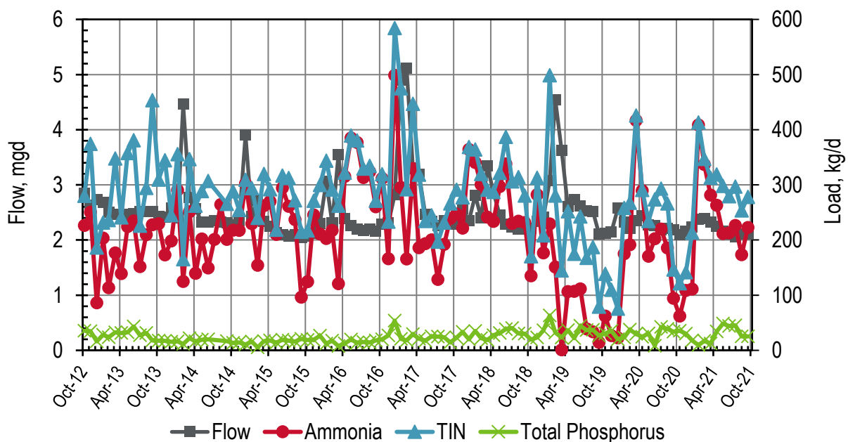
Figure 19-1. Discharge: Pinole Monthly Flows and Loads
