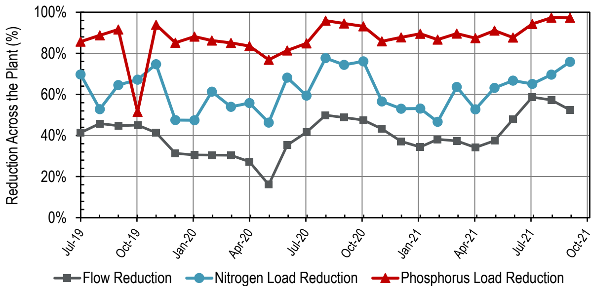
Figure 7-2. Influent: Delta Diablo Monthly Reductions Across the Plant
