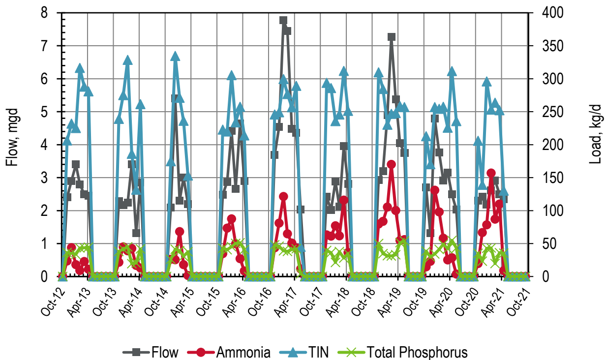
Figure 11-1. Discharge: Las Gallinas Monthly Flows and Loads
