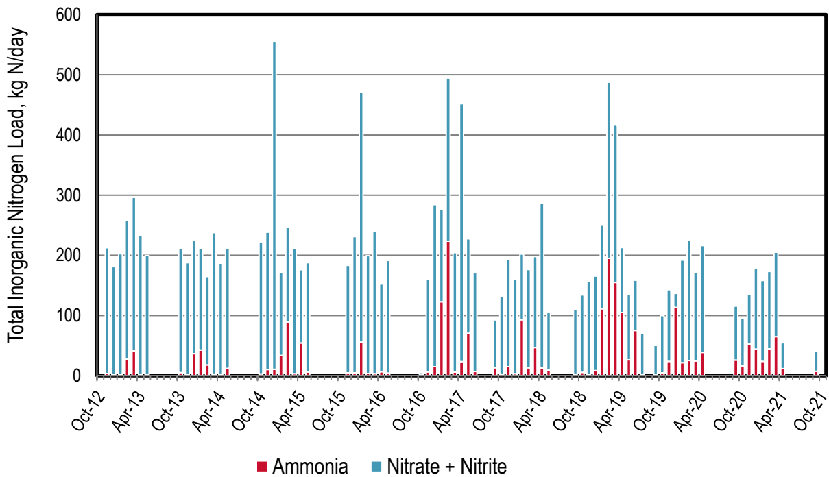
Figure 15-2. Discharge: Novato Monthly Nitrogen Loads
