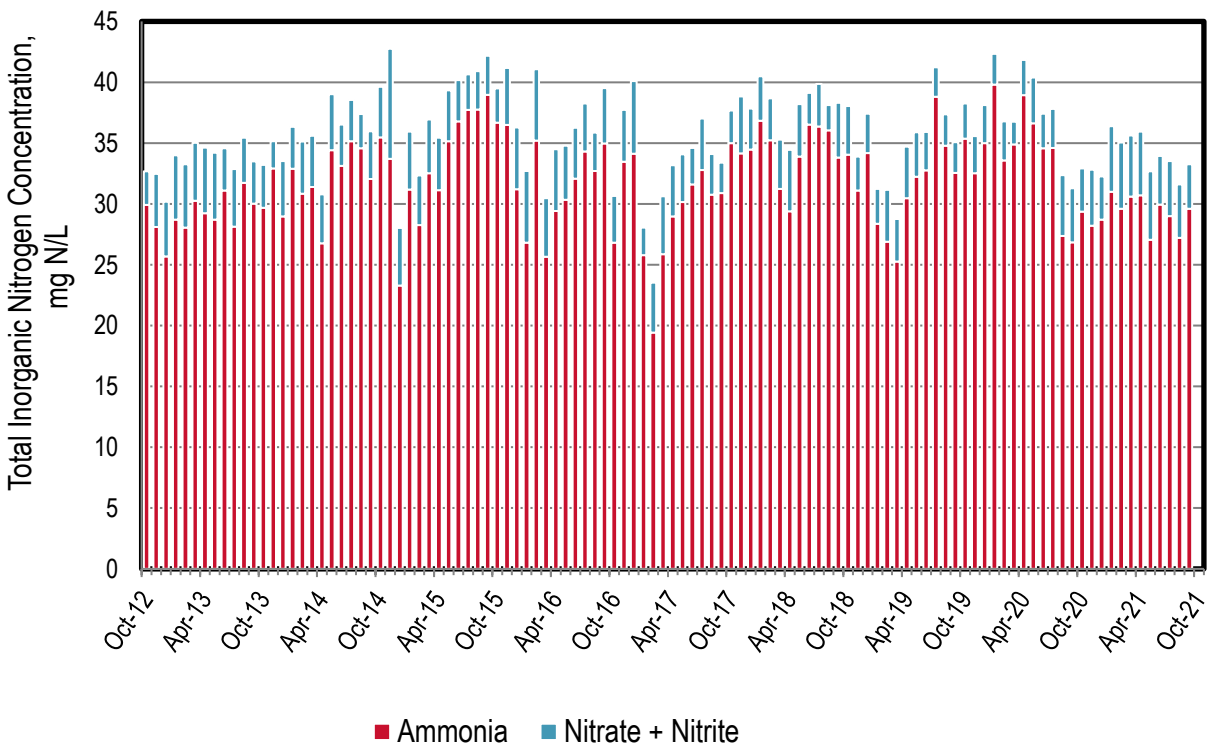
Figure 8-5. Discharge: EBDA Monthly Nitrogen Concentrations
