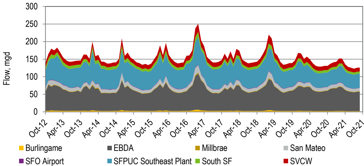
Figure 5-18. Flow Contribution by Discharger to South Bay
