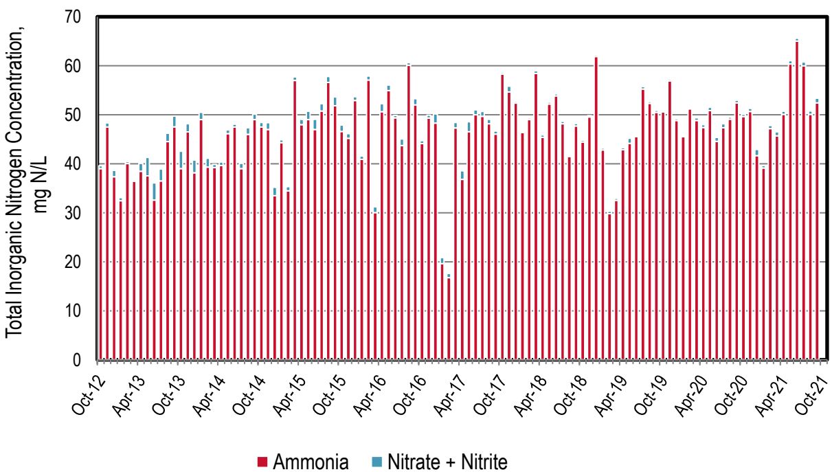
Figure 30-5. Discharge: SVCW Monthly Nitrogen Concentrations
