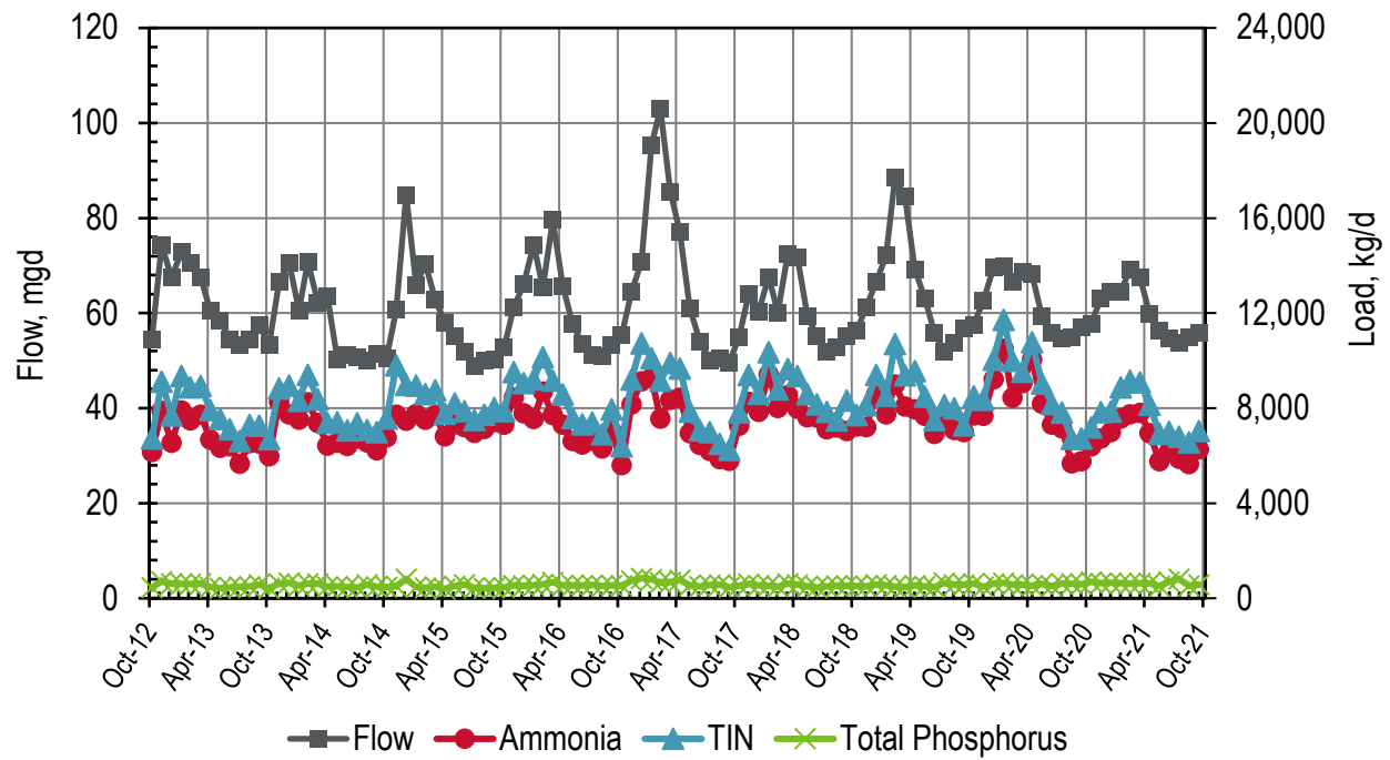
Figure 8-3. Discharge: EBDA Monthly Flows and Loads
