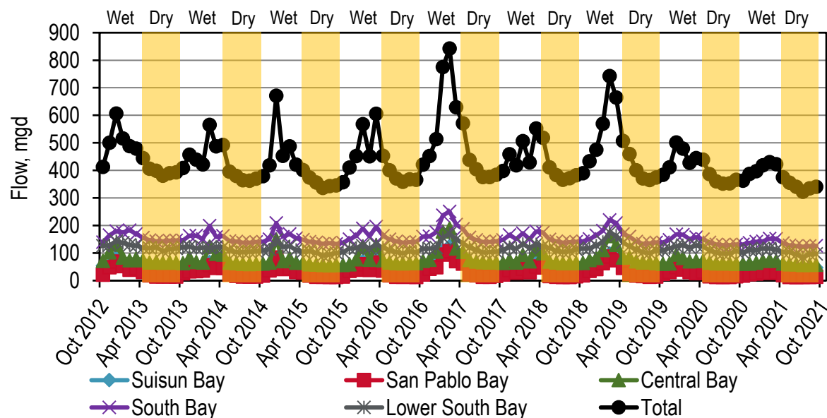
Figure 5-1. Discharge: Average Monthly Discharge Flows
