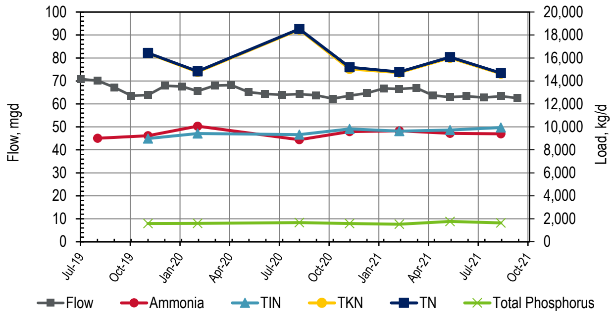
Figure 8-1. Influent: EBDA Monthly Flows and Loads
