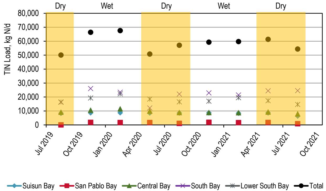
Figure 4-4. Influent: Historical Average Monthly TIN Loads
