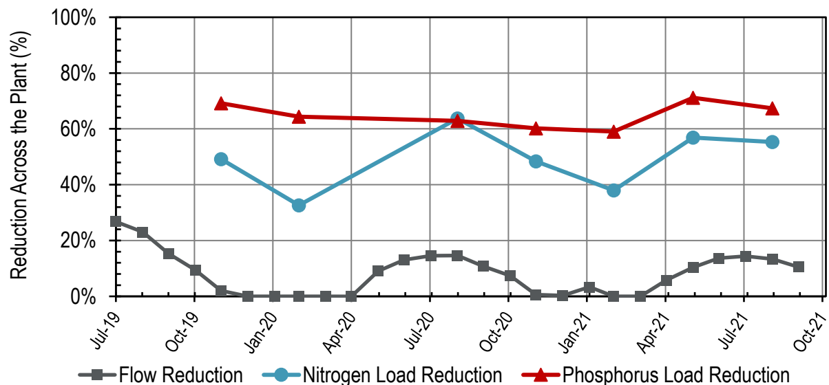
Figure 8-2. Influent: EBDA Monthly Reductions Across the Plant
