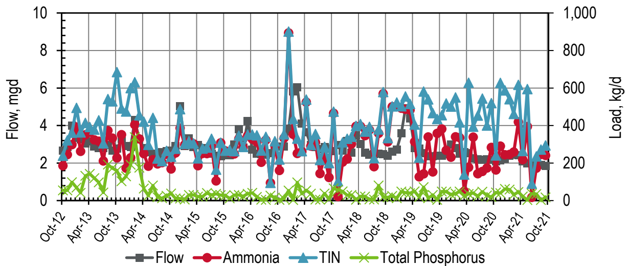
Figure 3-1. Discharge: Burlingame Monthly Flows and Loads
