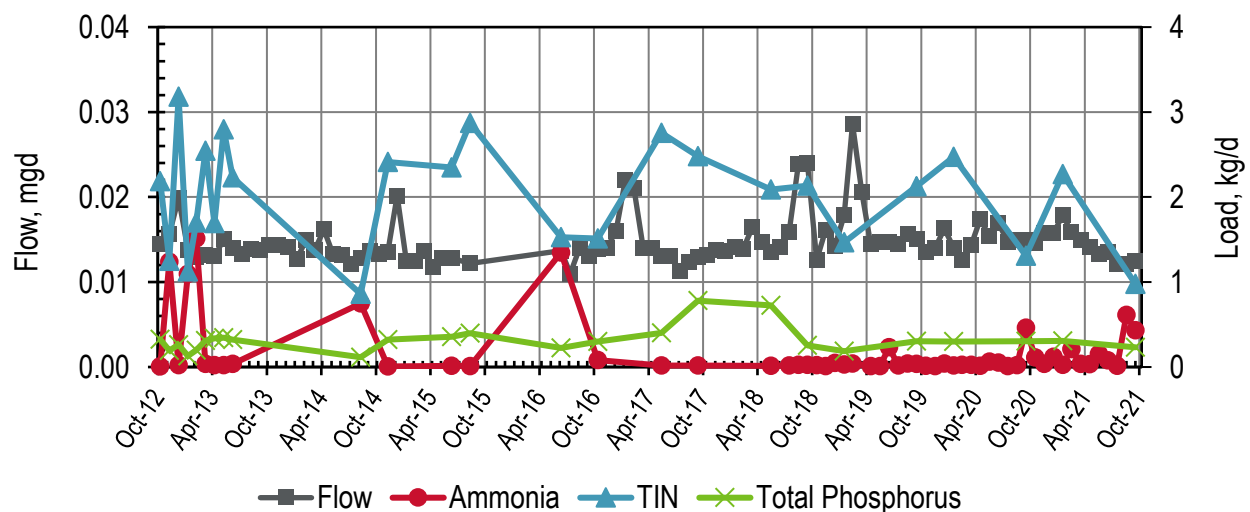
Figure 17-1. Discharge: Paradise Cove Monthly Flows and Loads
