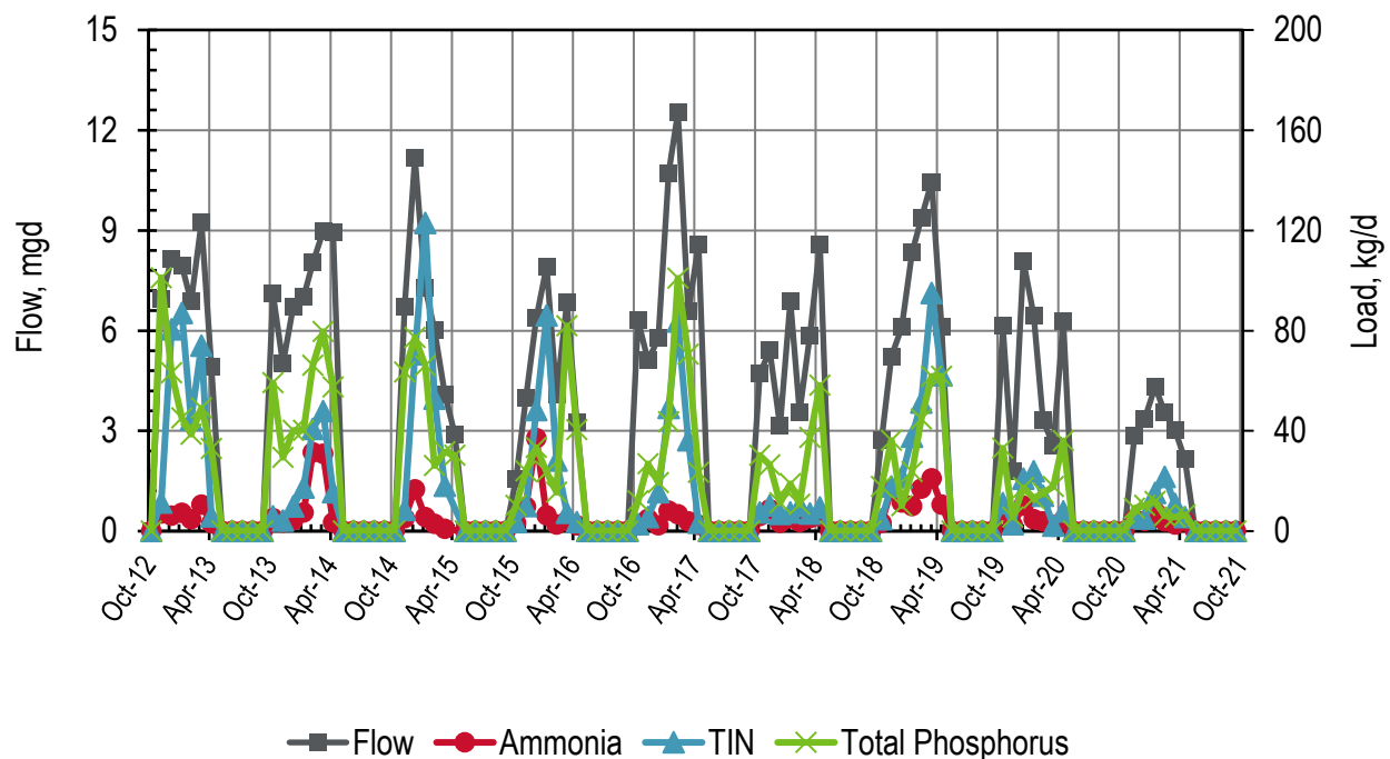
Figure 18-1. Discharge: Petaluma Monthly Flows and Loads
