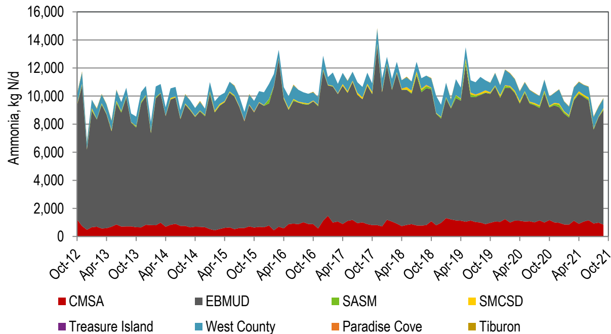
Figure 5-15. Ammonia Load Contribution by Discharger to Central Bay
