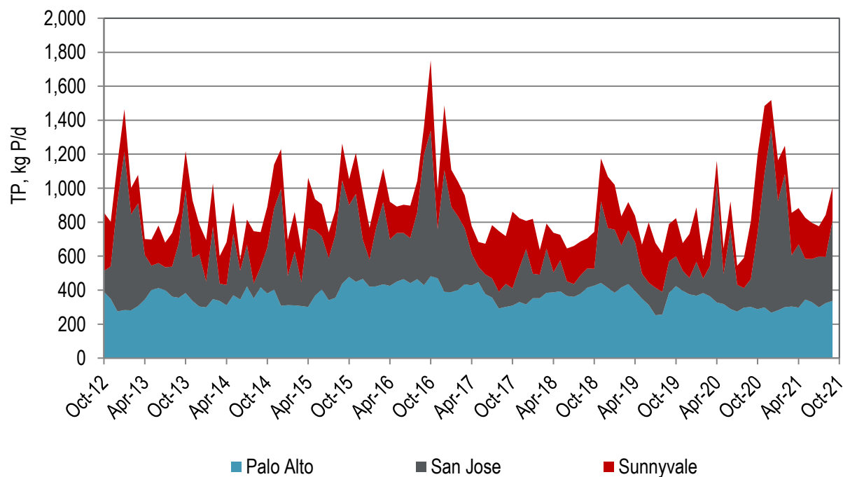
Figure 5-25. TP Load Contribution by Discharger to Lower South Bay
