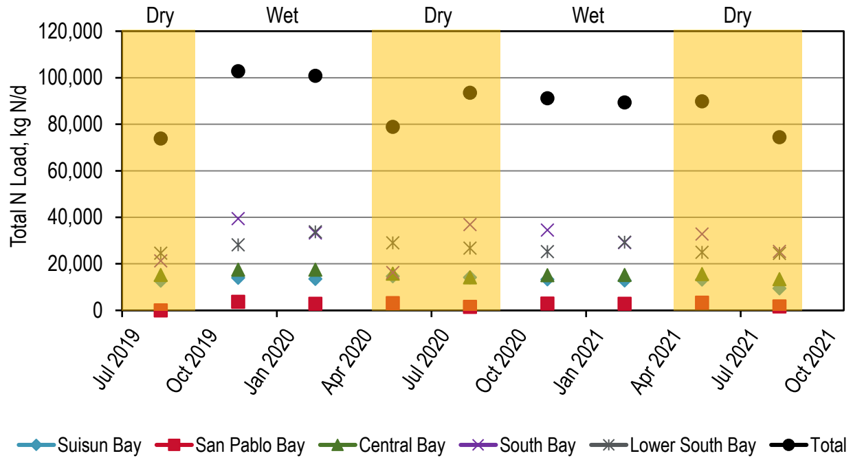
Figure 4-6. Influent: Historical Average Monthly Total N Loads
