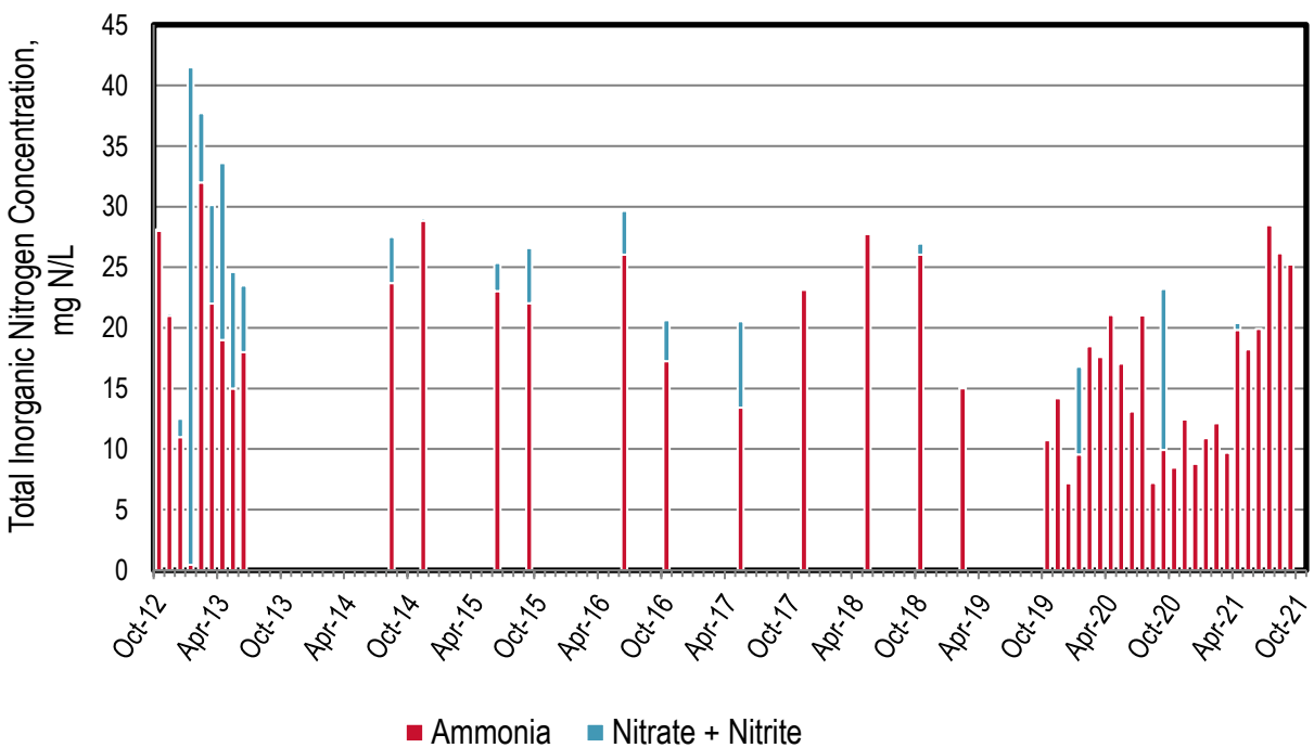
Figure 31-3. Discharge: Tiburon Monthly Nitrogen Concentrations
