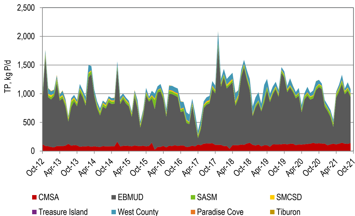
Figure 5-17. TP Load Contribution by Discharger to Central Bay
