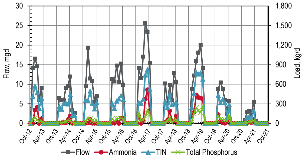
Figure 14-3. Discharge: Napa Sanitation District Monthly Flows and Loads
