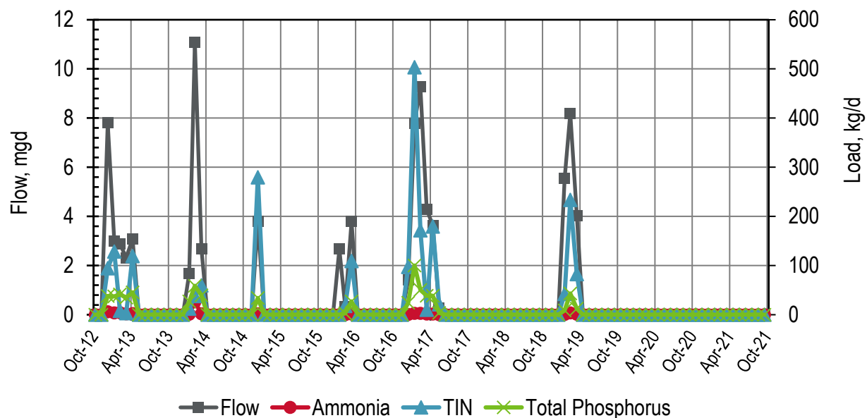
Figure 27-1. Discharge: Sonoma Valley Monthly Flows and Loads
