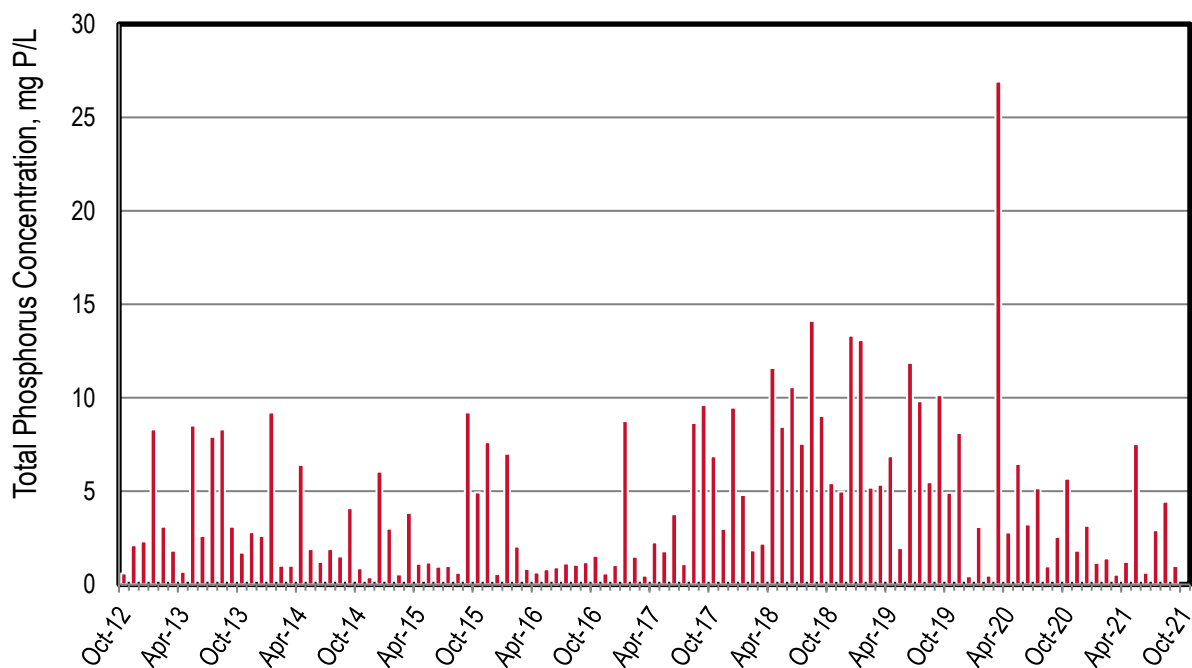
Figure 24-5. Discharge: SFO Airport Monthly Phosphorus Concentrations
