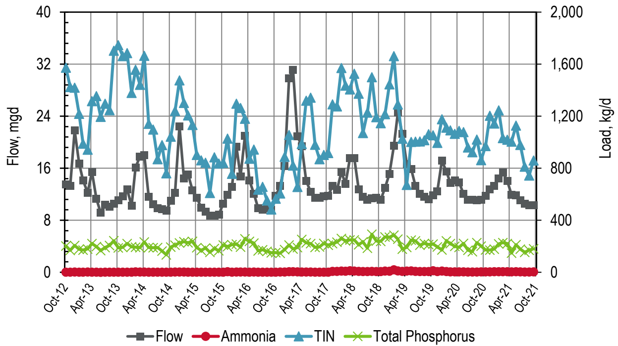
Figure 10-3. Discharge: FSSD Monthly Flows and Loads
