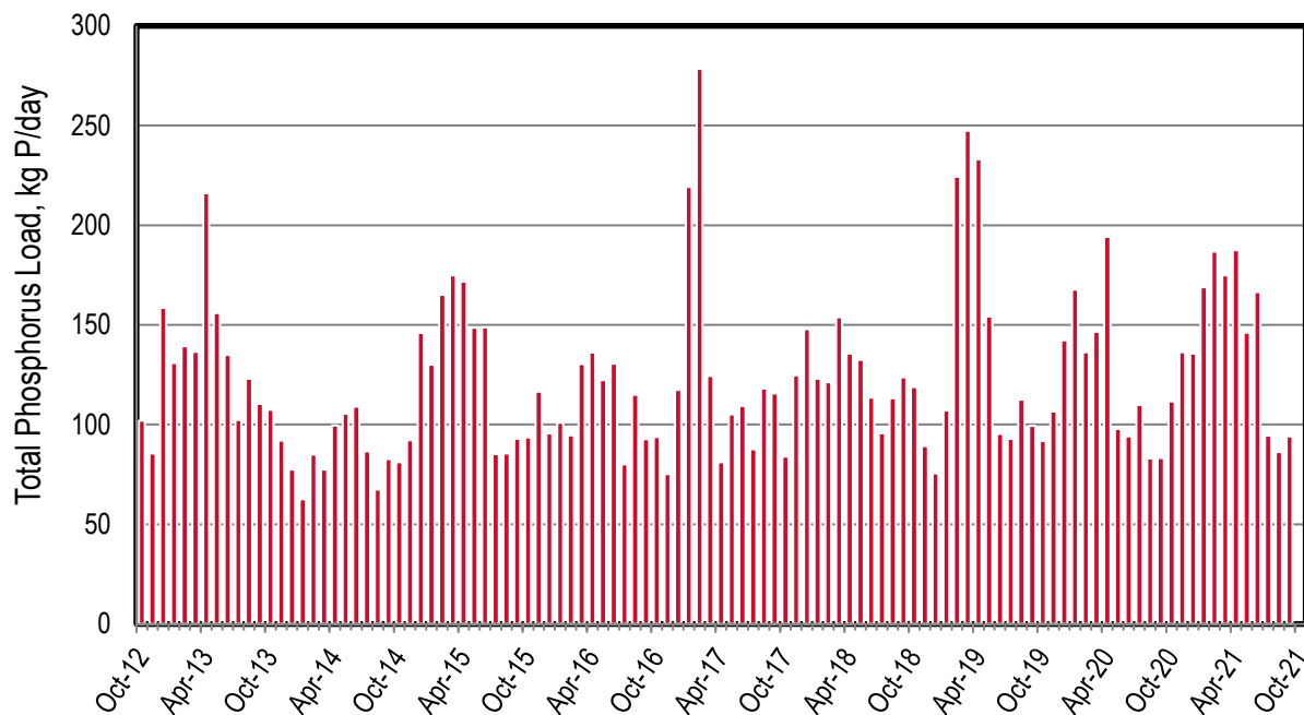
Figure 4-6. Discharge: Central San Monthly Phosphorus Loads
