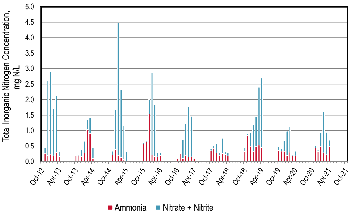
Figure 18-3. Discharge: Petaluma Monthly Nitrogen Concentrations
