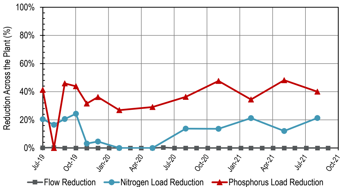
Figure 30-2. Influent: SVCW Monthly Reductions Across the Plant
