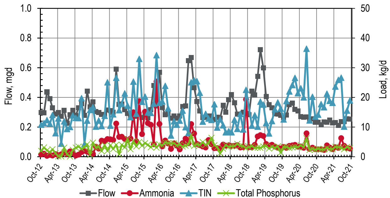
Figure 32-1. Treasure Island Monthly Flows and Loads
