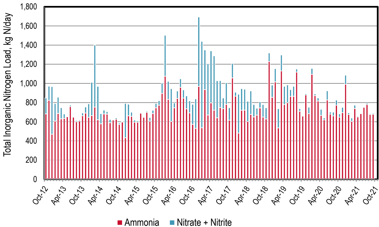
Figure 34-4. Discharge: West County Monthly Nitrogen Loads
