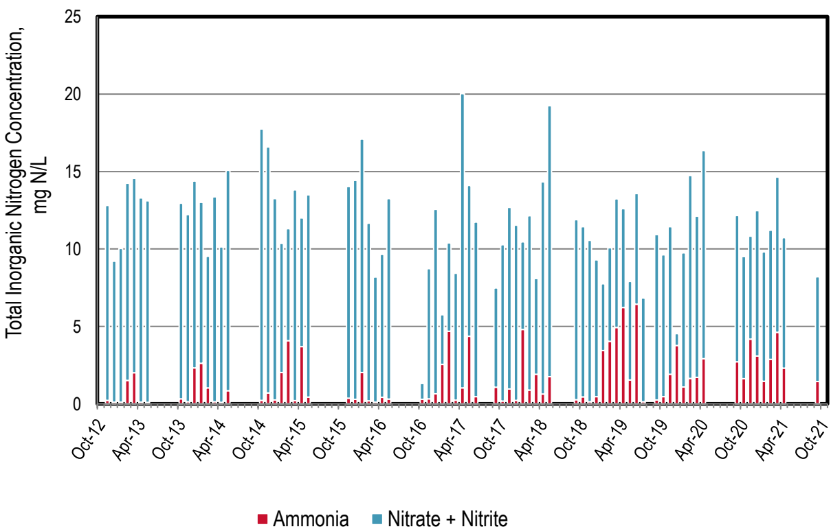
Figure 15-3. Discharge: Novato Monthly Nitrogen Concentrations
