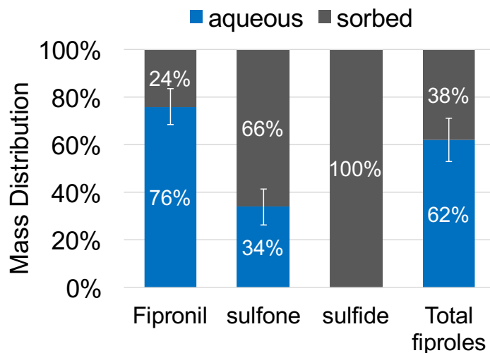
Figure S1. Relative distribution of the mass of imidacloprid, fipronil and major degradates between the dissolved and sorbed state (suspended solids) of wastewater influent samples ( n=8 ). Error bars represent standard deviation among 8 samples.
